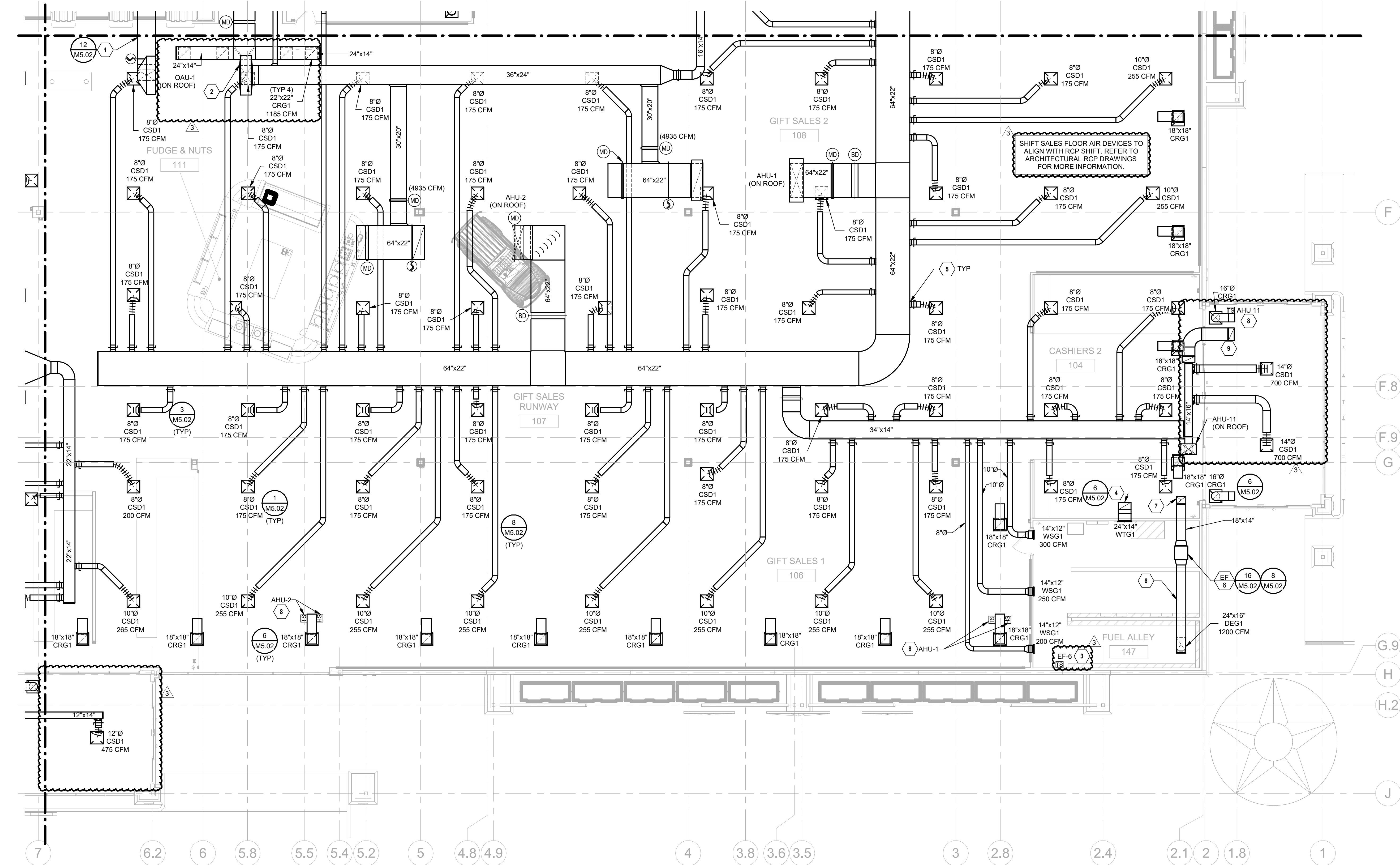
MECHANICAL FLOOR PLAN - AREA B 1/8" = 1'-0"
