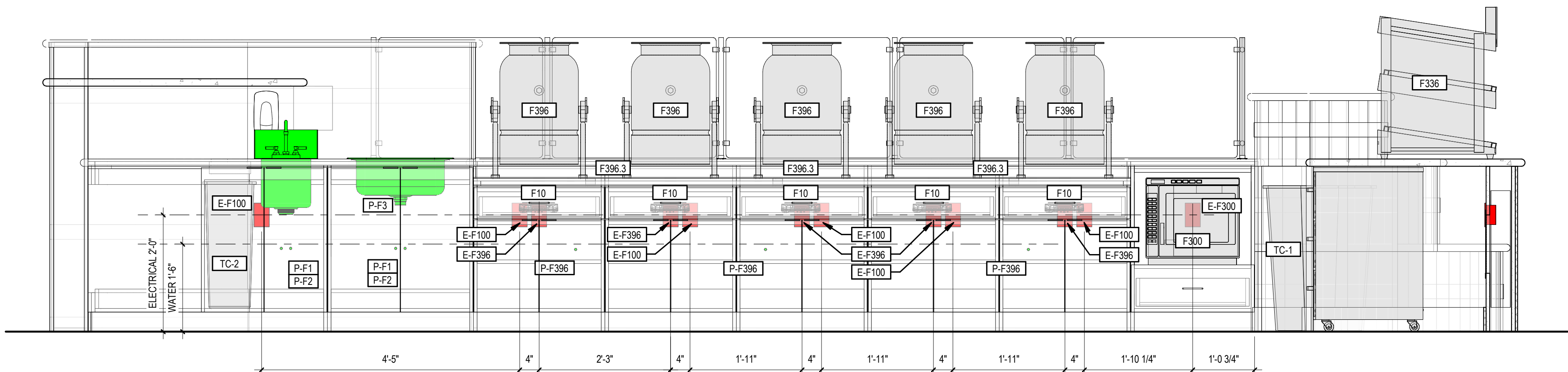
1 FUDGE & NUT EQUIPMENT ELEVATION
