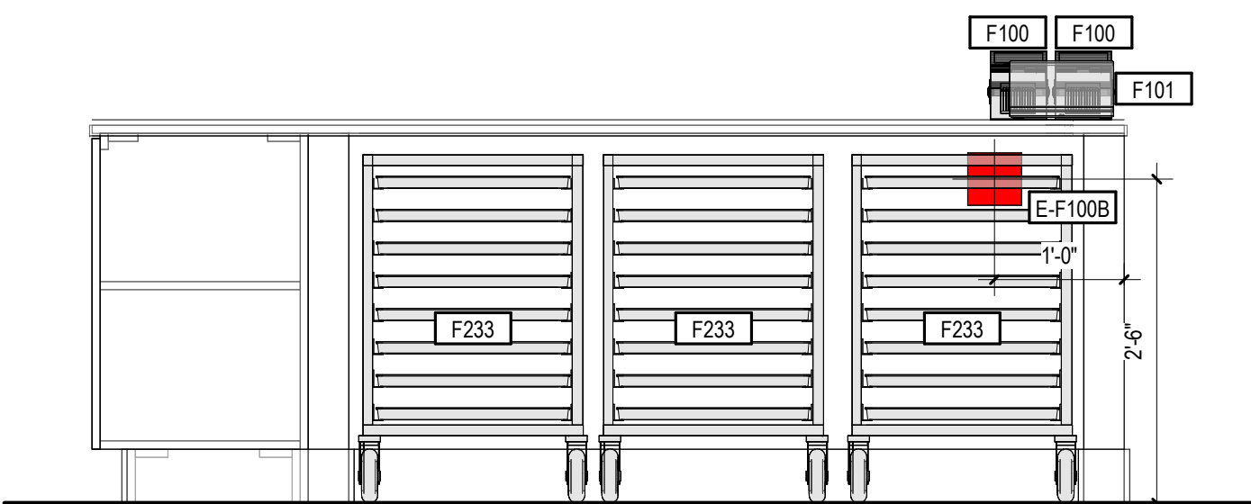
4 FUDGE & NUT EQUIPMENT ELEVATION
