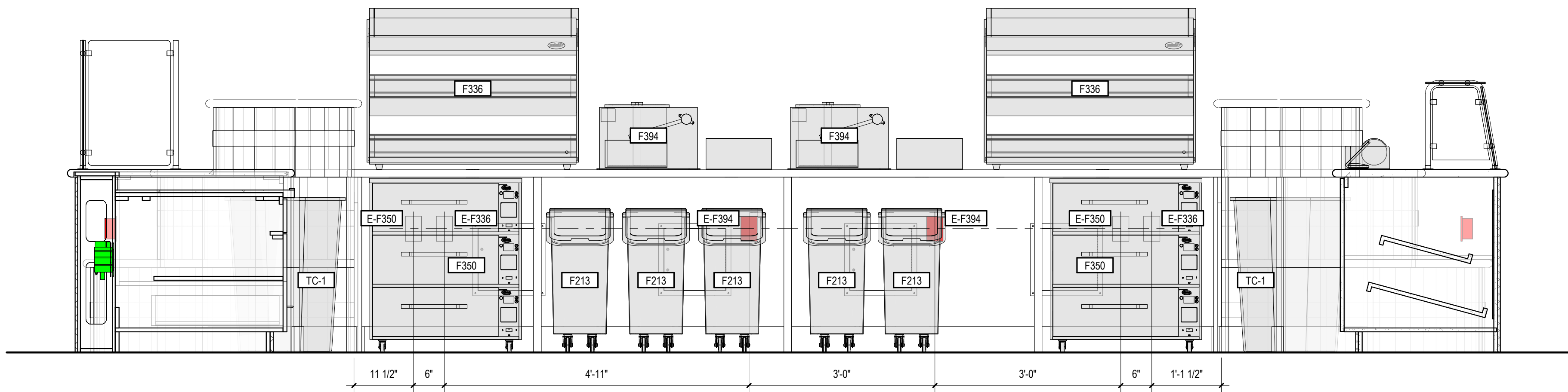
3 FUDGE & NUT EQUIPMENT ELEVATION
