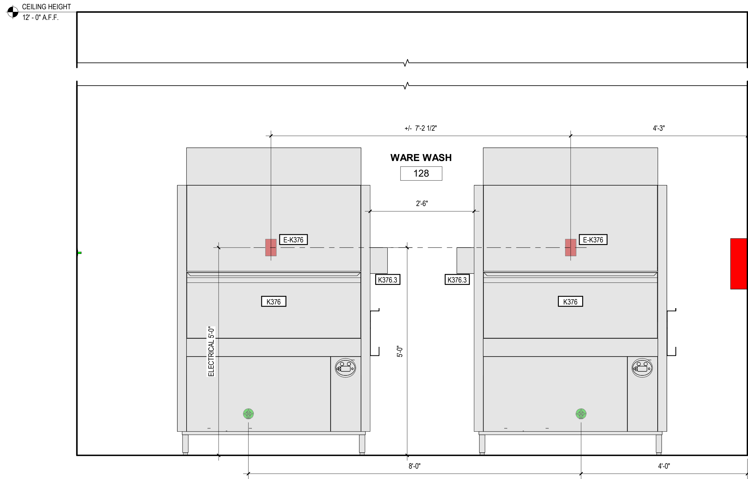
2 MAIN KITCHEN EQUIPMENT ELEVATION 3/4" = 1'-0"
