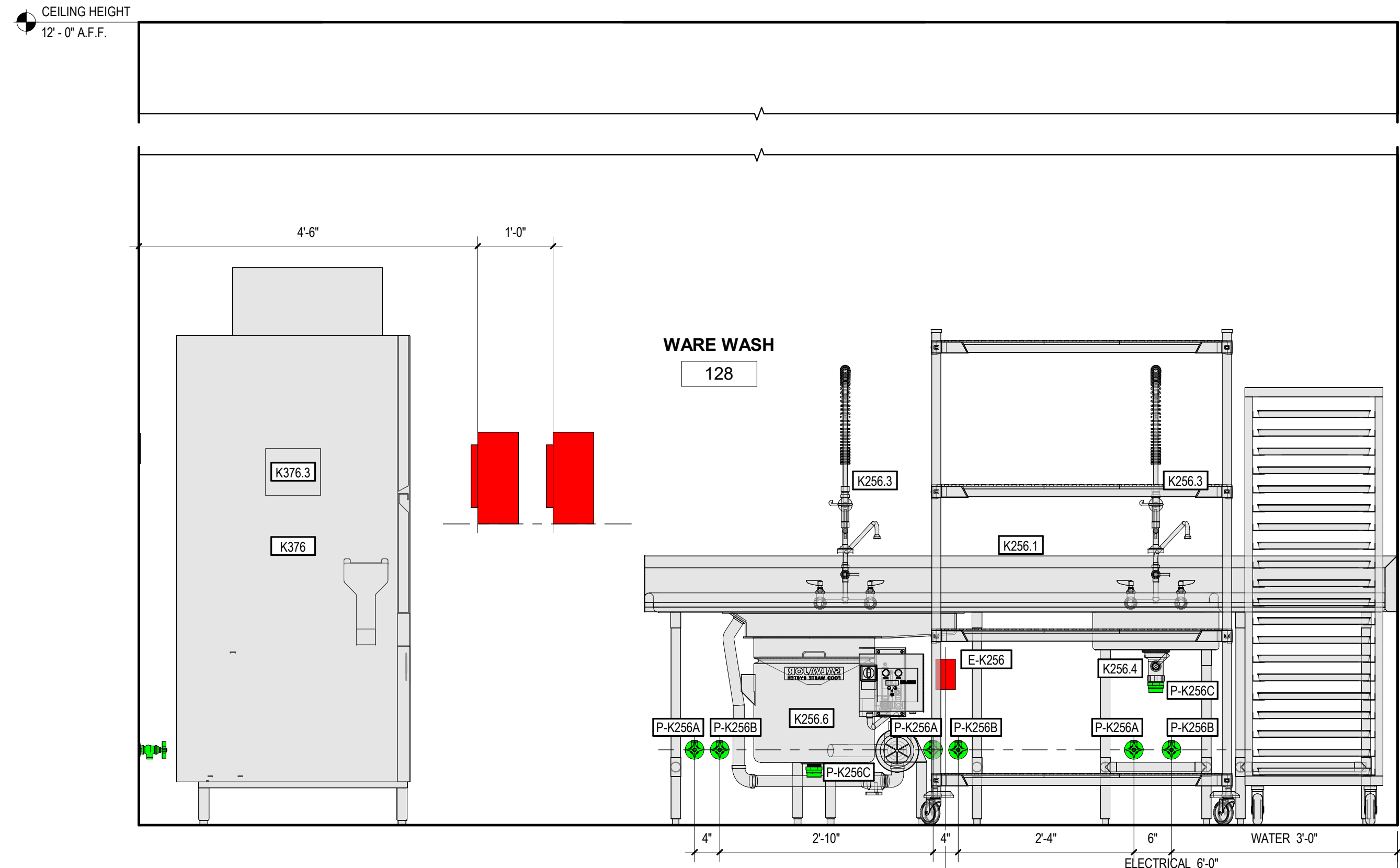
1 MAIN KITCHEN EQUIPMENT ELEVATION 3/4" = 1'-0"
