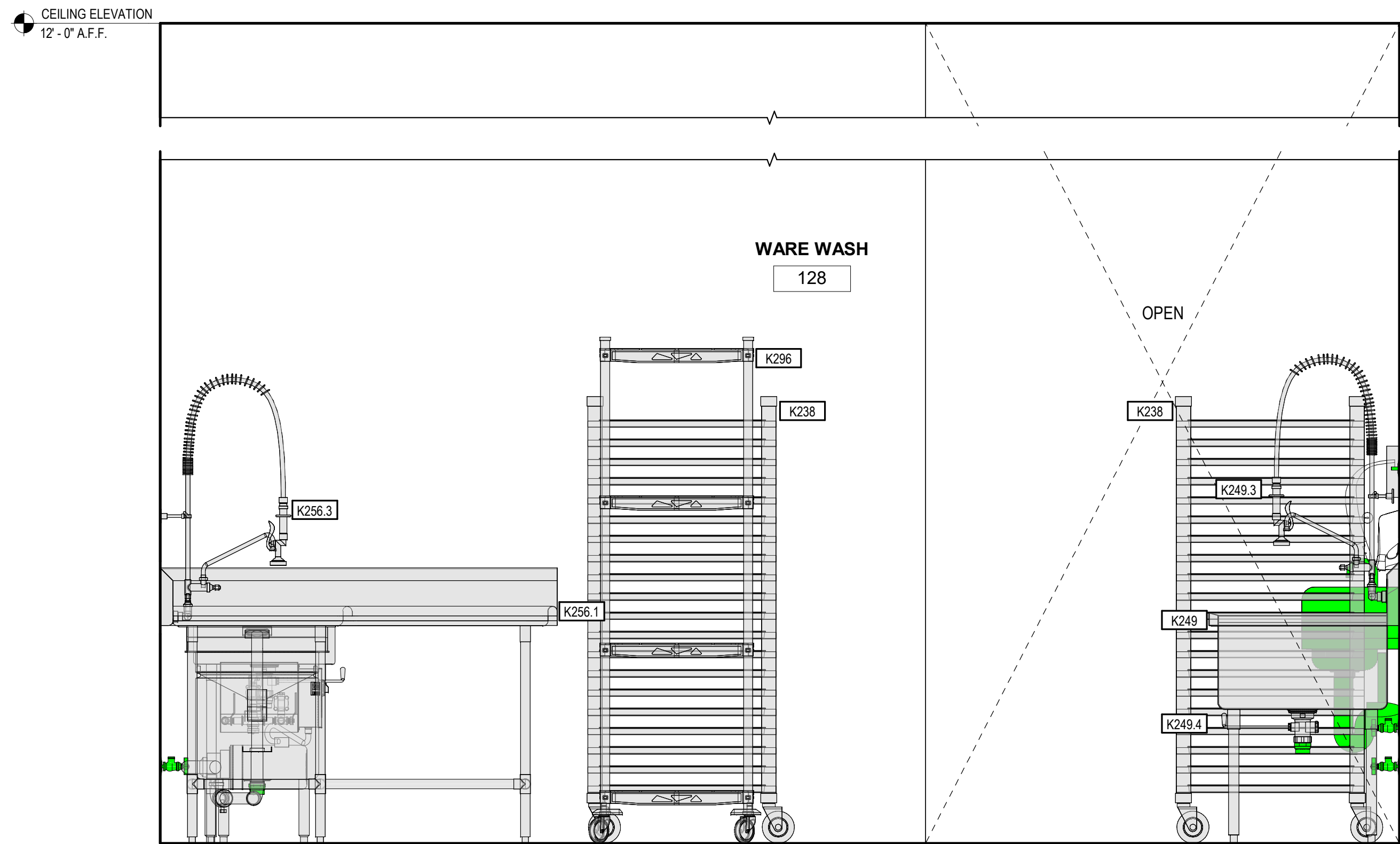
6 MAIN KITCHEN EQUIPMENT ELEVATION 3/4" = 1'-0"
