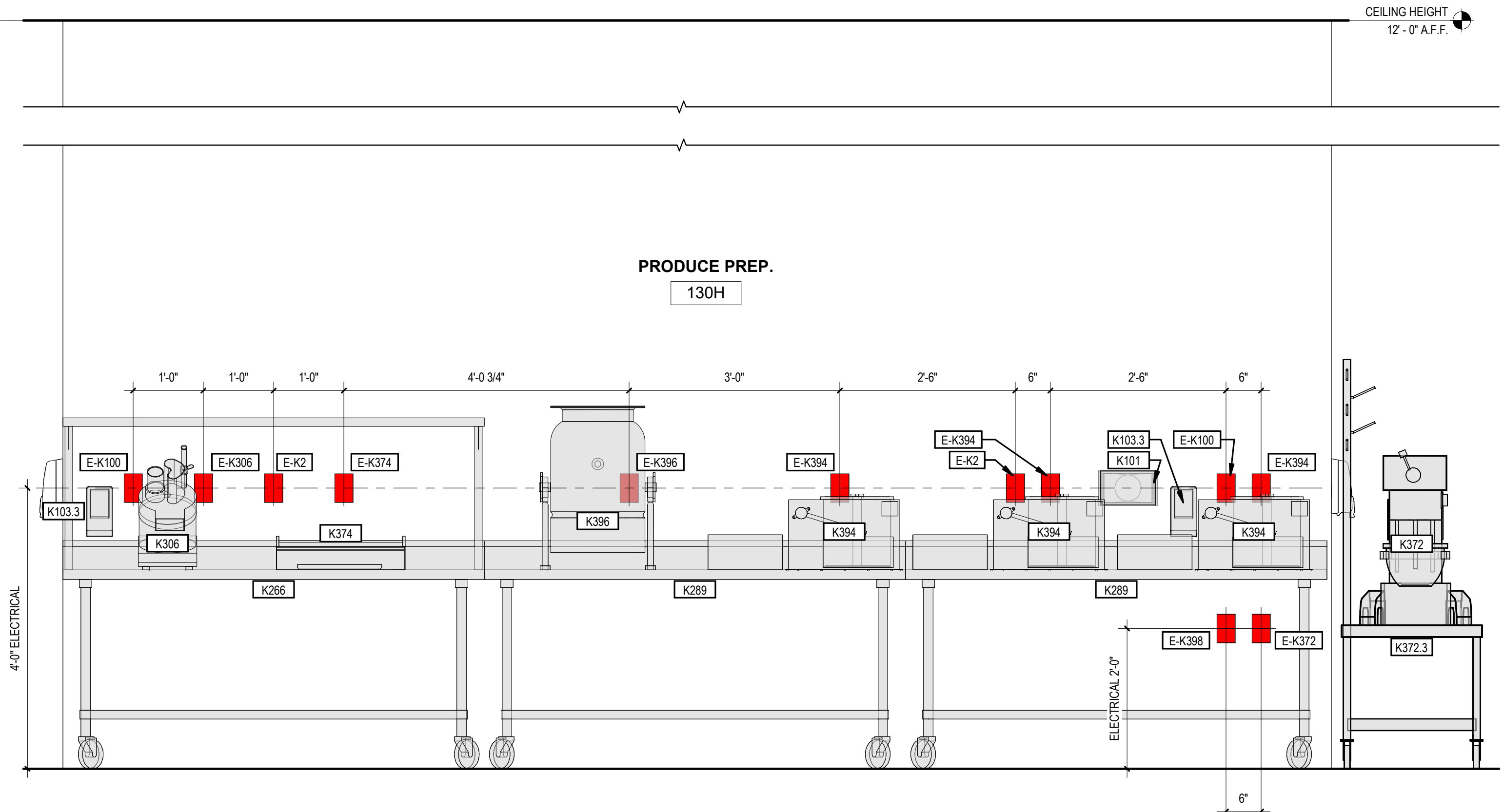
5 MAIN KITCHEN EQUIPMENT ELEVATION 3/4" = 1'-0"
