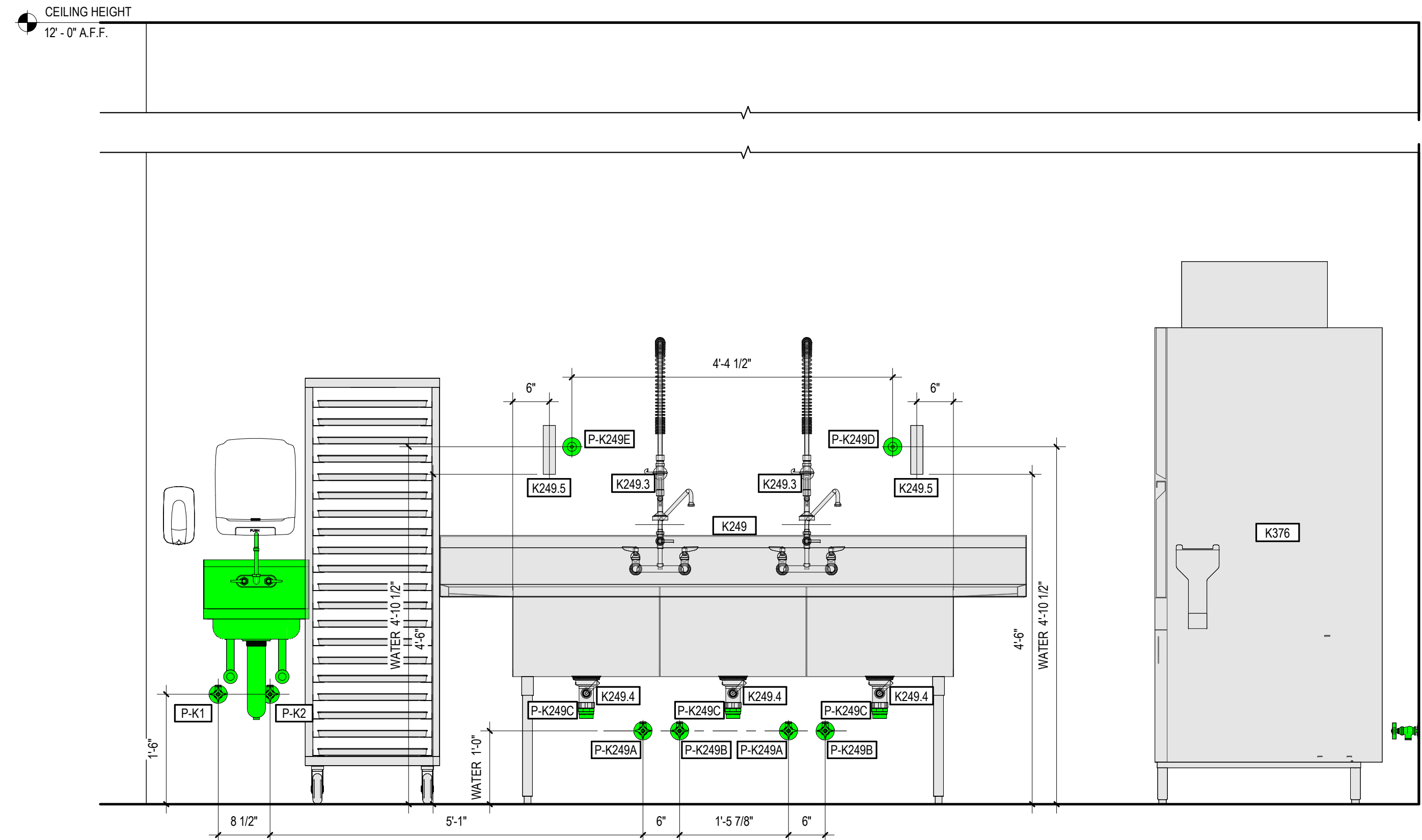
3 MAIN KITCHEN EQUIPMENT ELEVATION 3/4" = 1'-0"
