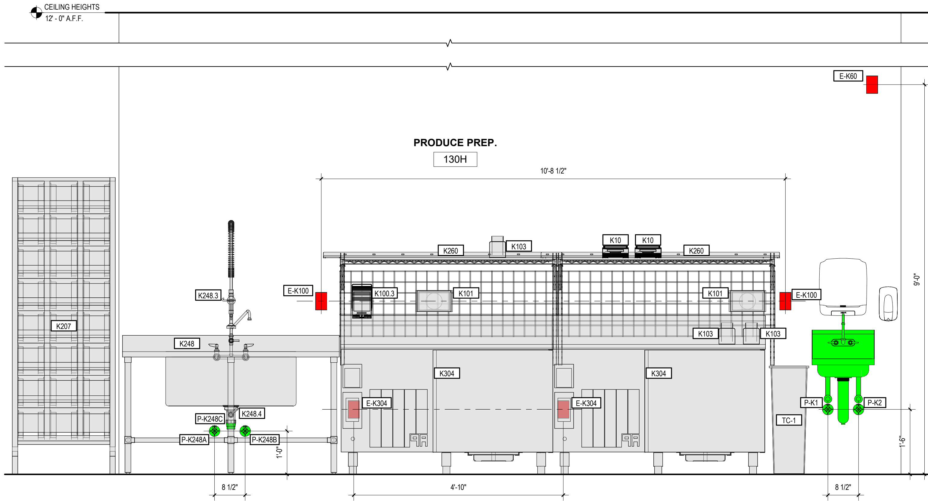
6 MAIN KITCHEN EQUIPMENT ELEVATION 3/4" = 1'-0"
