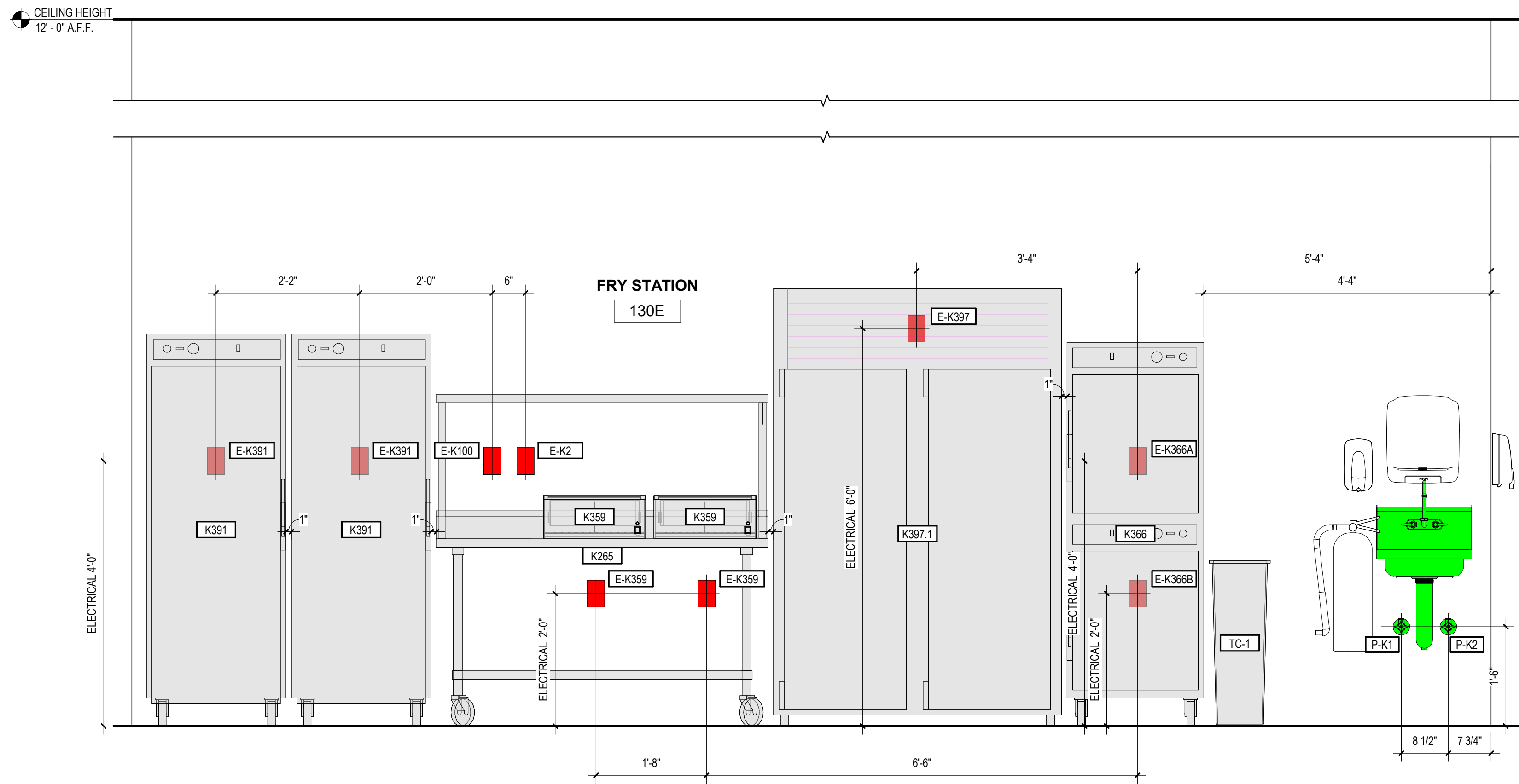
5 MAIN KITCHEN EQUIPMENT ELEVATION 3/4" = 1'-0"
