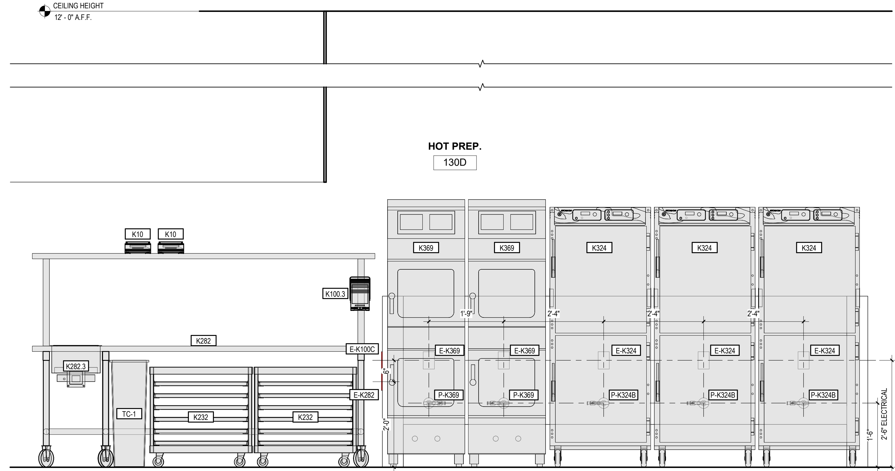
4 MAIN KITCHEN EQUIPMENT ELEVATION 3/4" = 1'-0"
