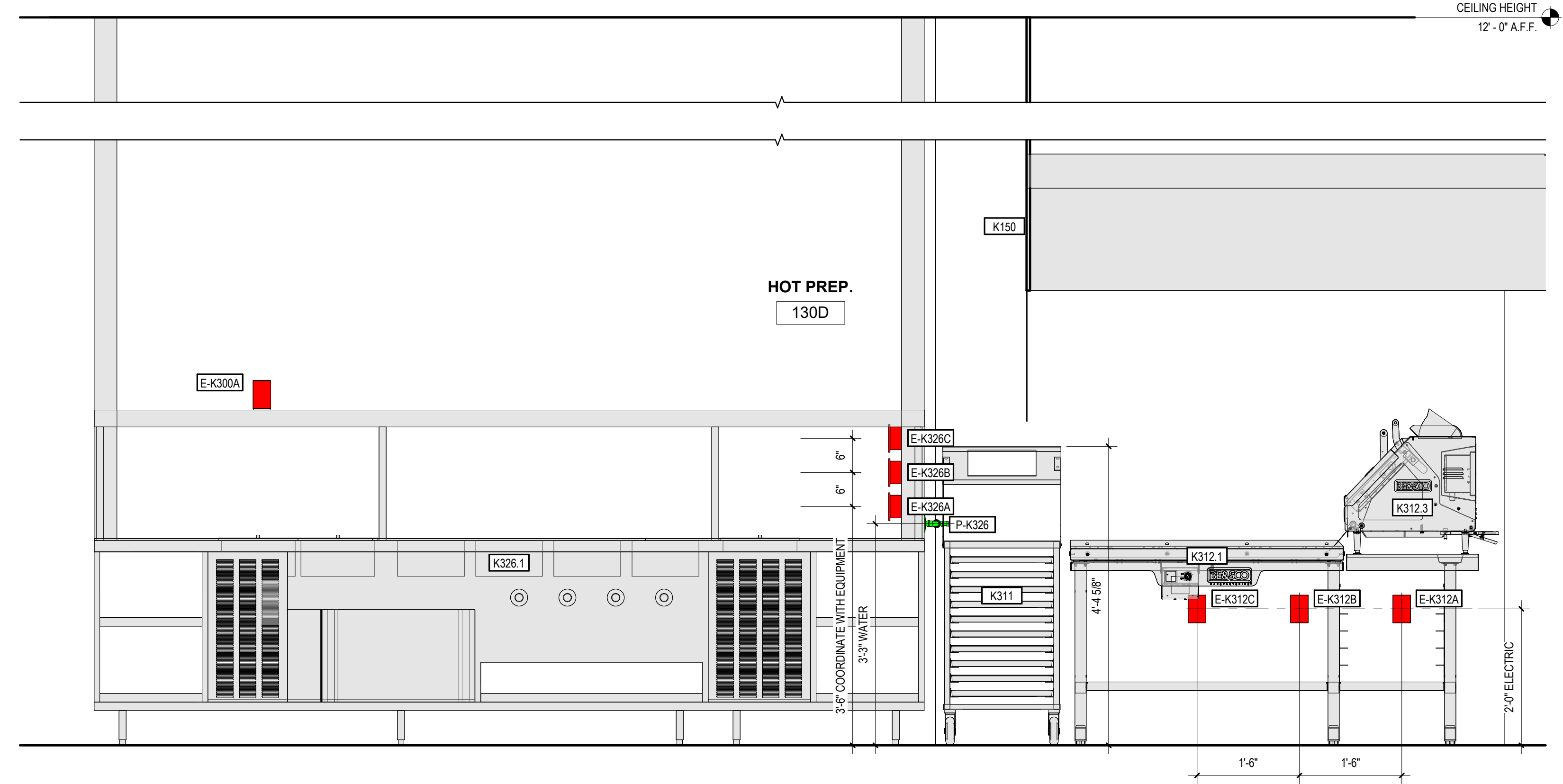
3 MAIN KITCHEN EQUIPMENT ELEVATION 3/4" = 1'-0"
