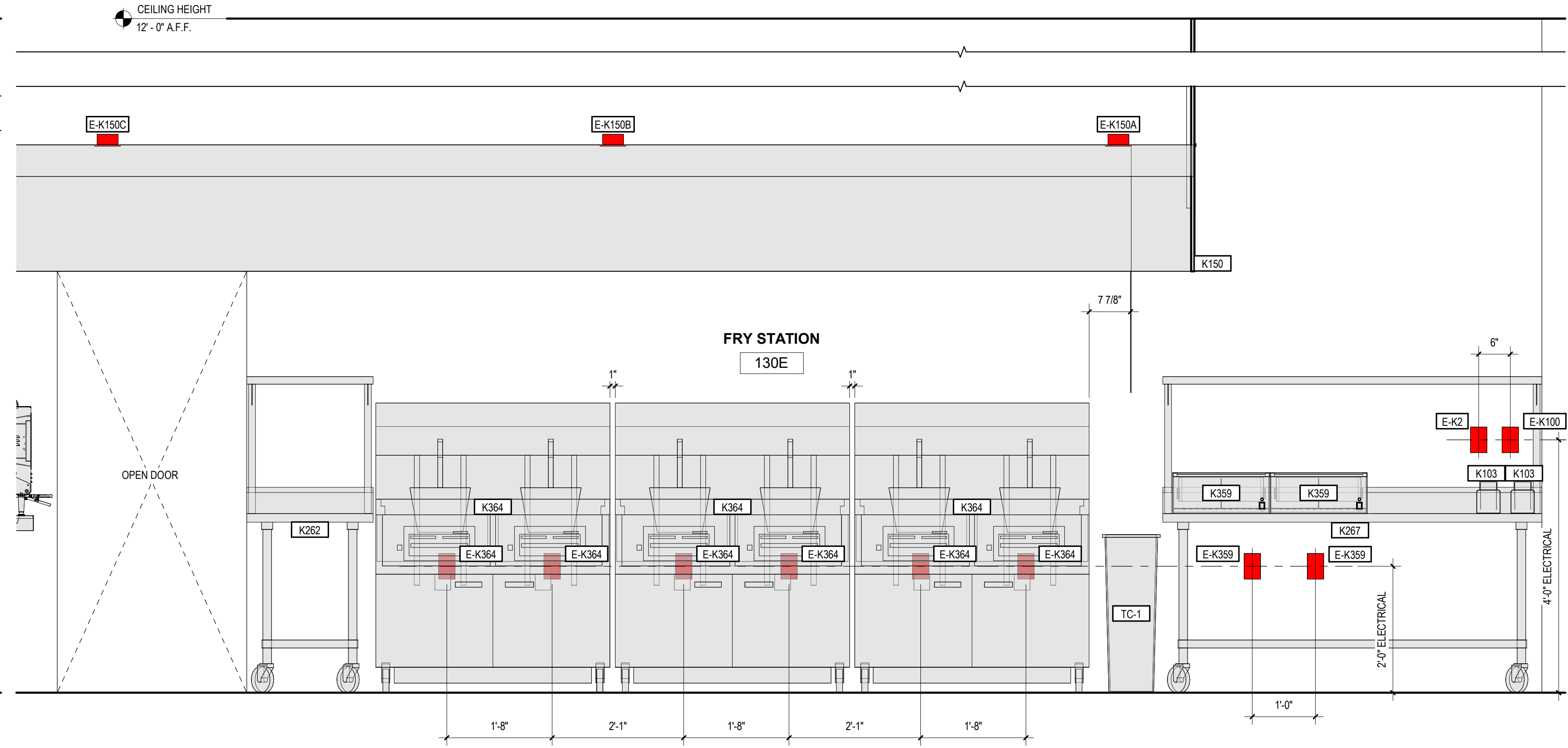
4 MAIN KITCHEN EQUIPMENT ELEVATION 3/4" = 1'-0"
