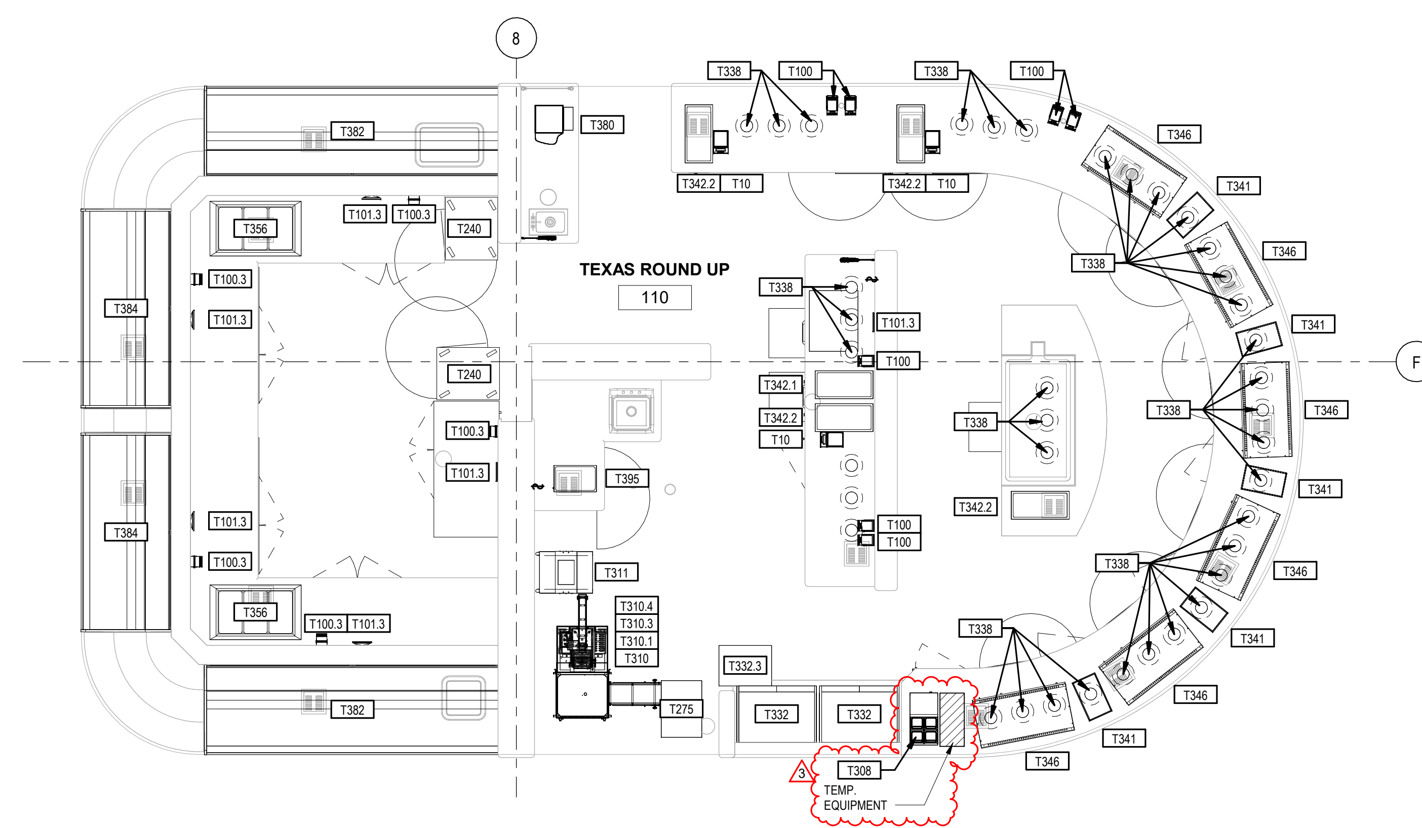
3 TEXAS ROUND UP EQUIPMENT PLAN - ABOVE COUNTER 1/4" = 1'-0"
