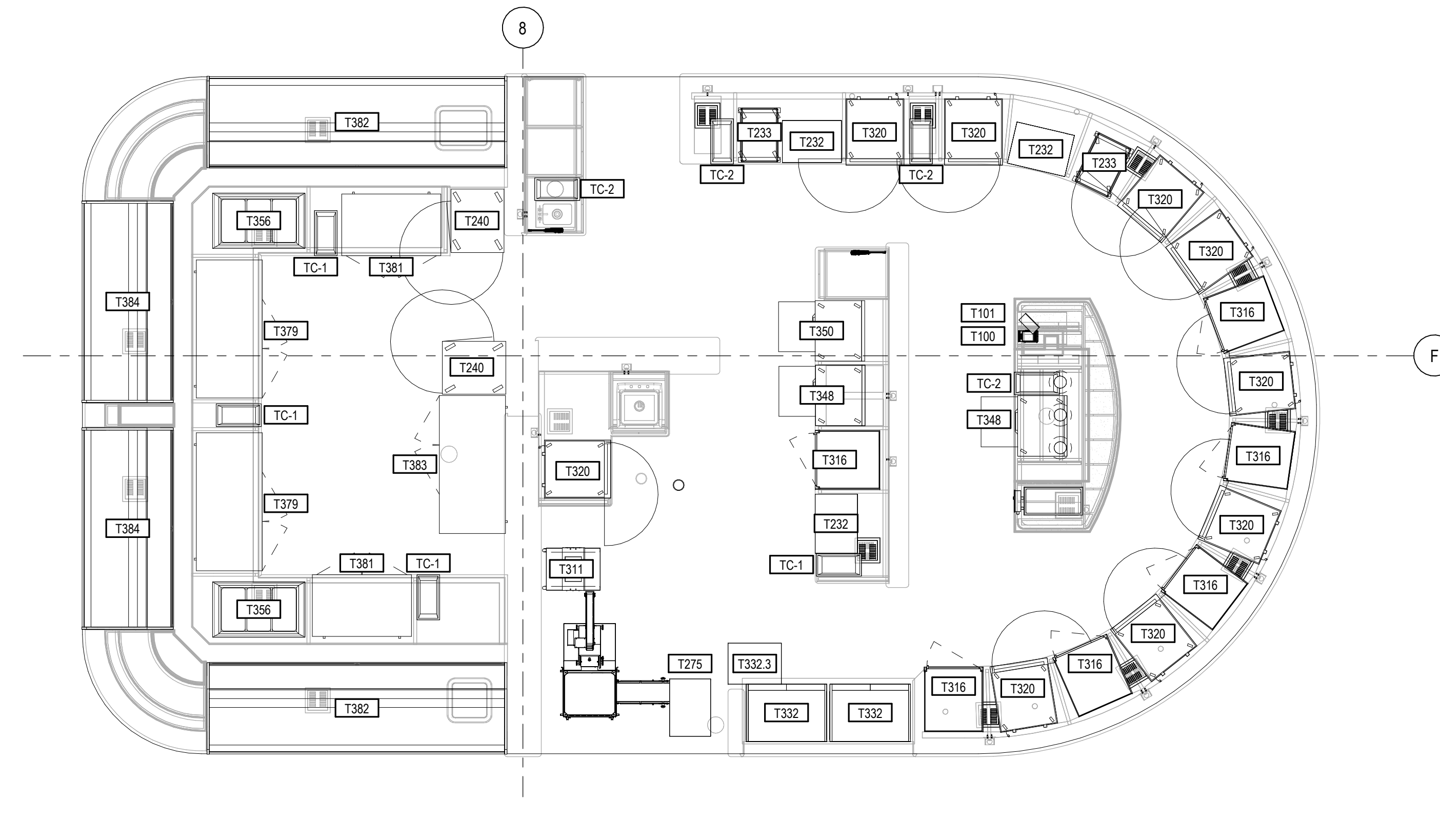
1 TEXAS ROUND UP EQUIPMENT PLAN - BELOW COUNTER 1/4" = 1'-0"
