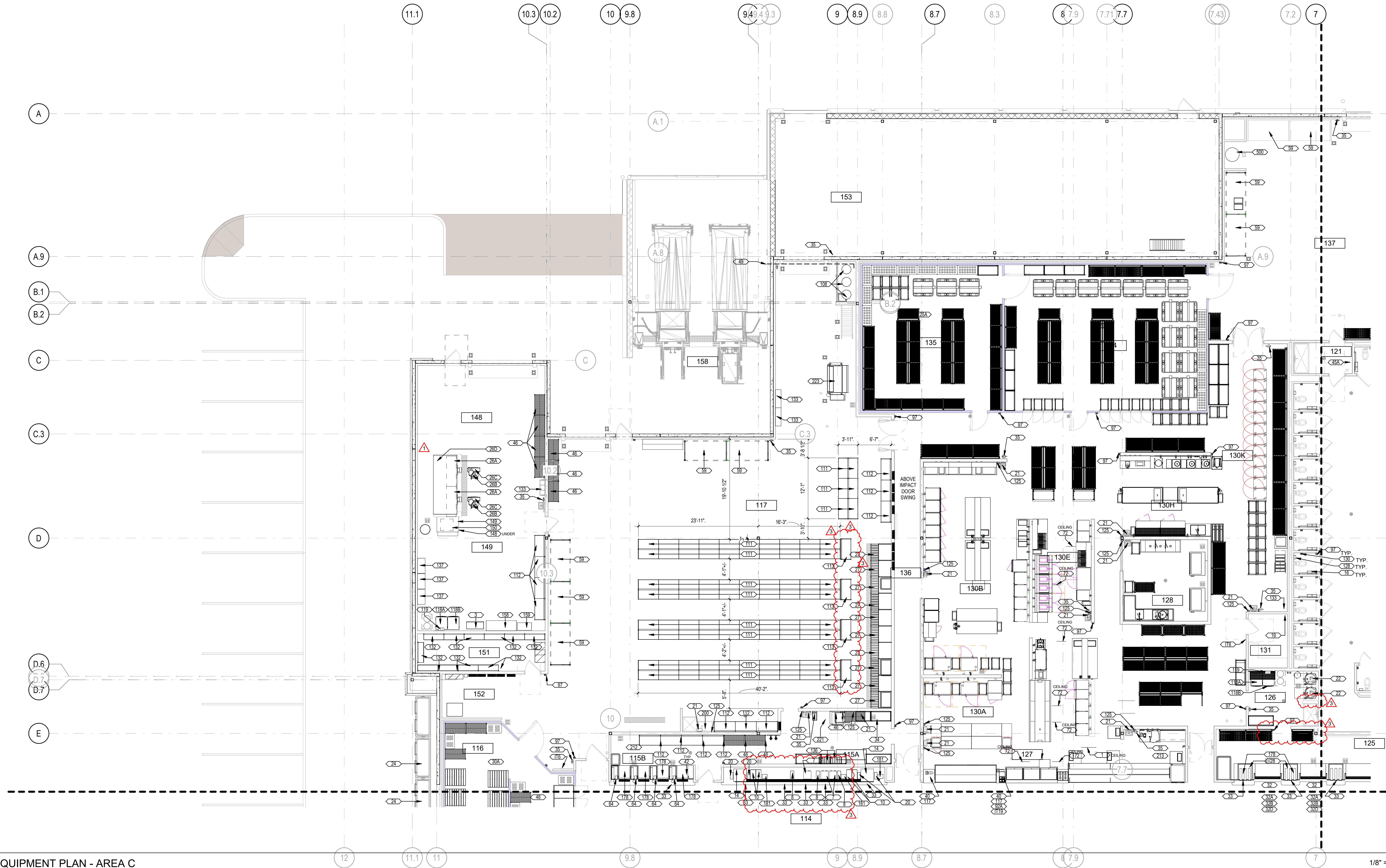
1 EQUIPMENT PLAN - AREA C
