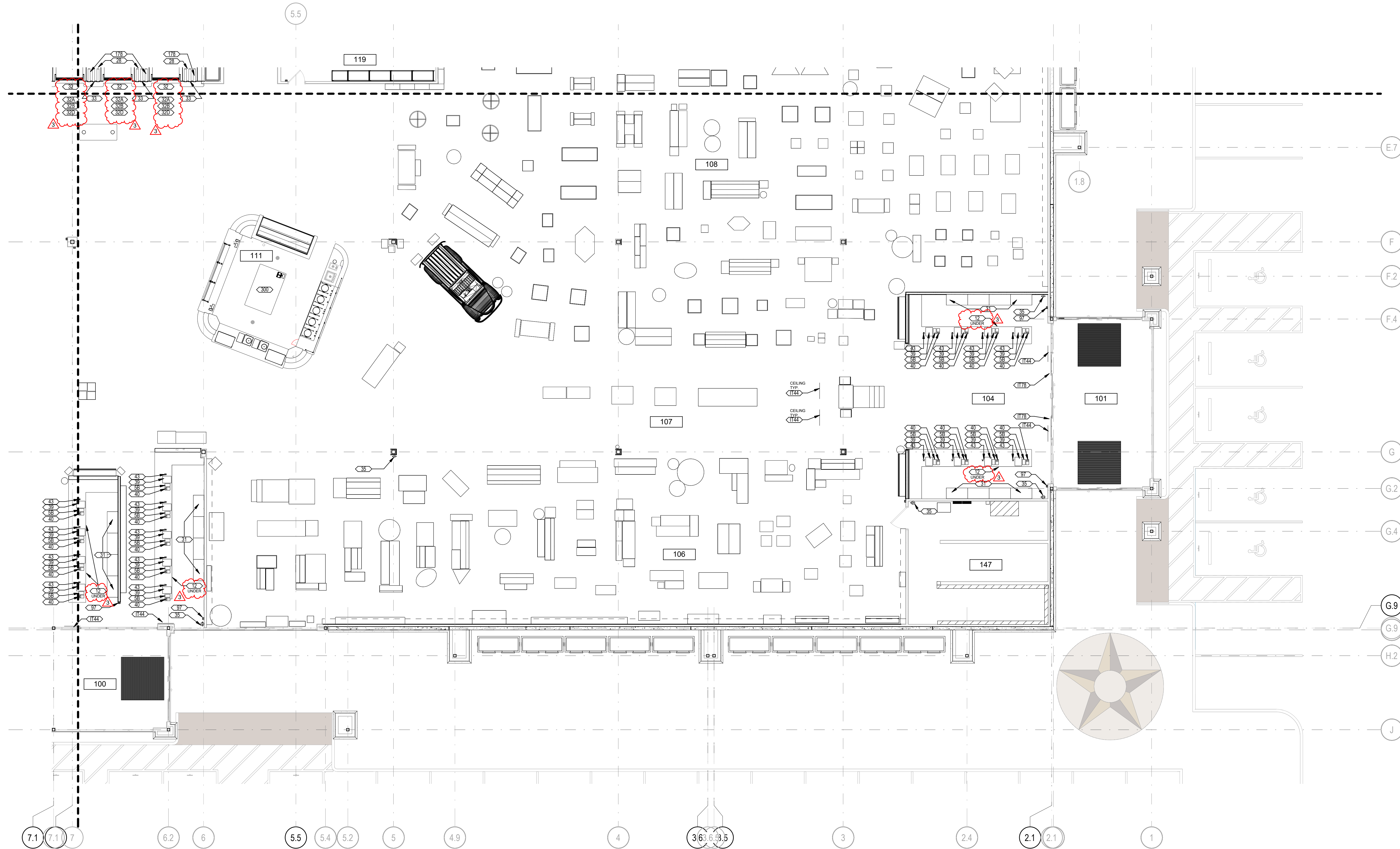
1 EQUIPMENT PLAN - AREA B
