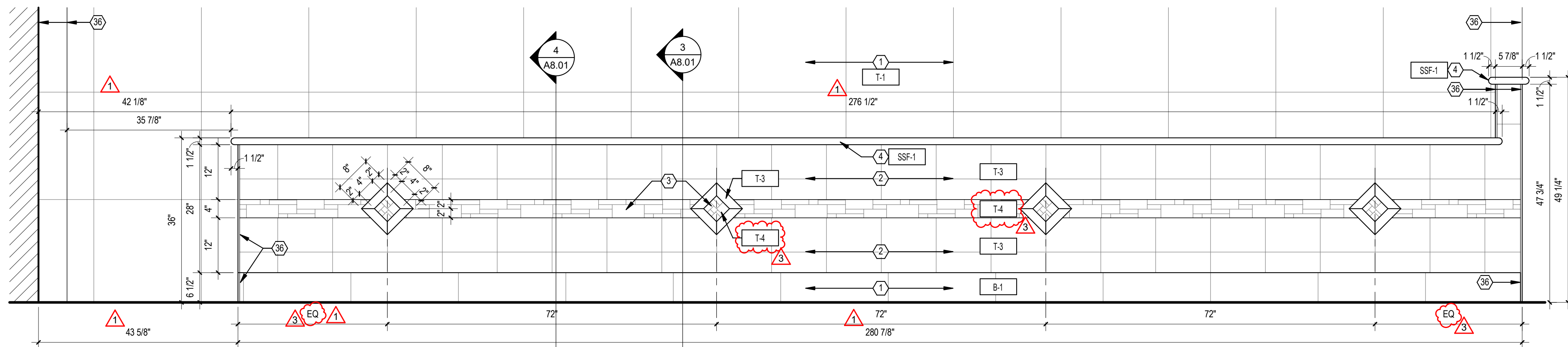
\frac{3}{4}'' = 1'-0''
