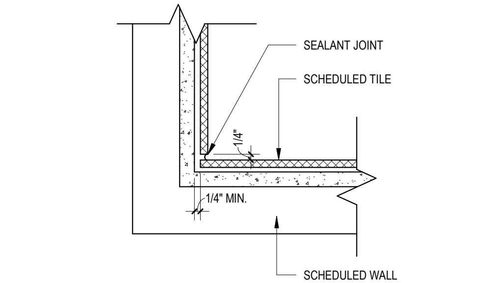
3 TYP. INSIDE CORNER 3" = 1'-0"
