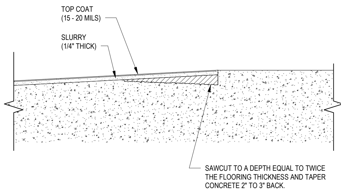
10 TRANSITION @ SLOPED FLOOR 3" = 1'-0"
