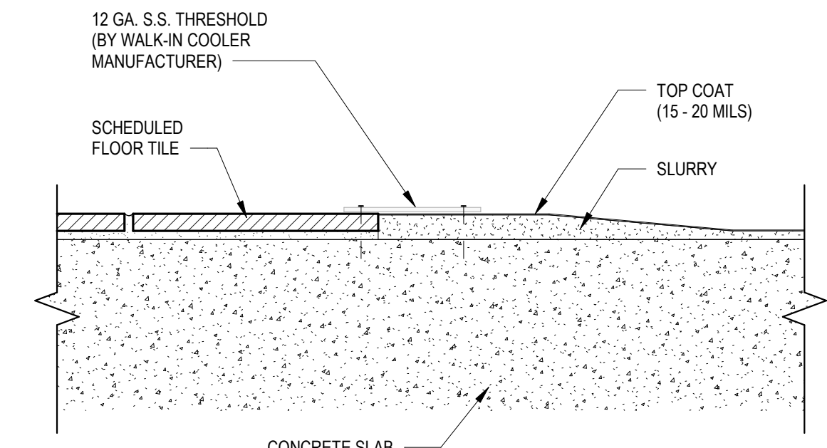
8 TRANSITION @ THRESHOLD 3" = 1'-0"
