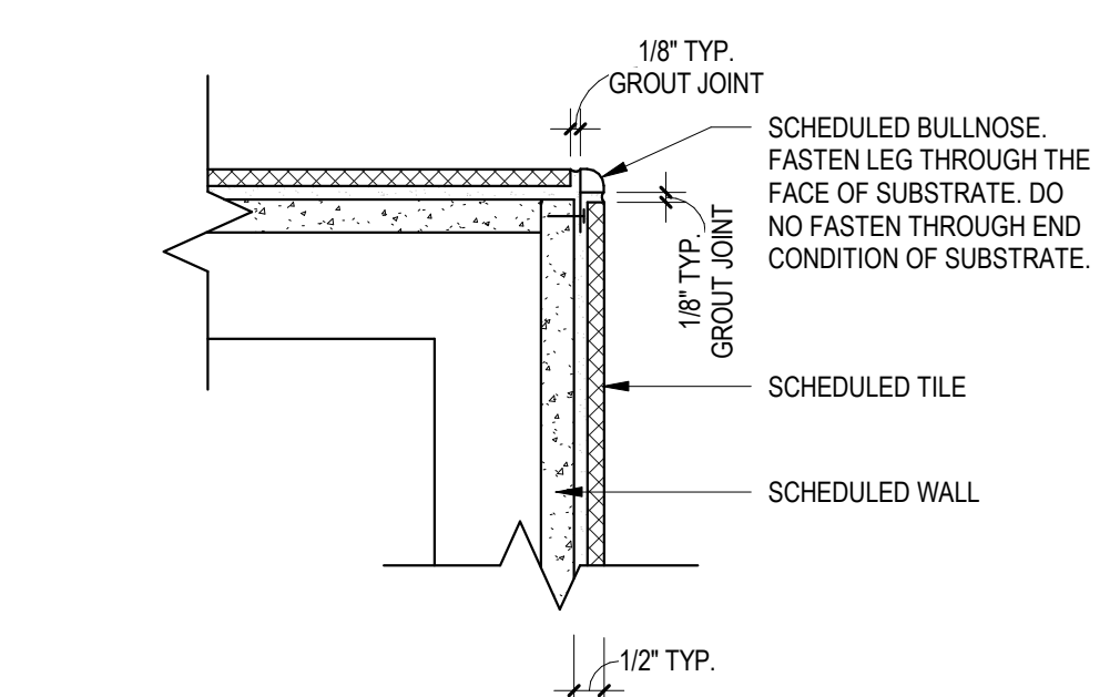
4 TYP. OUTSIDE CORNER 3" = 1'-0"
