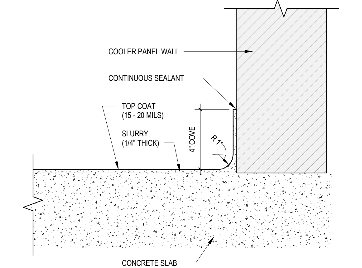
7 COVE BASE DETAIL 3" = 1'-0"
