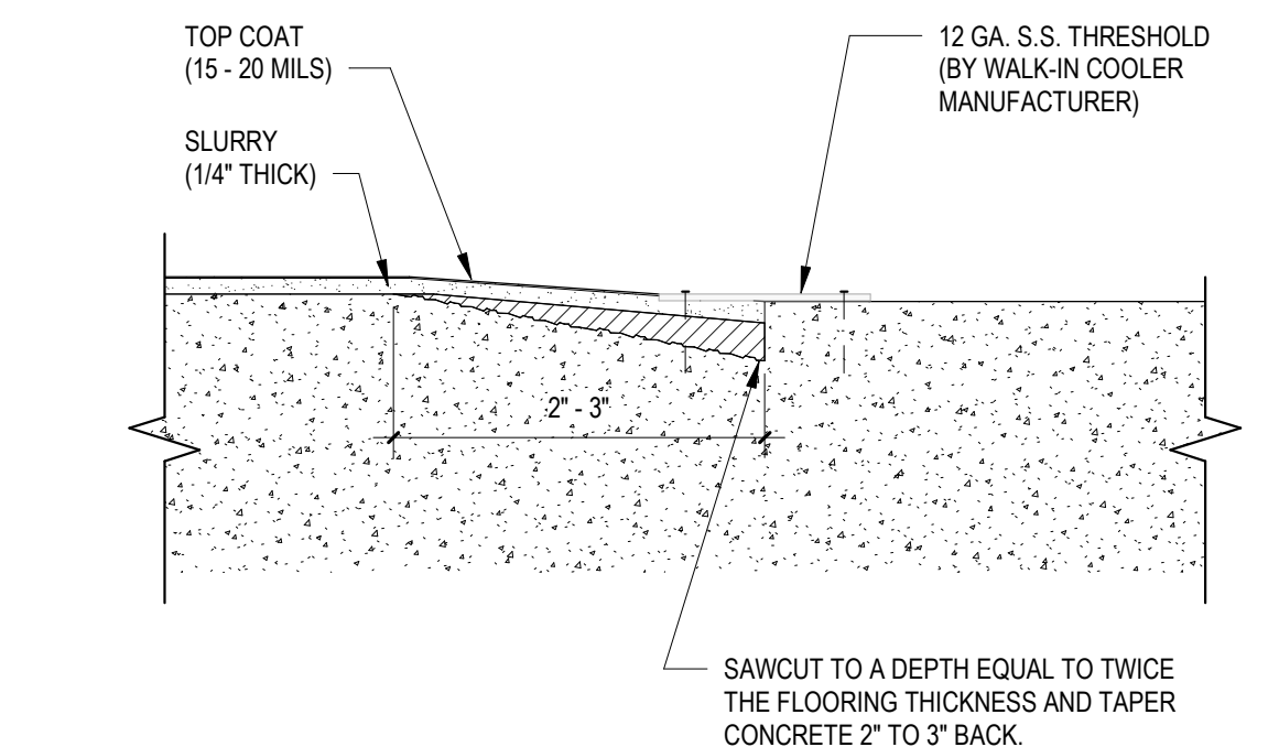
9 TRANSITION @ THRESHOLD 3" = 1'-0"
