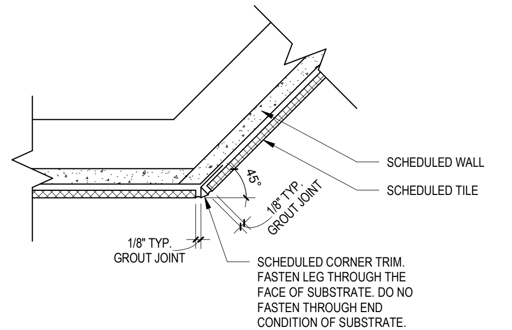
5 TYP. 45° OUTSIDE CORNER 3" = 1'-0"
