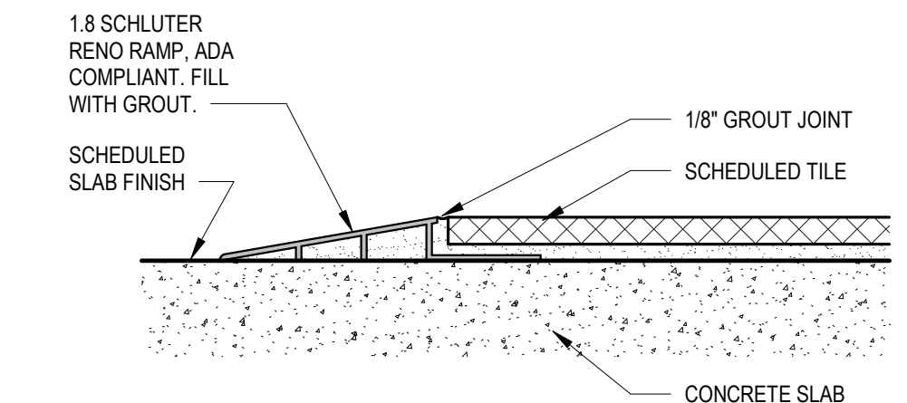
2 TILE TRANSITION 6" = 1'-0"
