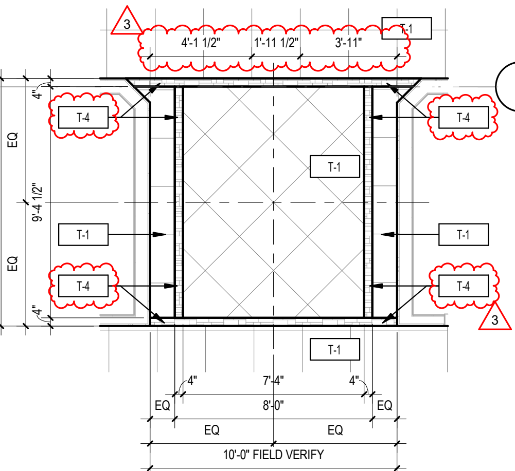
1 ENLARGED FINISH PLAN 1/4" = 1'-0"
