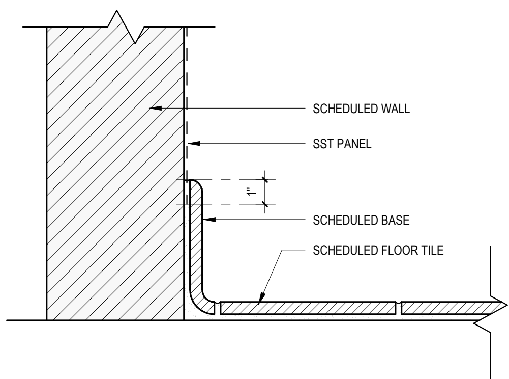
6 SST PANEL AT BASE 3" = 1'-0"
