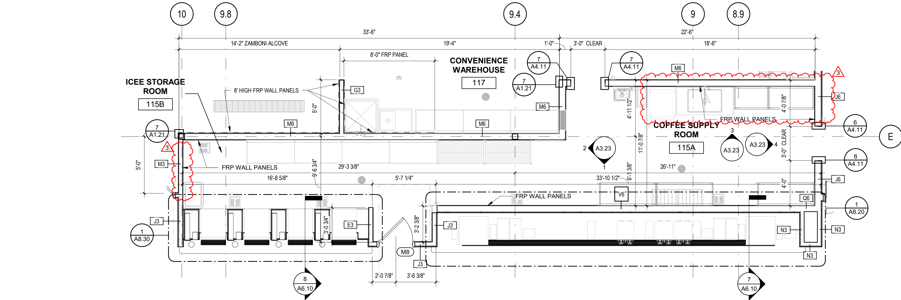
4 ENLARGED PLAN - COFFEE & ICEE COUNTER 1/4" = 1'-0"
