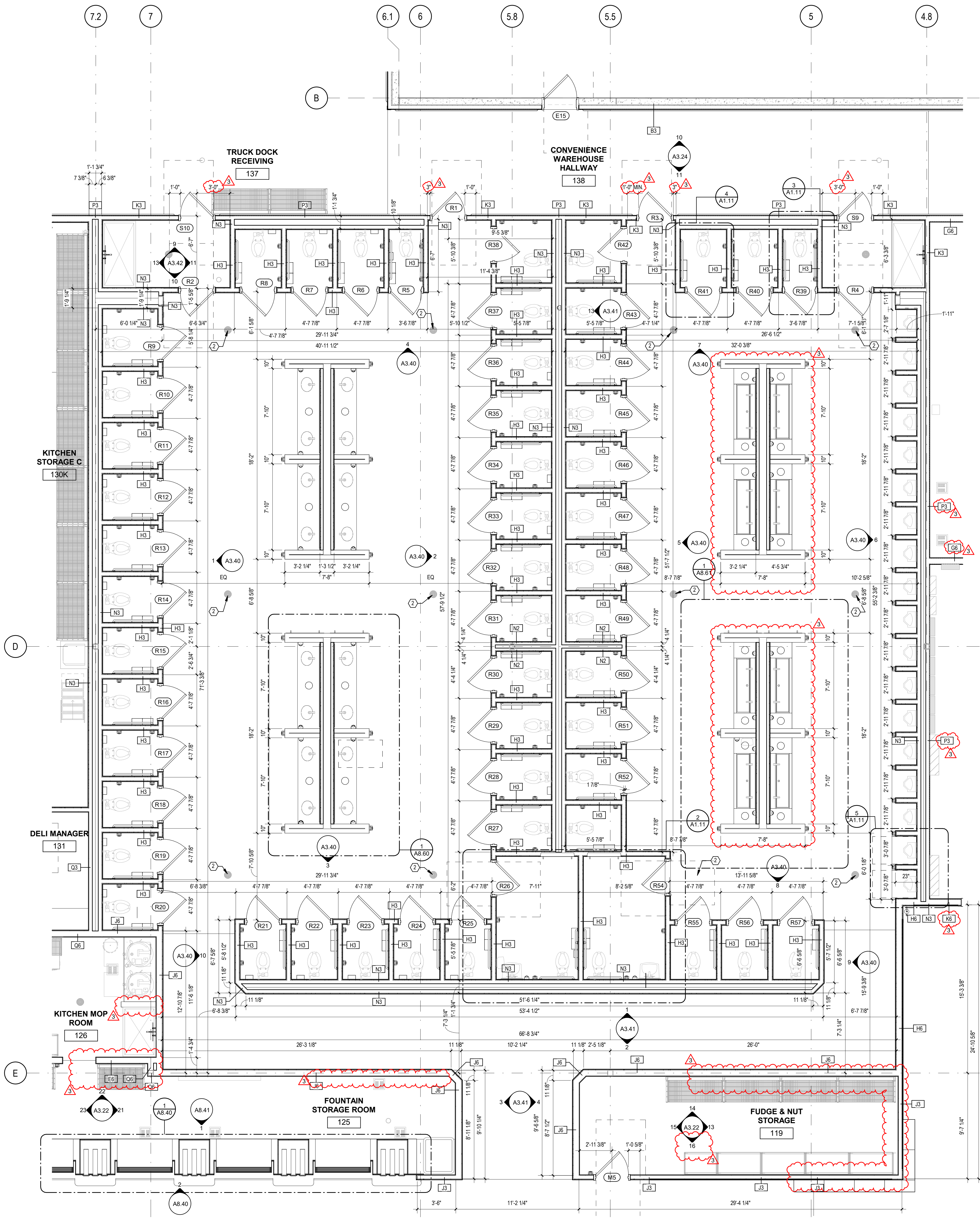
1 ENLARGED RESTROOM PLAN
