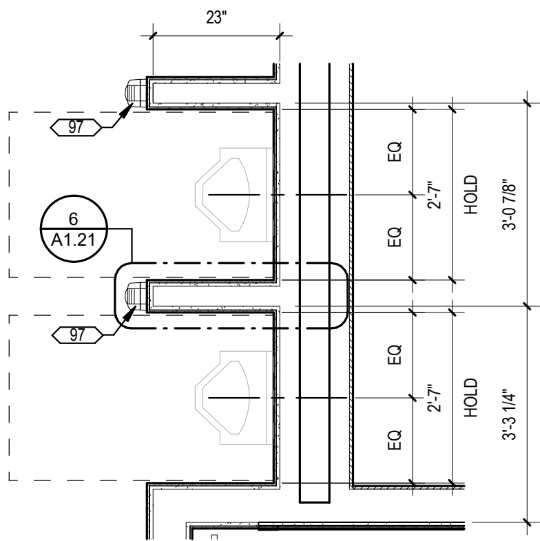
5 ADA URINAL 1/2" = 1'-0"
