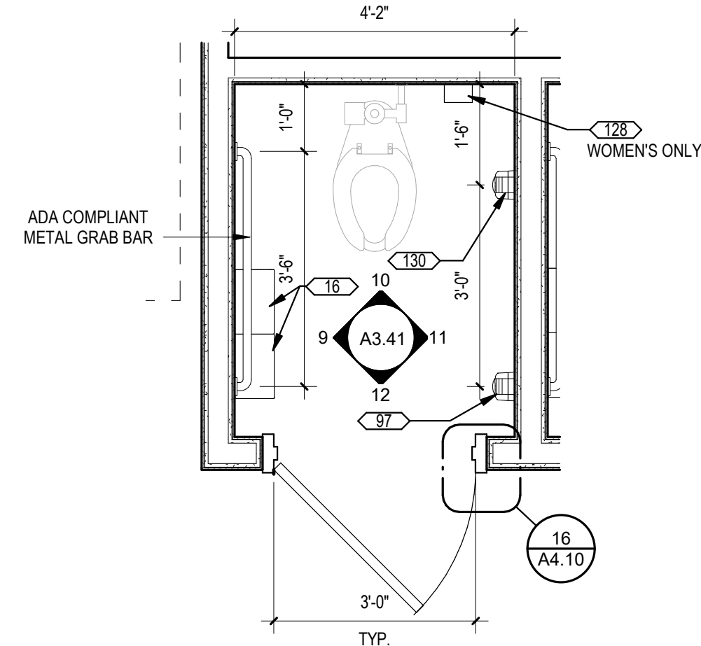
4 TYPICAL TOILET STALL 1/2" = 1'-0"
