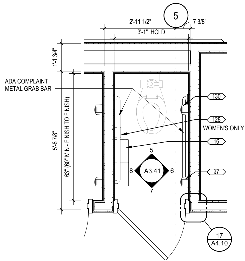
3 ADA AMBULATORY STALL 1/2" = 1'-0"
