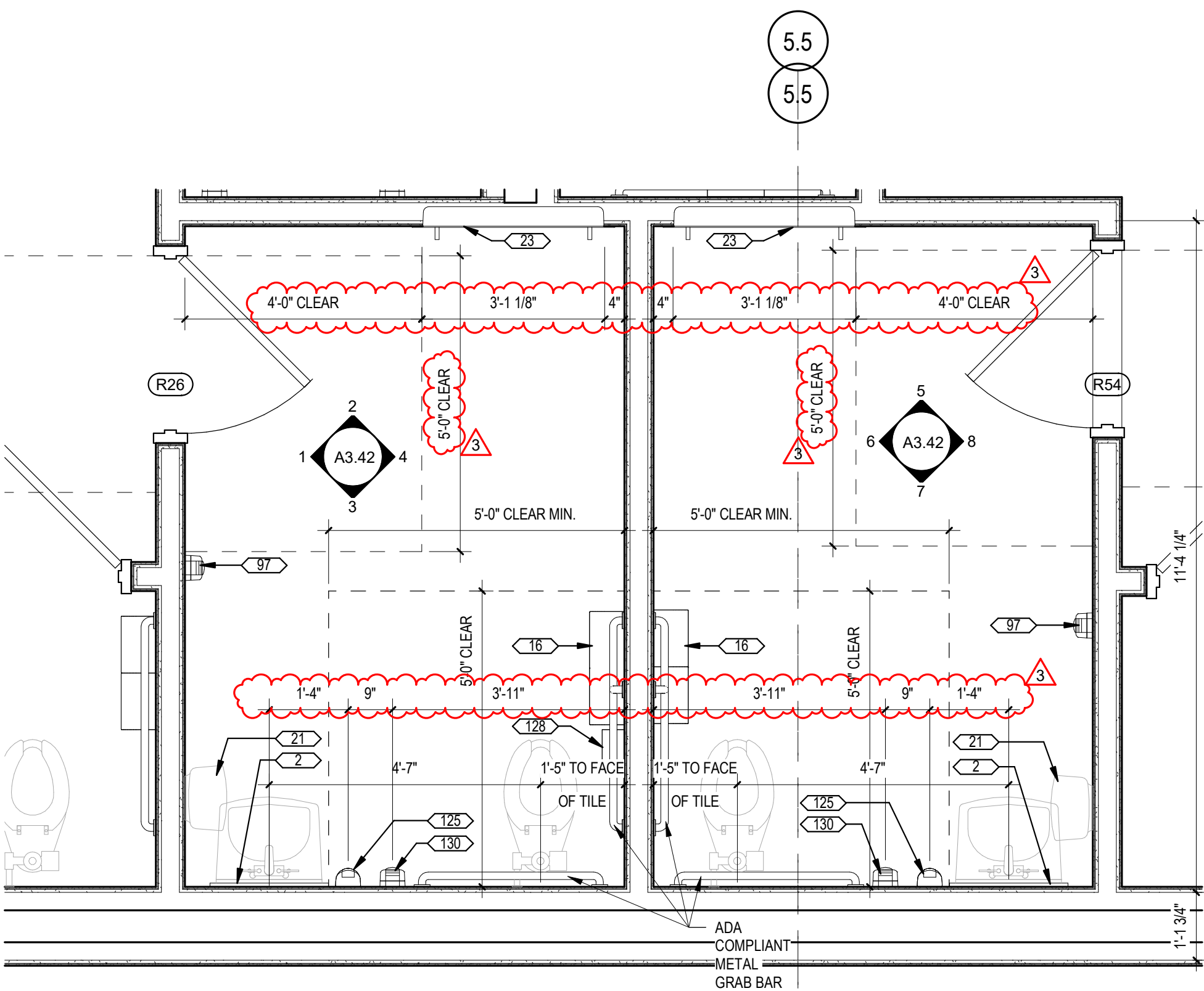
2 ENLARGED RESTROOM PLAN - ACCESSIBLE STALLS 1/2" = 1'-0"
