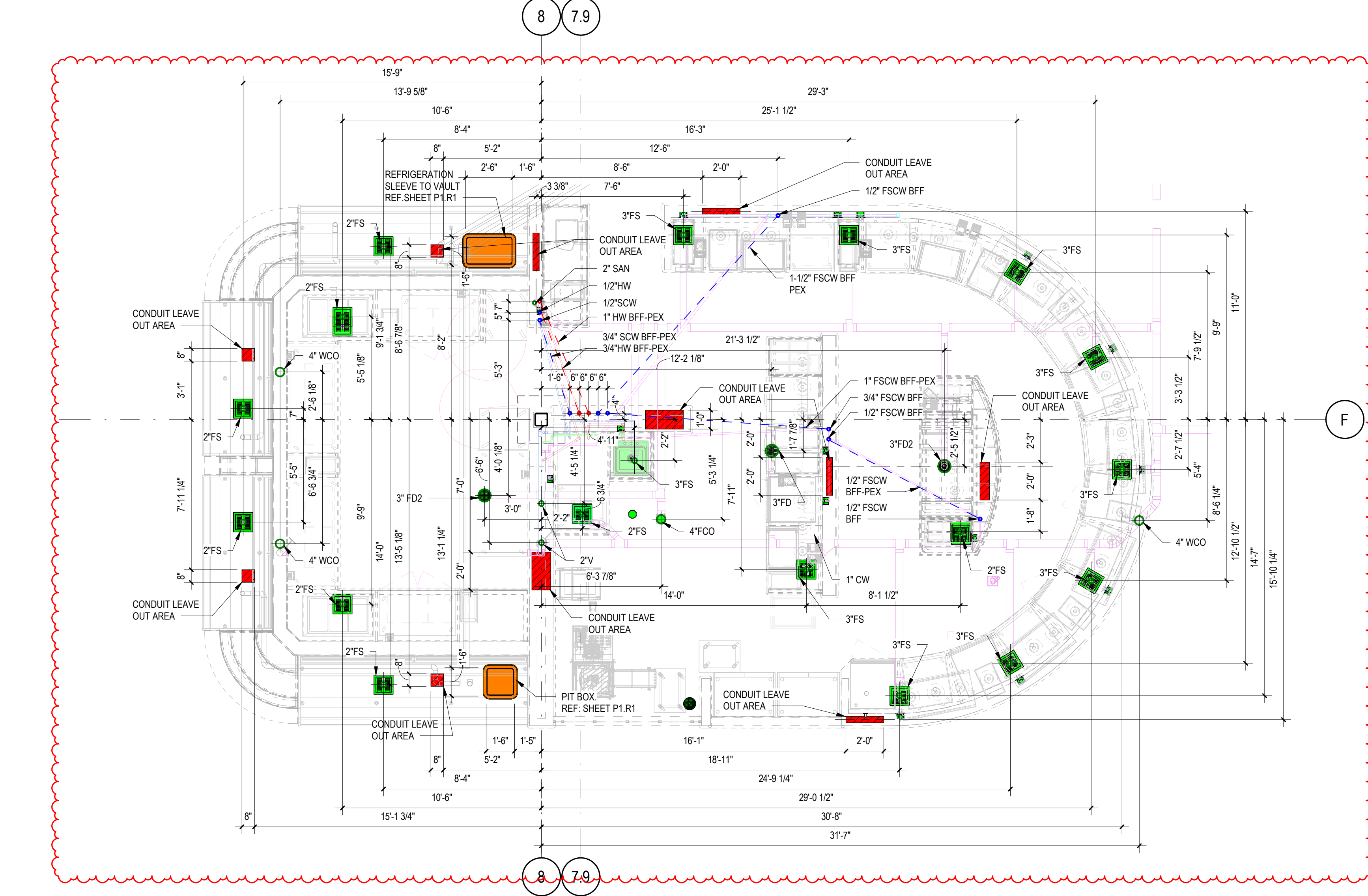
2 STUB UP PLAN - TEXAS ROUND UP
