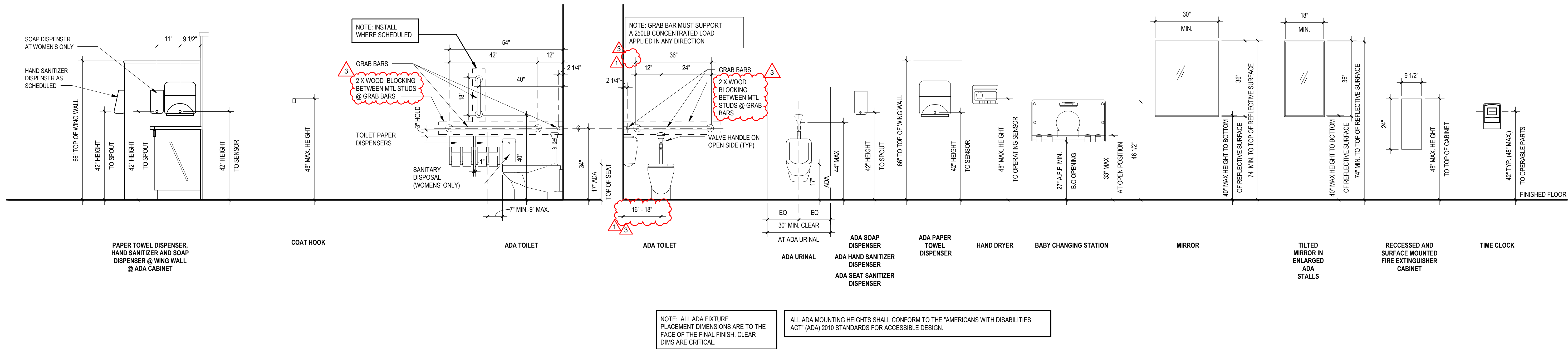
1 ADA MOUNTING HEIGHTS 1/2" = 1'-0"
