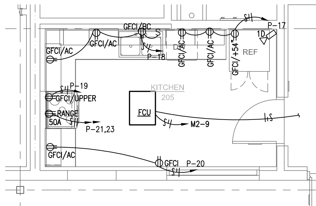
3 POWER AND SYSTEMS PLAN - SECOND FLOOR ENLARGED SCALE: 1/4" = 1'-0"
