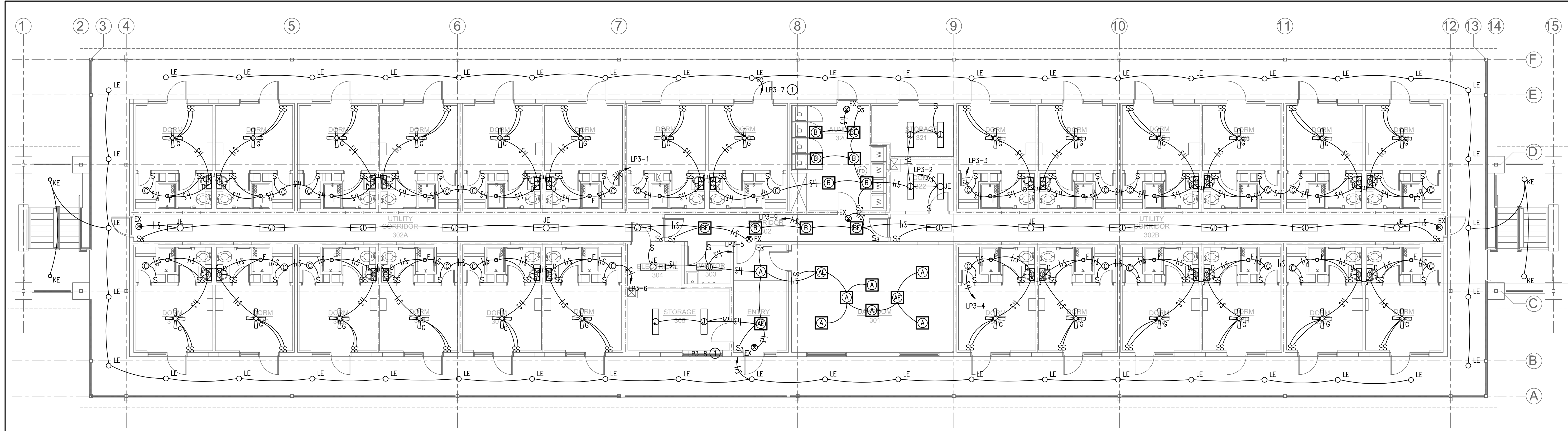
1 LIGHTING PLAN - THIRD FLOOR SCALE: 1/8" = 1'-0"
