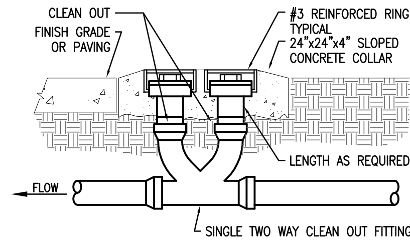
2 DOUBLE CLEAN OUT TO GRADE DETAIL SCALE: NONE
