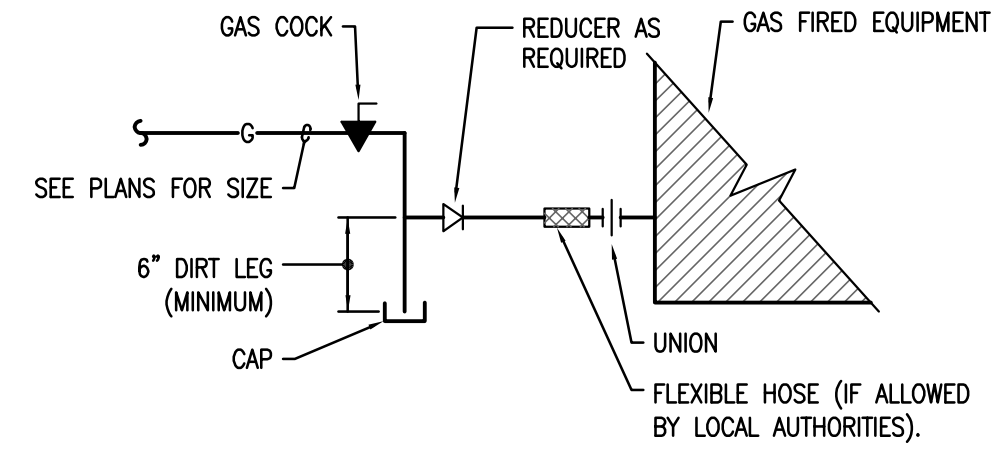
4 NATURAL GAS CONNECTION DETAIL SCALE: NONE
