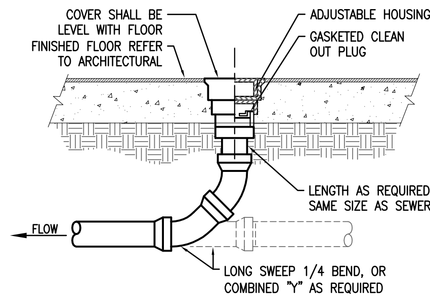
3 FLOOR CLEAN OUT (FCO) DETAIL SCALE: NONE
