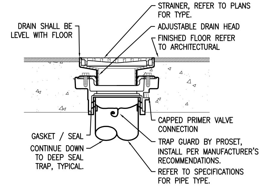
5 TYPICAL FLOOR DRAIN DETAIL SCALE: NONE
