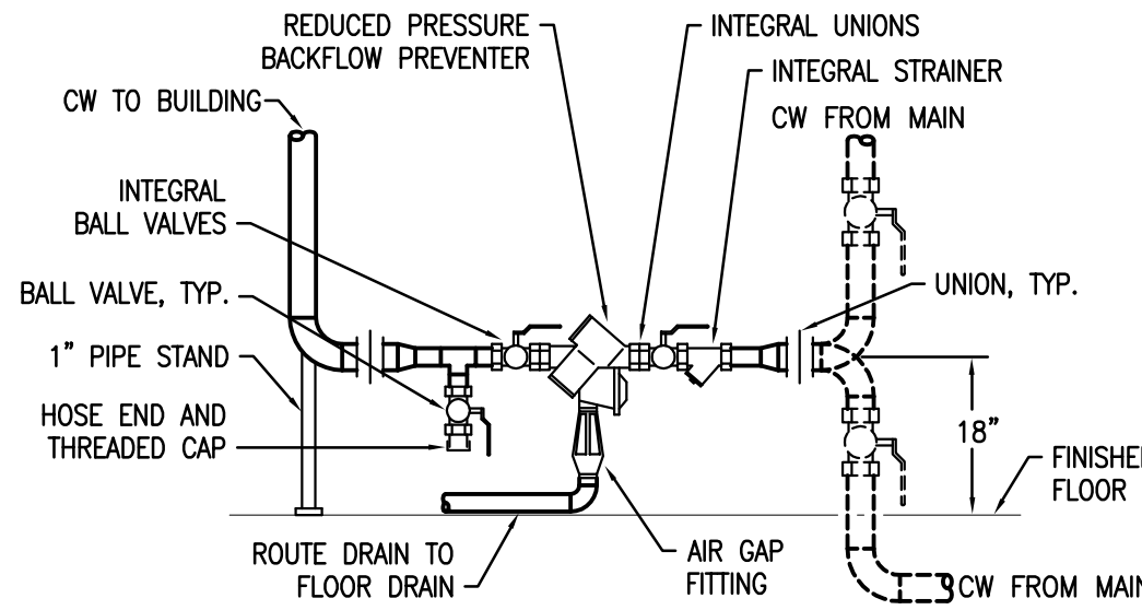
7 DOMESTIC WATER RPZ DETAIL SCALE: NONE
