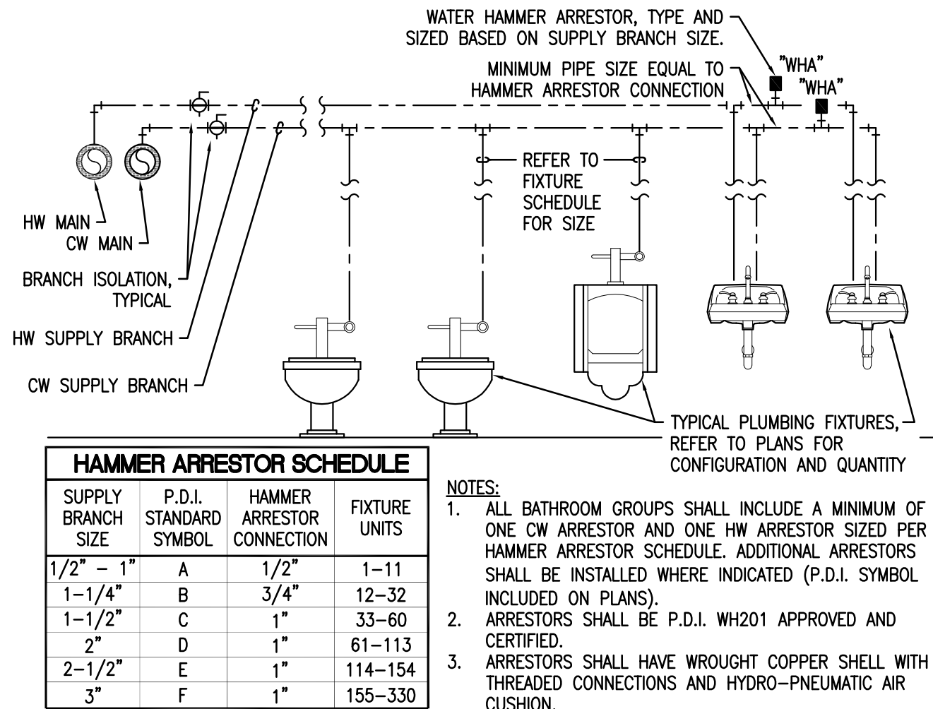
6 WATER HAMMER ARRESTOR DETAIL SCALE: NONE
