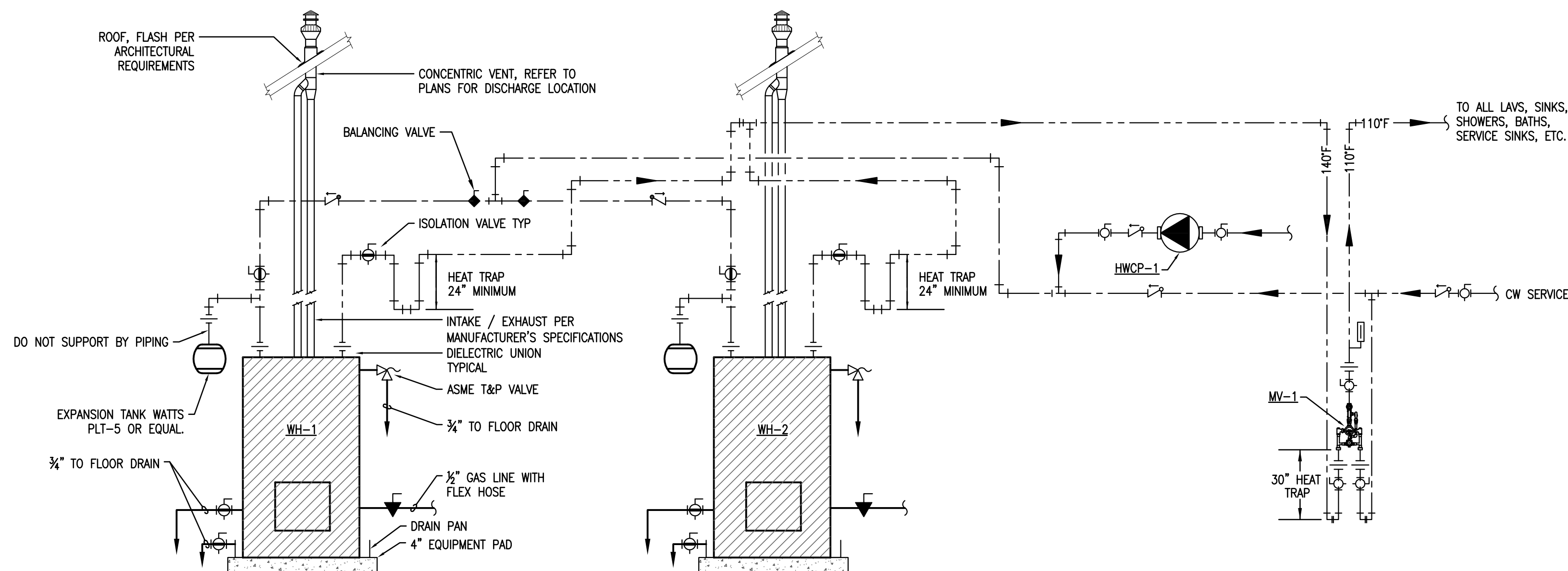
8 WATER HEATER PIPING DIAGRAM SCALE: NONE
