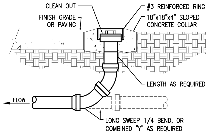
1 CLEAN OUT TO GRADE DETAIL SCALE: NONE
