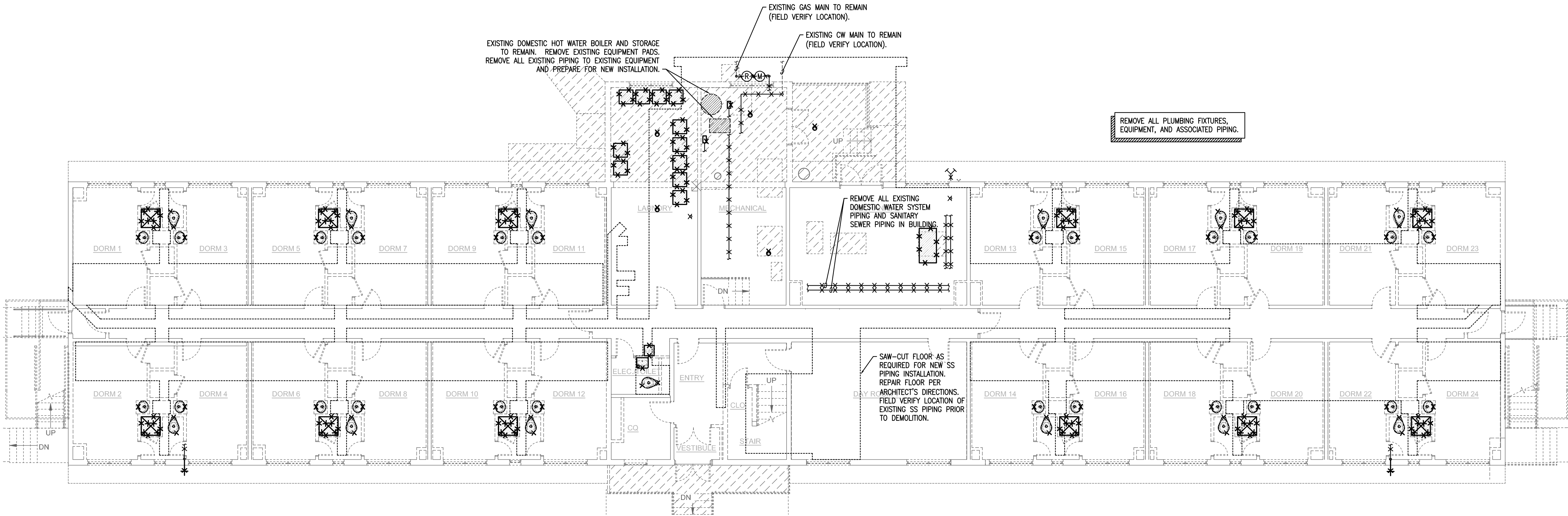
1 FIRST FLOOR PLUMBING DEMOLITION PLAN SCALE: 1/8" = 1'-0"
