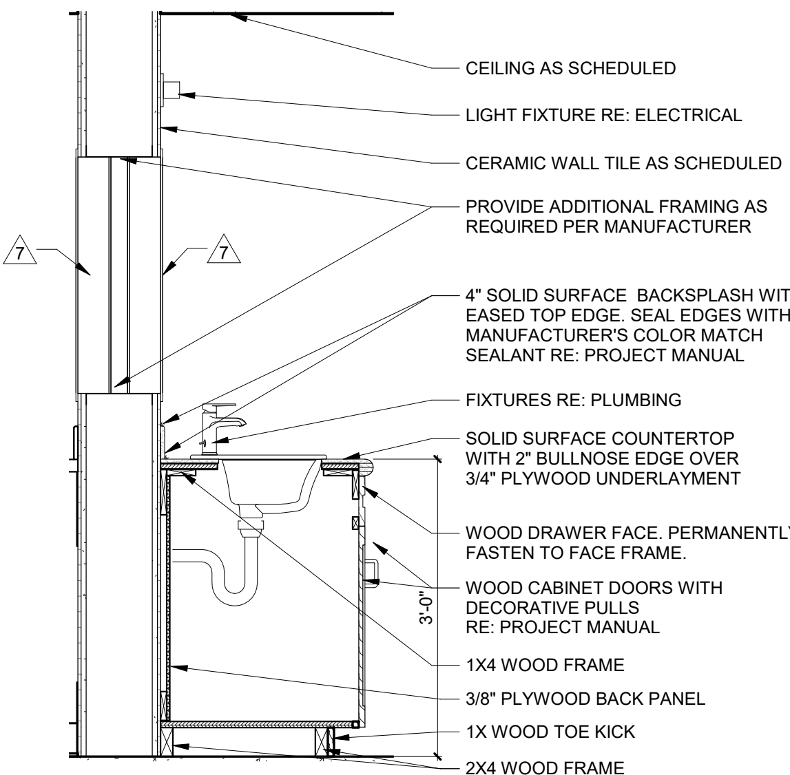
8 DORM VANITY SECTION 3/4\"/>
