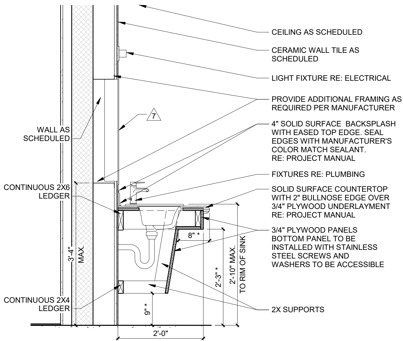
6 ADA VANITY SECTION 3/4\"/>
