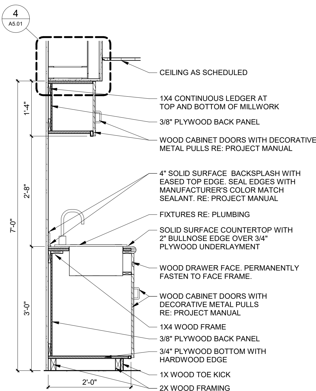
2 KITCHEN CABINET SECTION @ SINK 3/4\"/>
