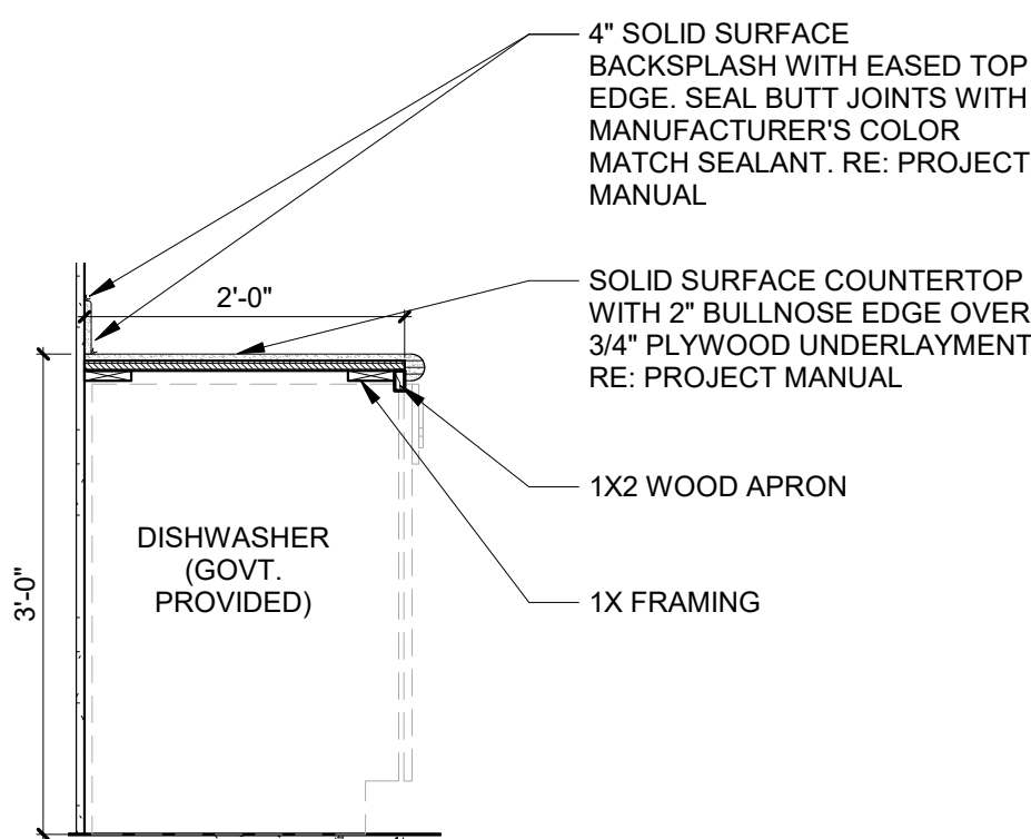
3 KITCHEN CABINET SECTION @ DW 3/4\"/>
