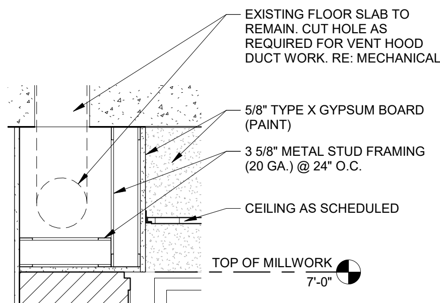
4 FURR DOWN @ KITCHEN 205 1\"/>
