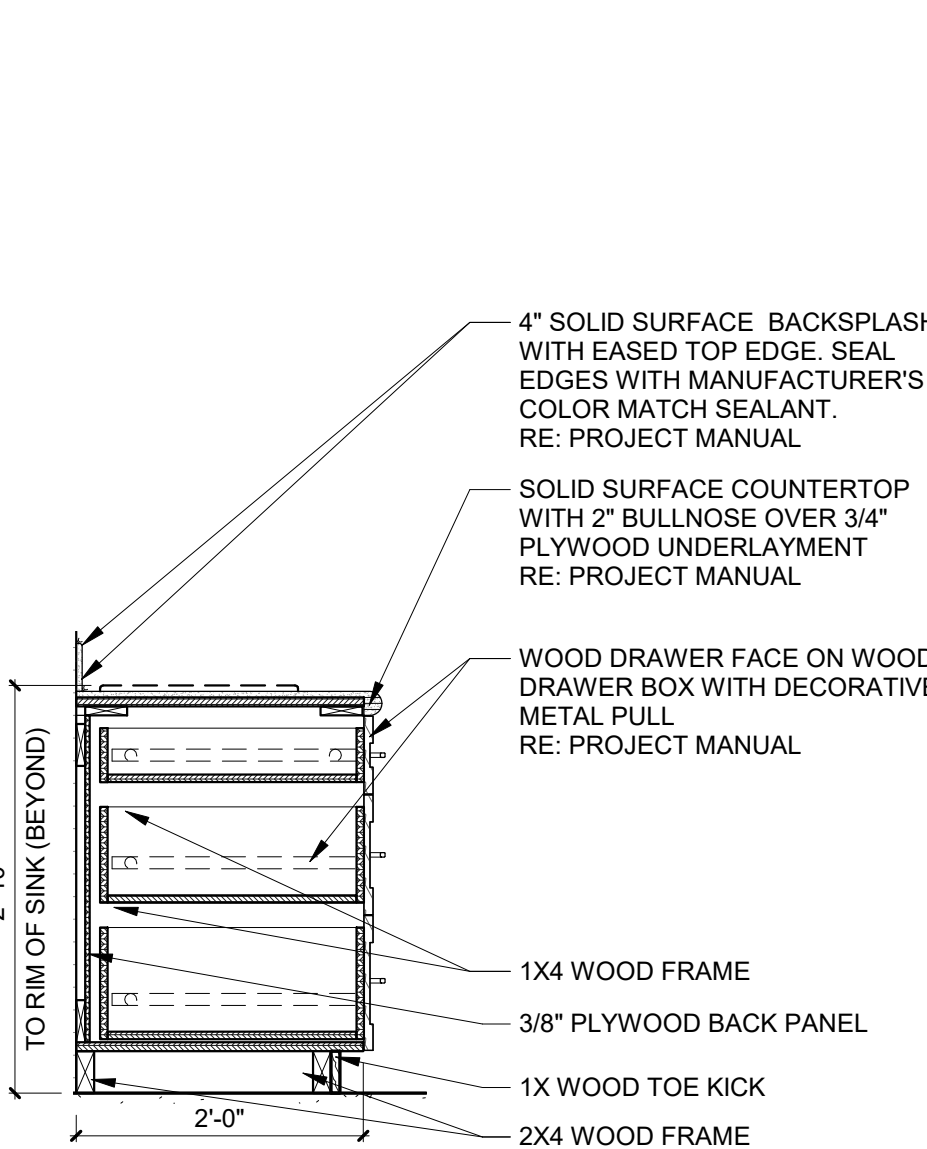
7 ADA VANITY DRAWER SECTION 3/4\"/>
