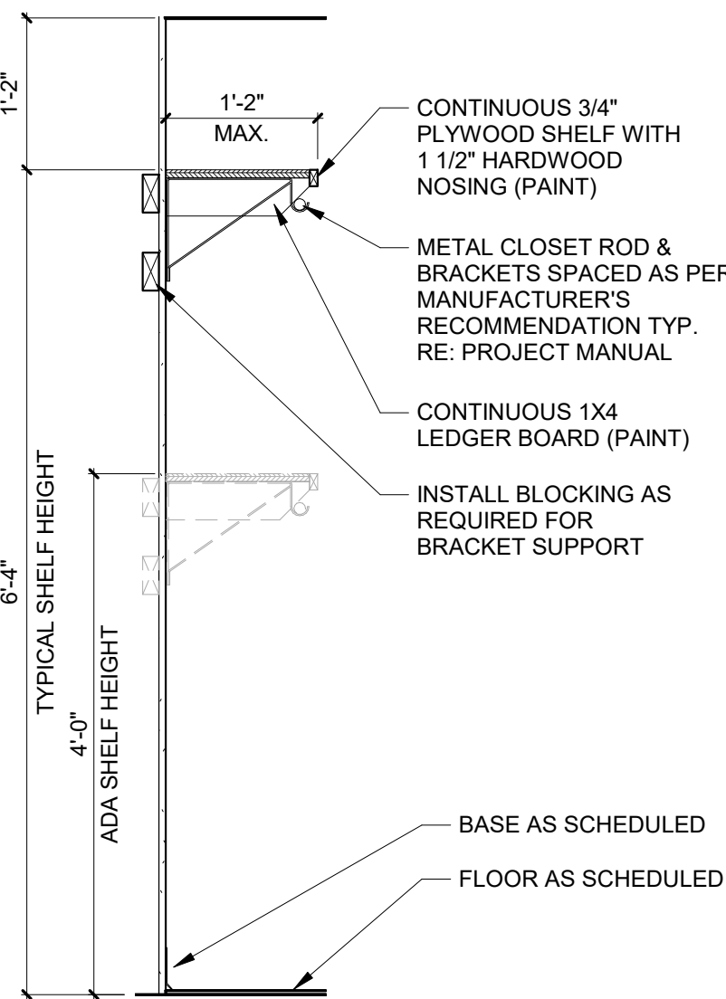
10 CLOSET SHELF SECTION 3/4\"/>
