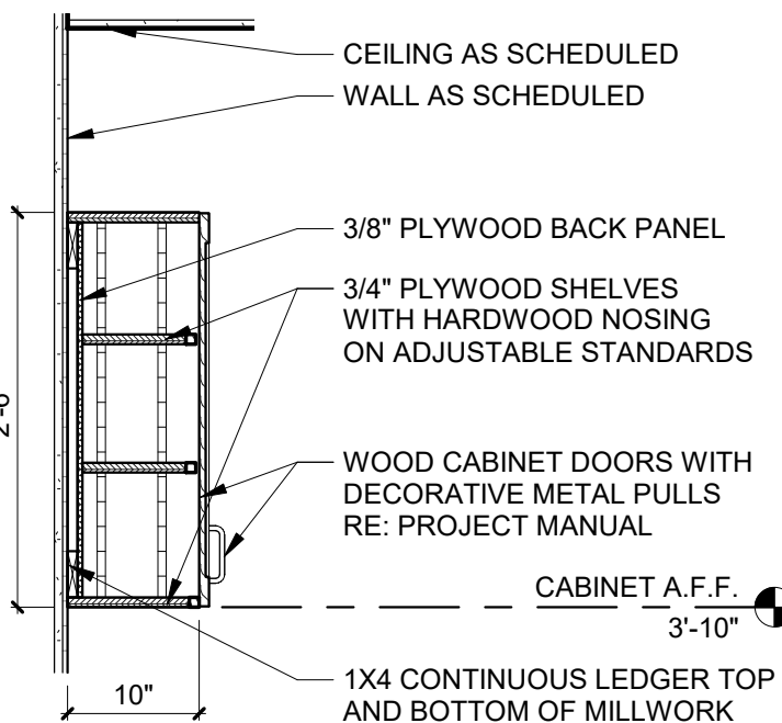
5 BATHROOM UPPER CABINET SECTION (TYP) 3/4\"/>
