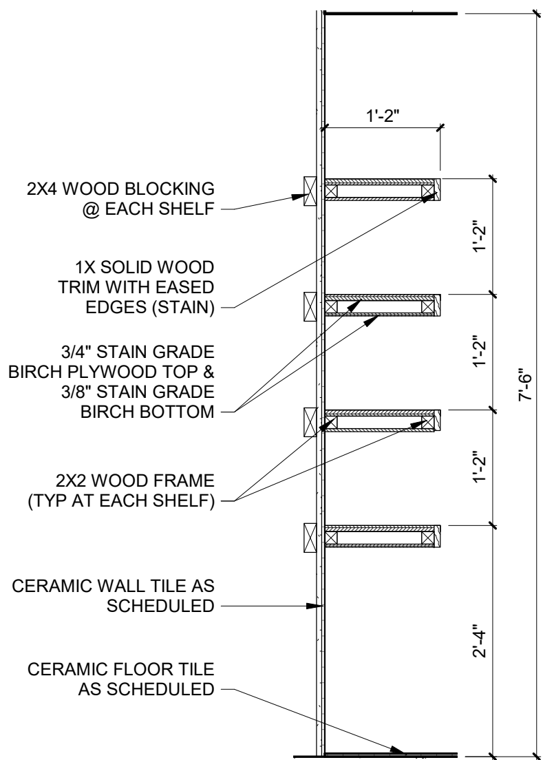
9 DORM SHELVES SECTION 3/4\"/>
