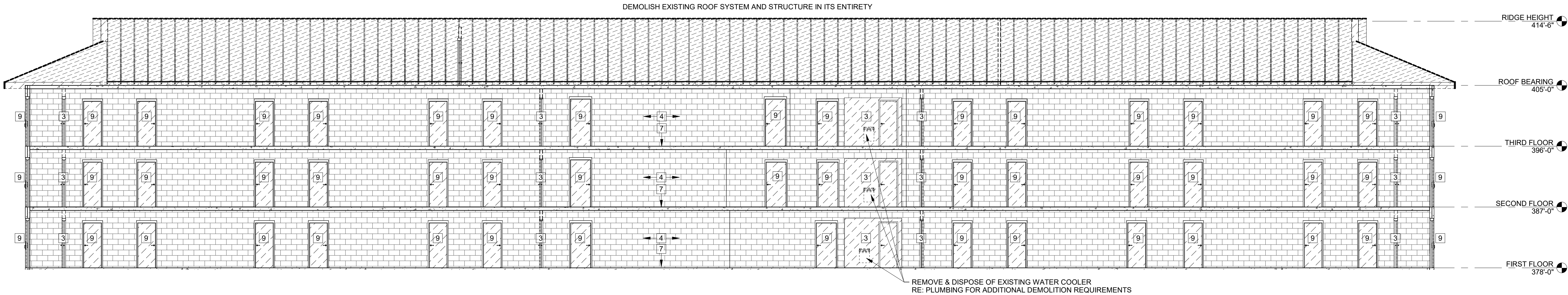
2 EXISTING BUILDING SECTION FACING SOUTH 1/8" = 1'-0"
