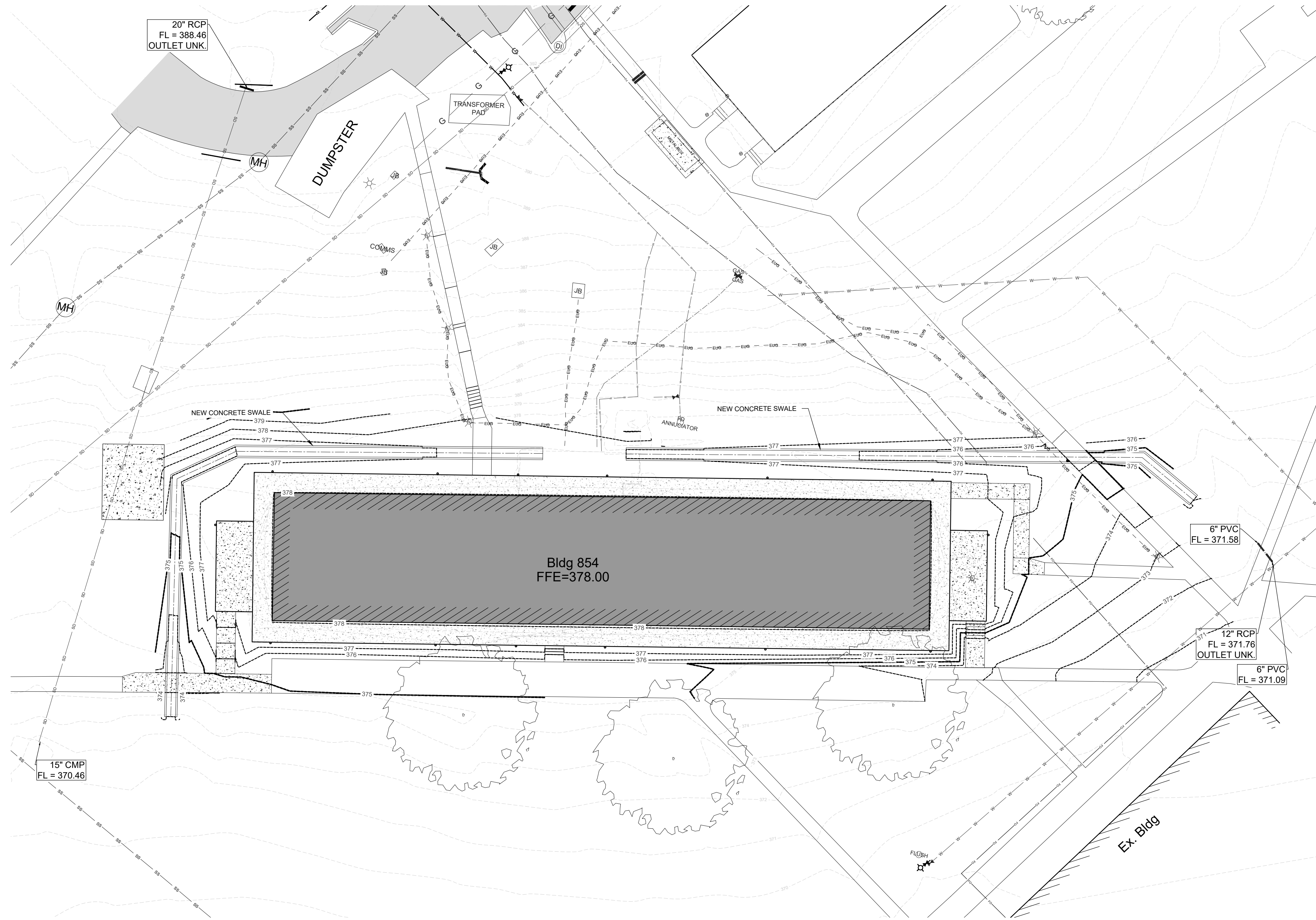
1 CIVIL SITE PLAN SCALE: 1" = 20'
