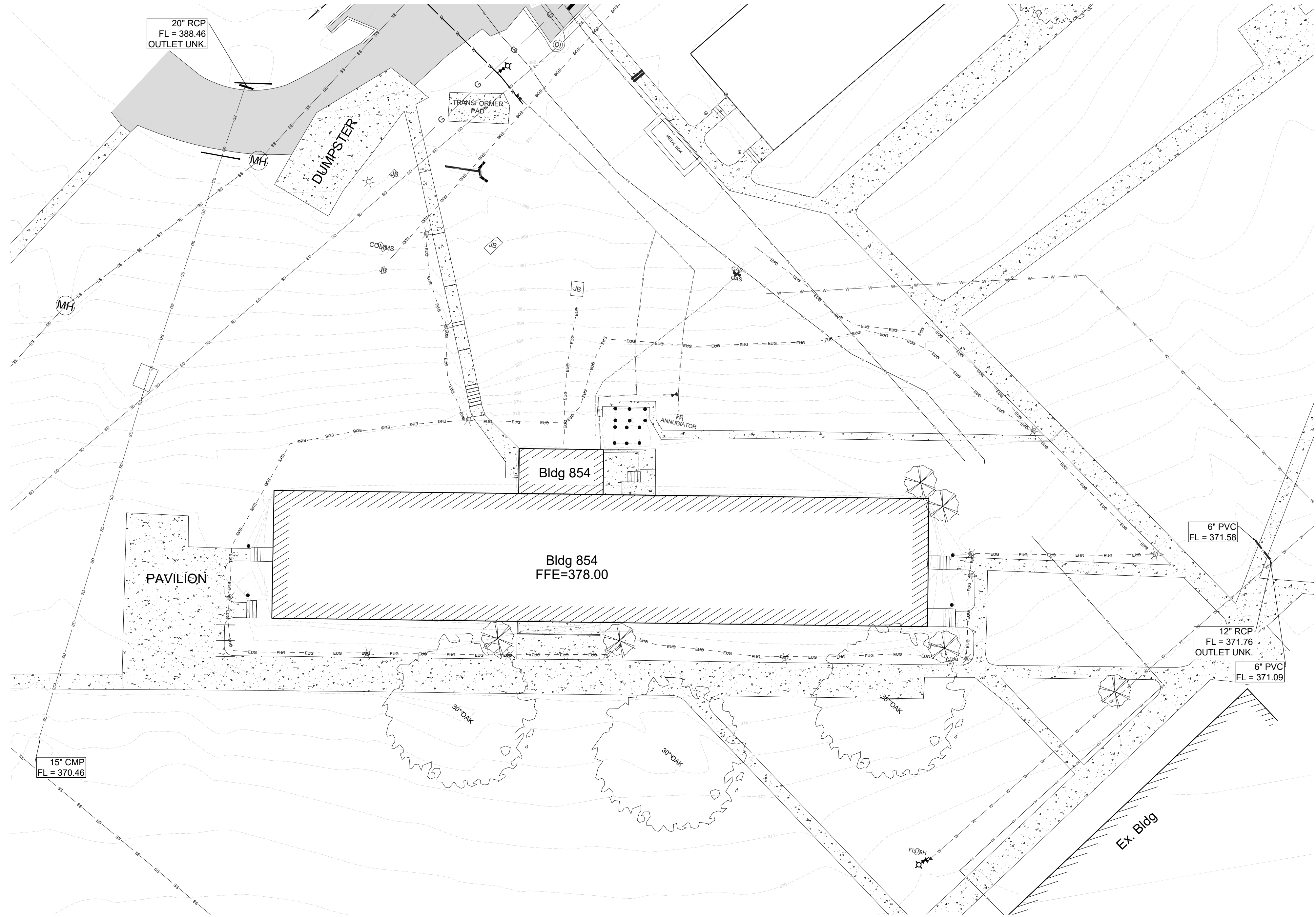
1 EXISTING CONDITIONS SCALE: 1" = 20'
