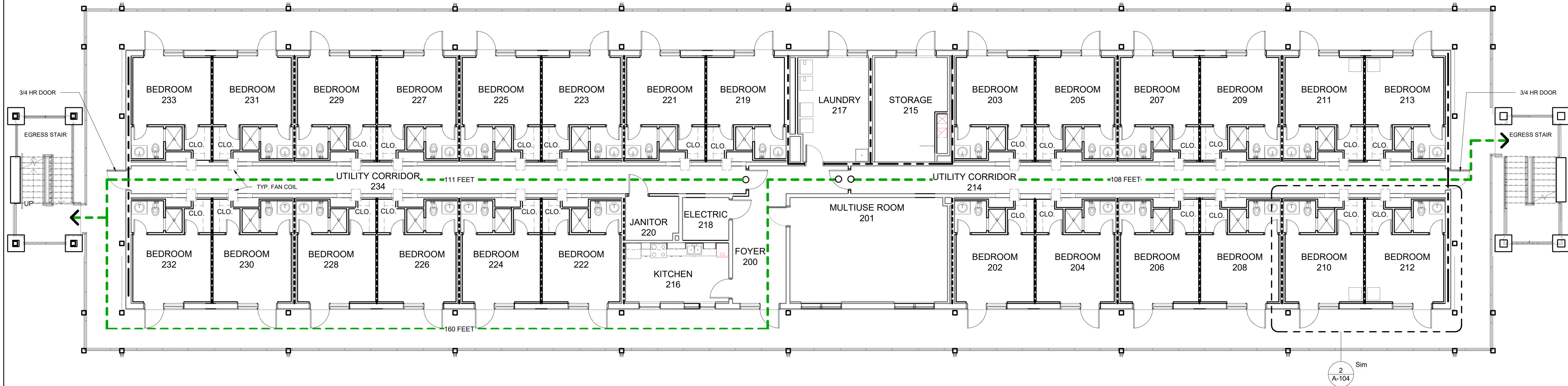
1 SECOND FLOOR-LIFE SAFETY PLAN 1/8" = 1'-0"
