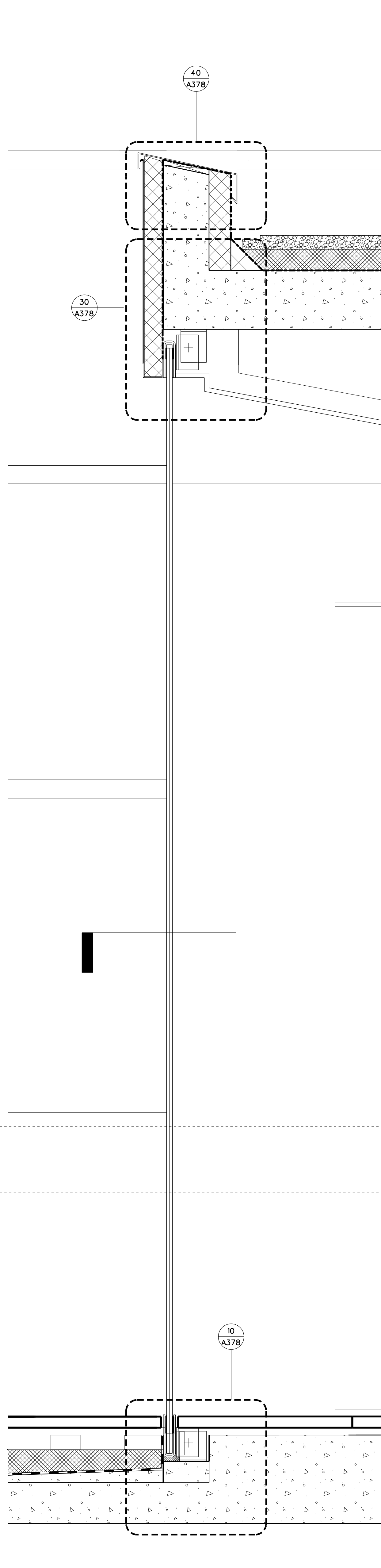
WALL SYSTEM H: TYP DETAIL AT FLOOR AND CORRIDOR ROOF
