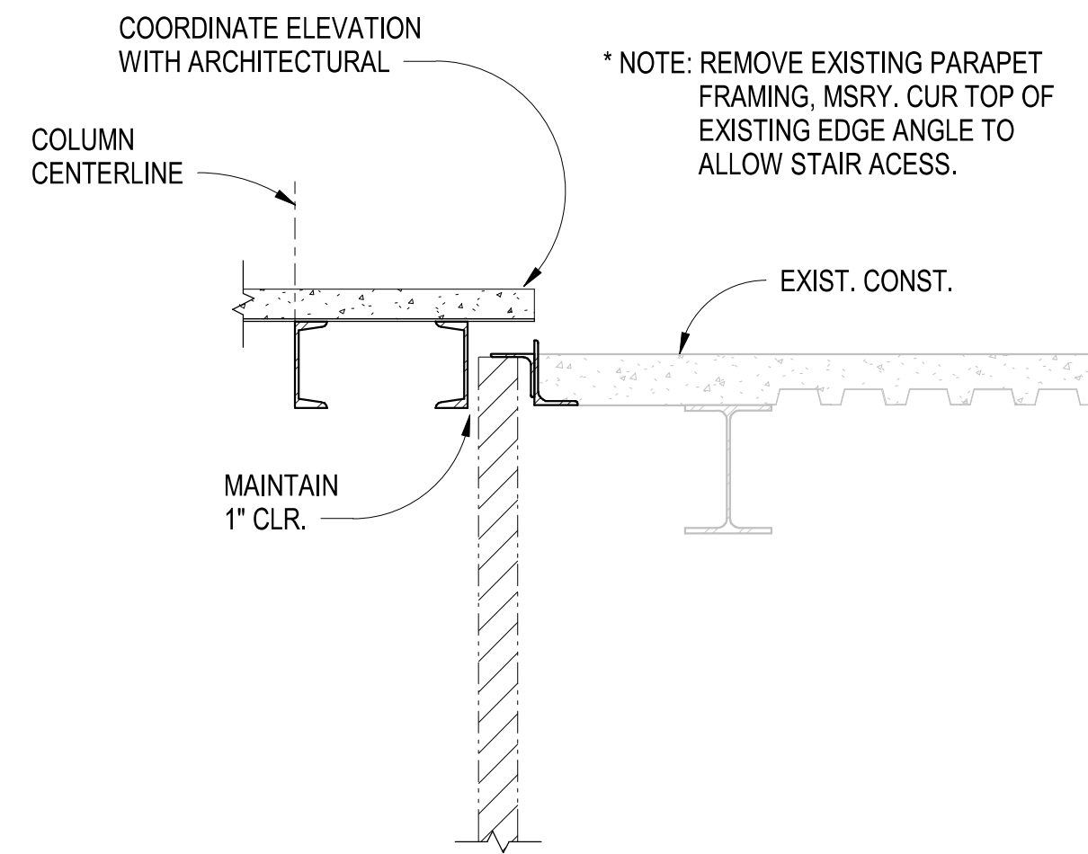
B5 SECTION 3/4" = 1'-0"
