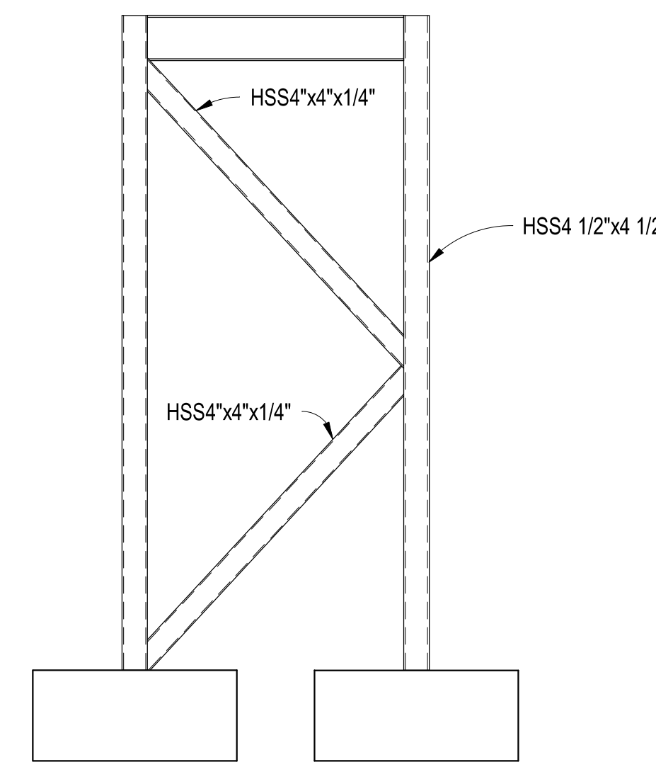
B5 SECTION 3/4" = 1'-0"
