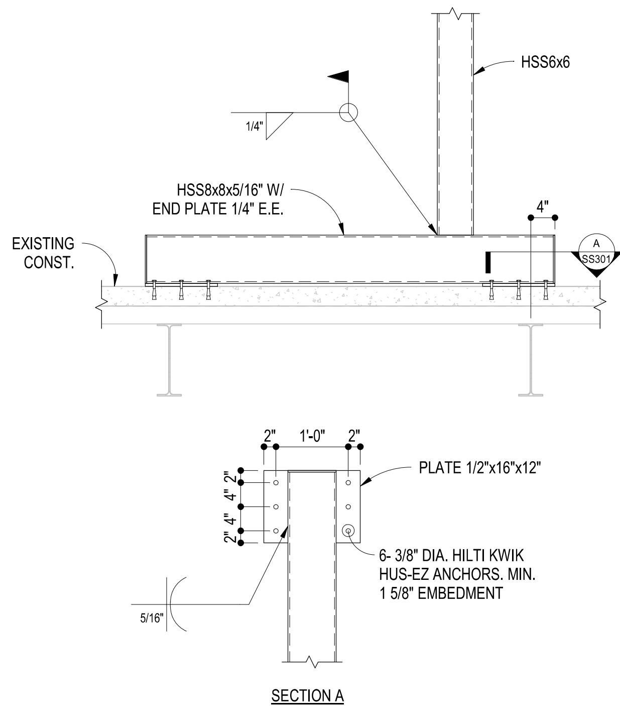
B2 SECTION 3/4" = 1'-0"
