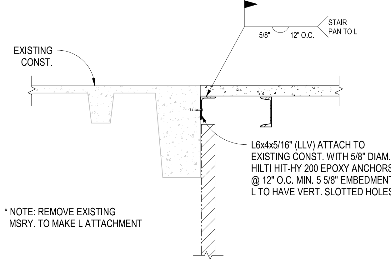
C1 SECTION 3/4" = 1'-0"
