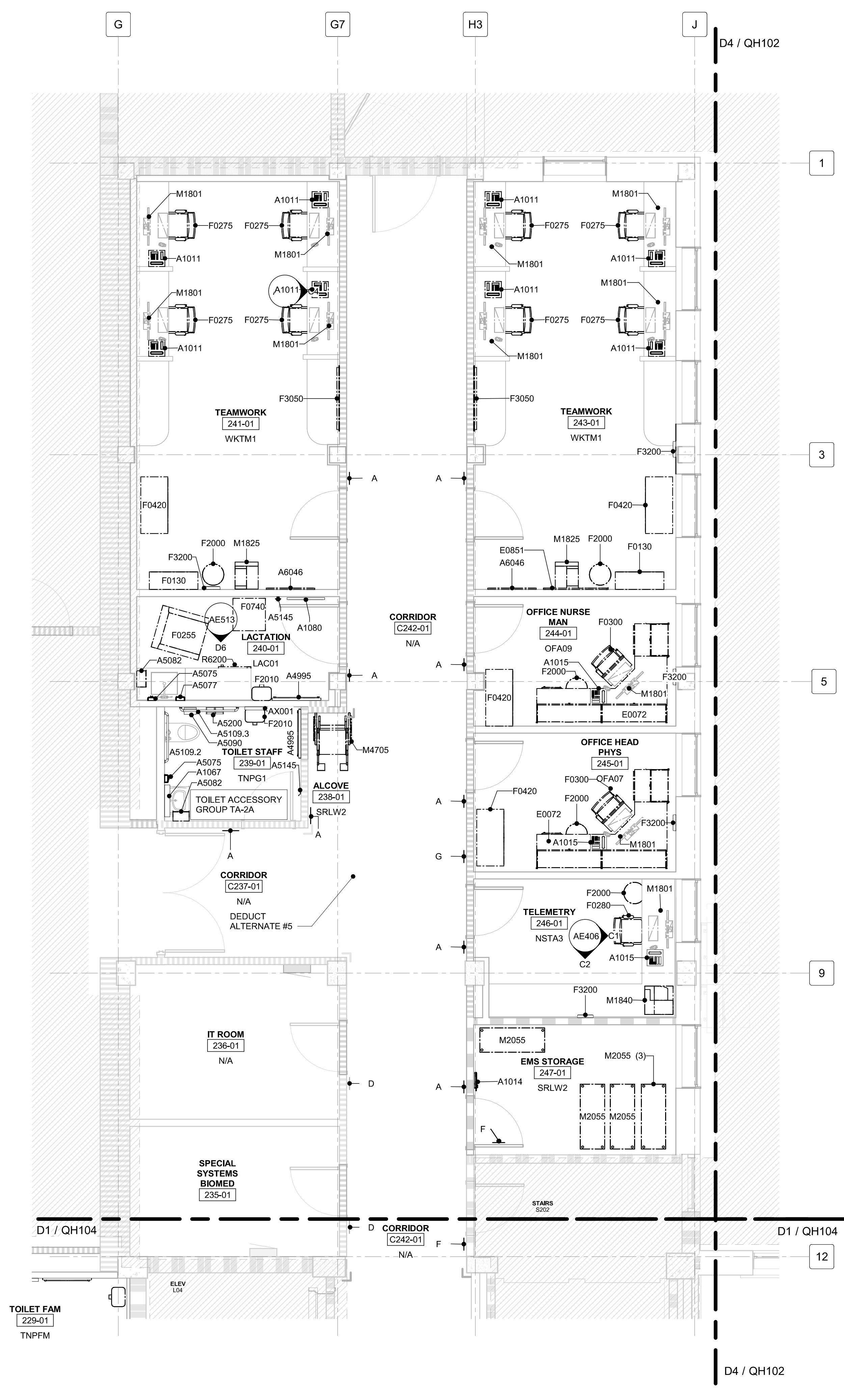
D4 ENLARGED EQUIPMENT PLAN - PHASE 2 - UNIT 2 NORTH 1/4" = 1'-0"
