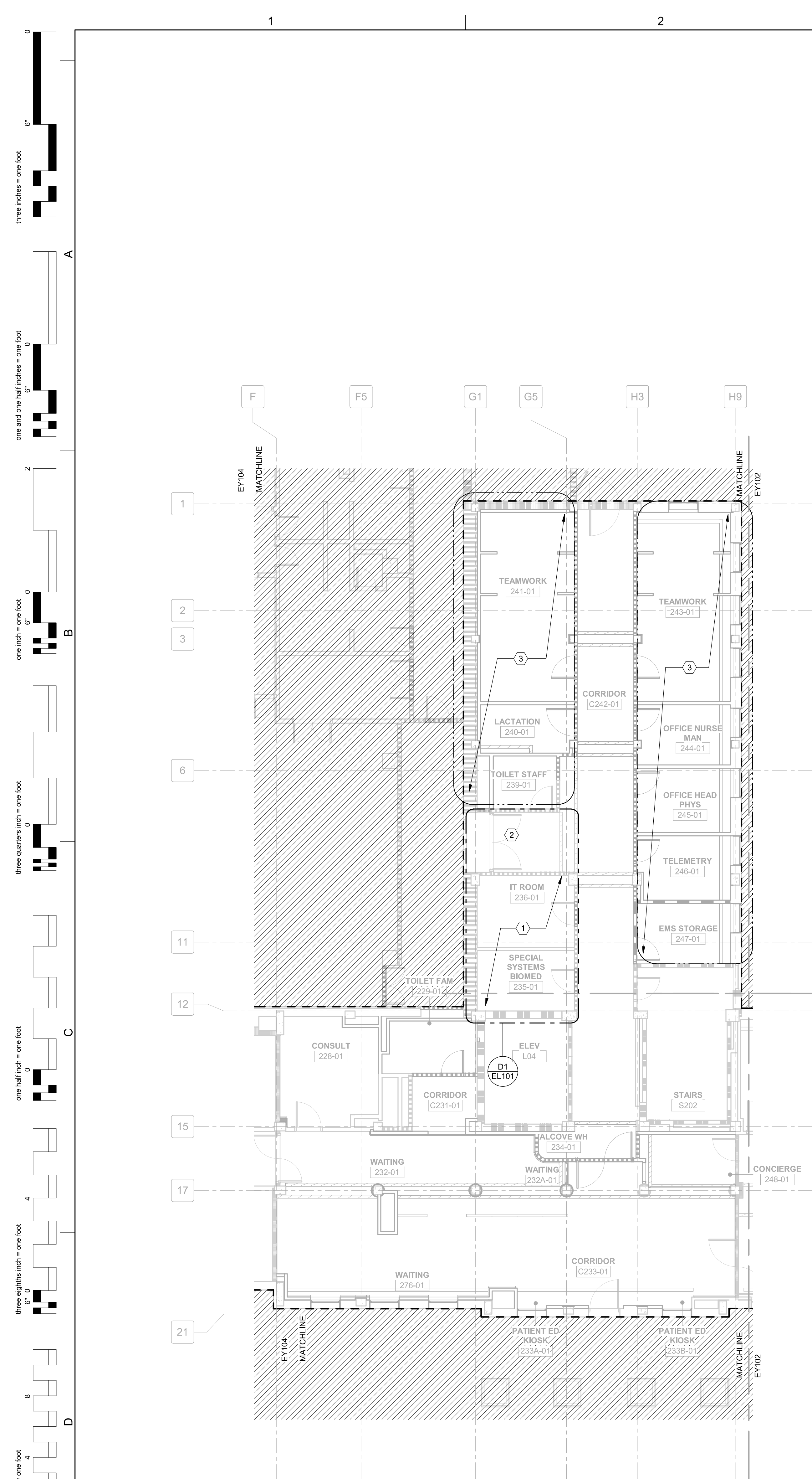
D2 PARTIAL 2 SECOND FLOOR POWER PLAN - PHASE 2 DEDUCT PLAN 1/8" = 1'-0"
