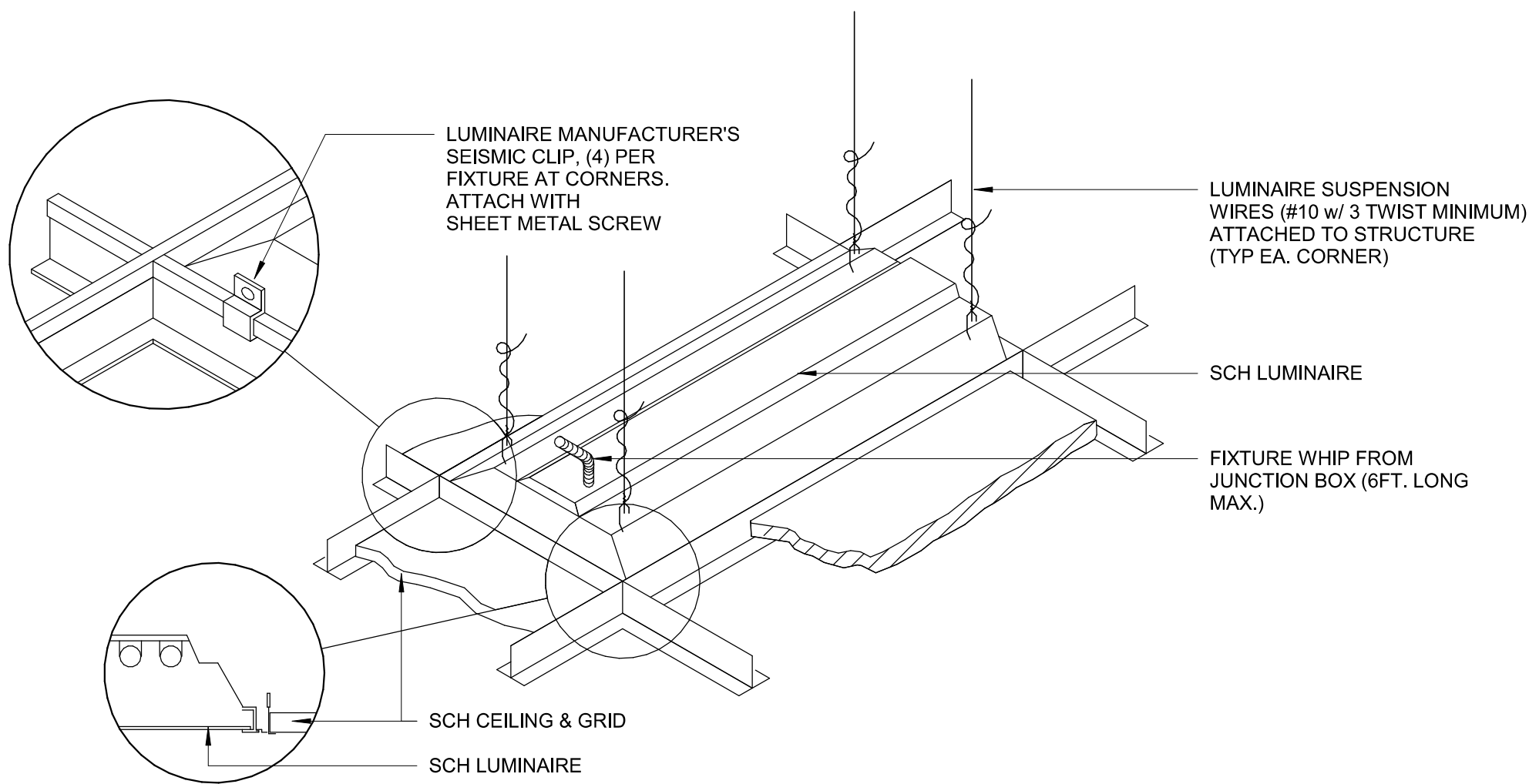
C1 LUMINAIRE MOUNTING - LAY-IN CEILING NO SCALE
