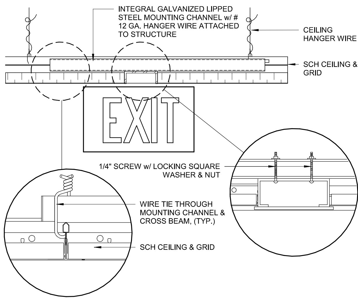
D1 EXIT SIGN MOUNTING - LAY-IN CEILING NO SCALE
