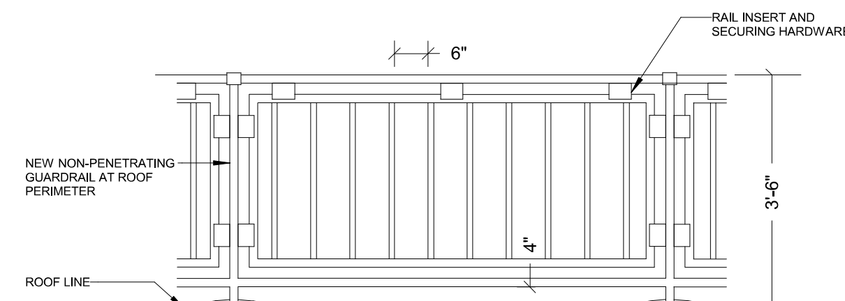
NON-PENETRATING GUARDRAIL ELEVATION, TYPICAL A5 1/2" = 1'-0"
