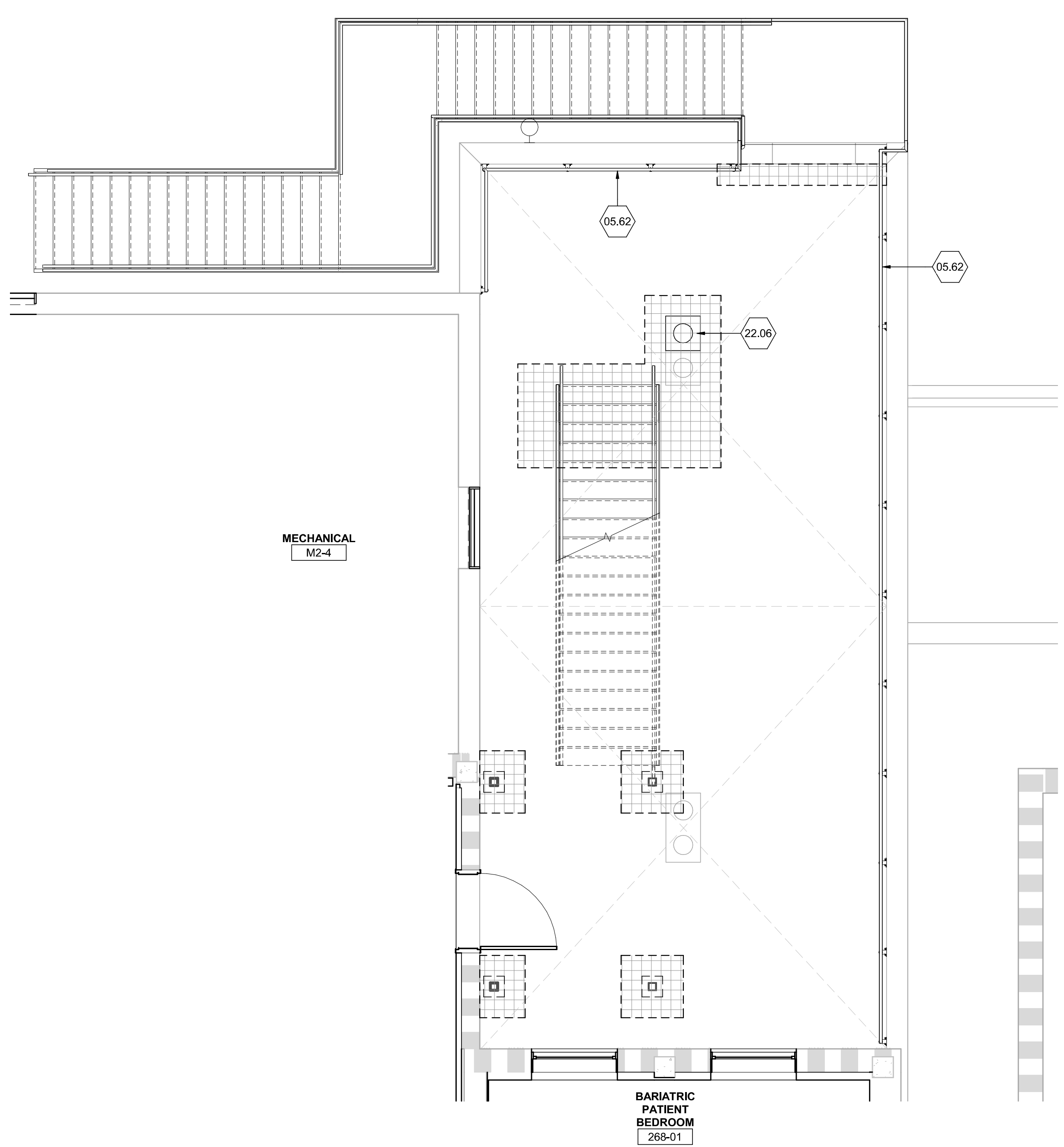
D5 RE-ROOF PLAN - EXTERIOR STAIR EAST SECOND FLOOR 1/4" = 1'-0"
