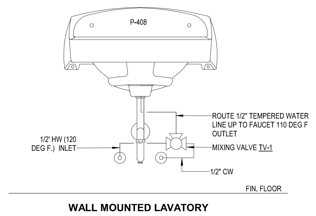
F4 MIXING VALVE FOR LAVATORIES NOT TO SCALE
