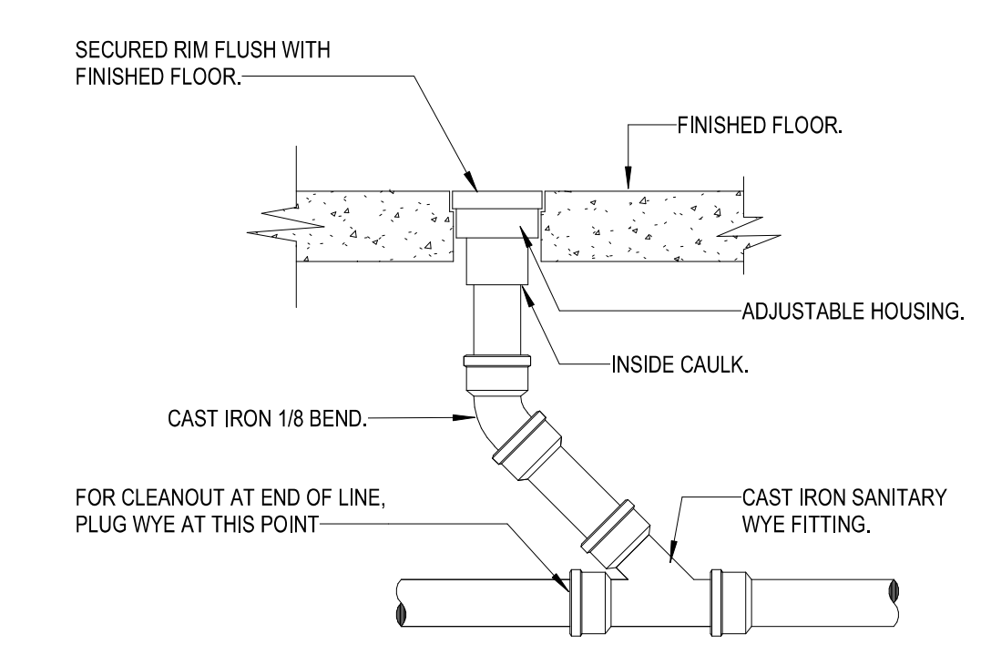
F7 FLOOR CLEANOUT DETAIL NOT TO SCALE
