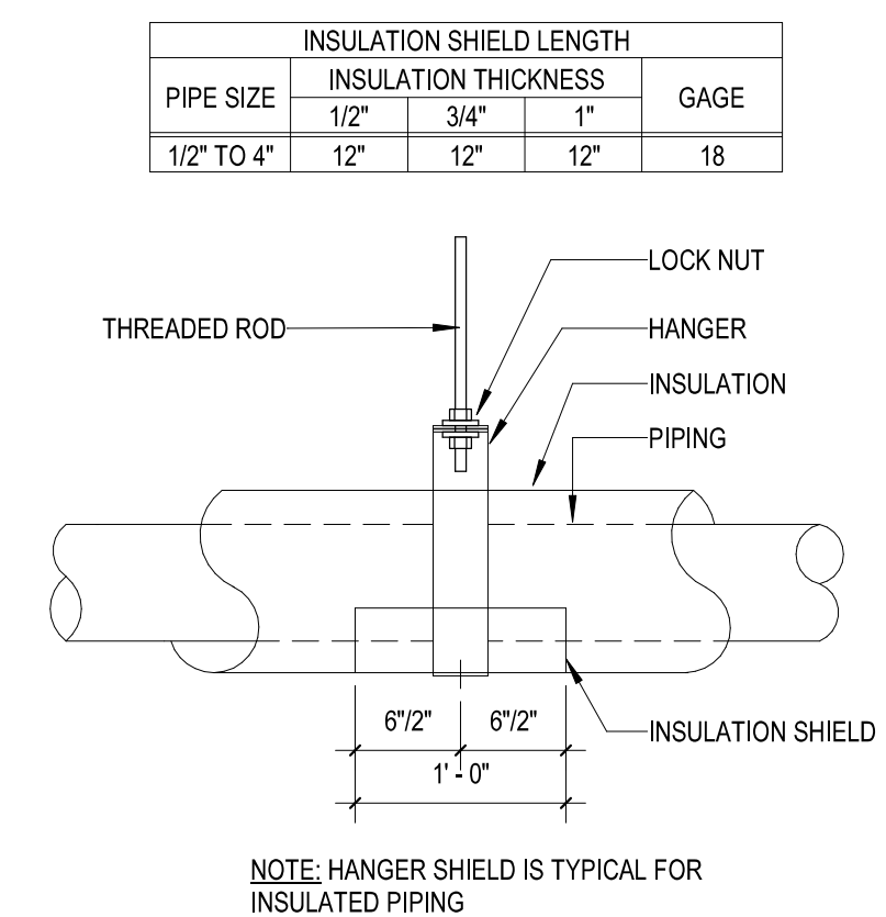
D4 INSULATION SHIELD DETAIL NOT TO SCALE
