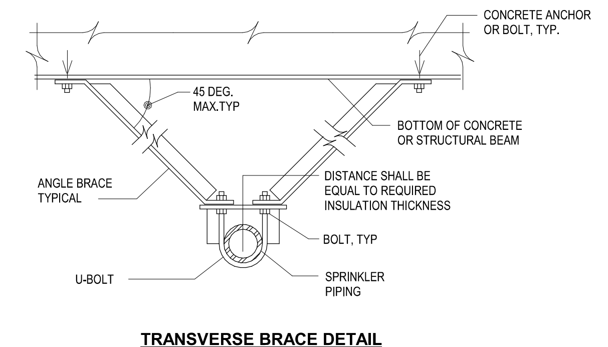
TRANSVERSE BRACE DETAIL
