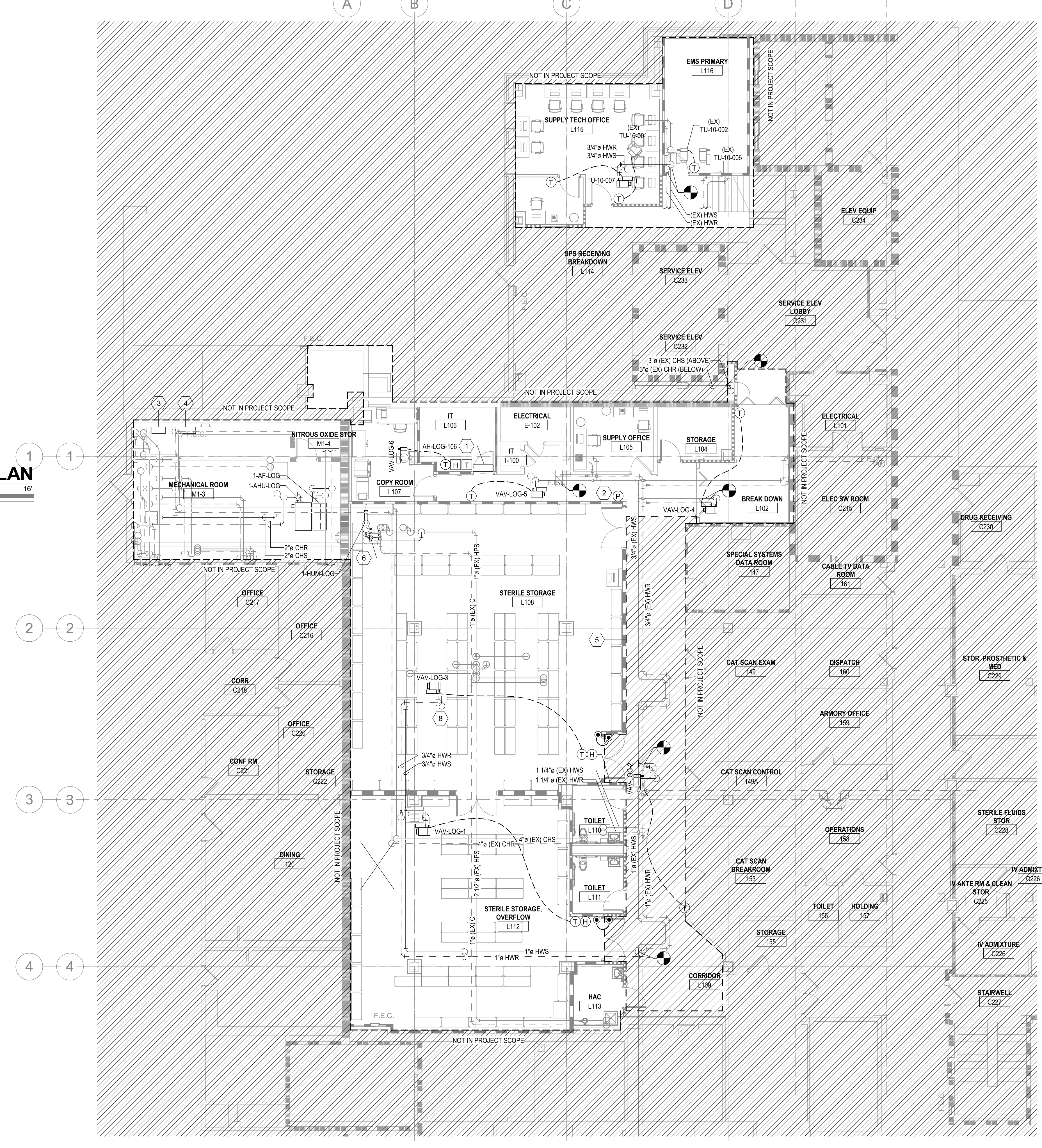
F4 FIRST FLOOR MECHANICAL PIPING PLAN 1/8" = 1'-0"
