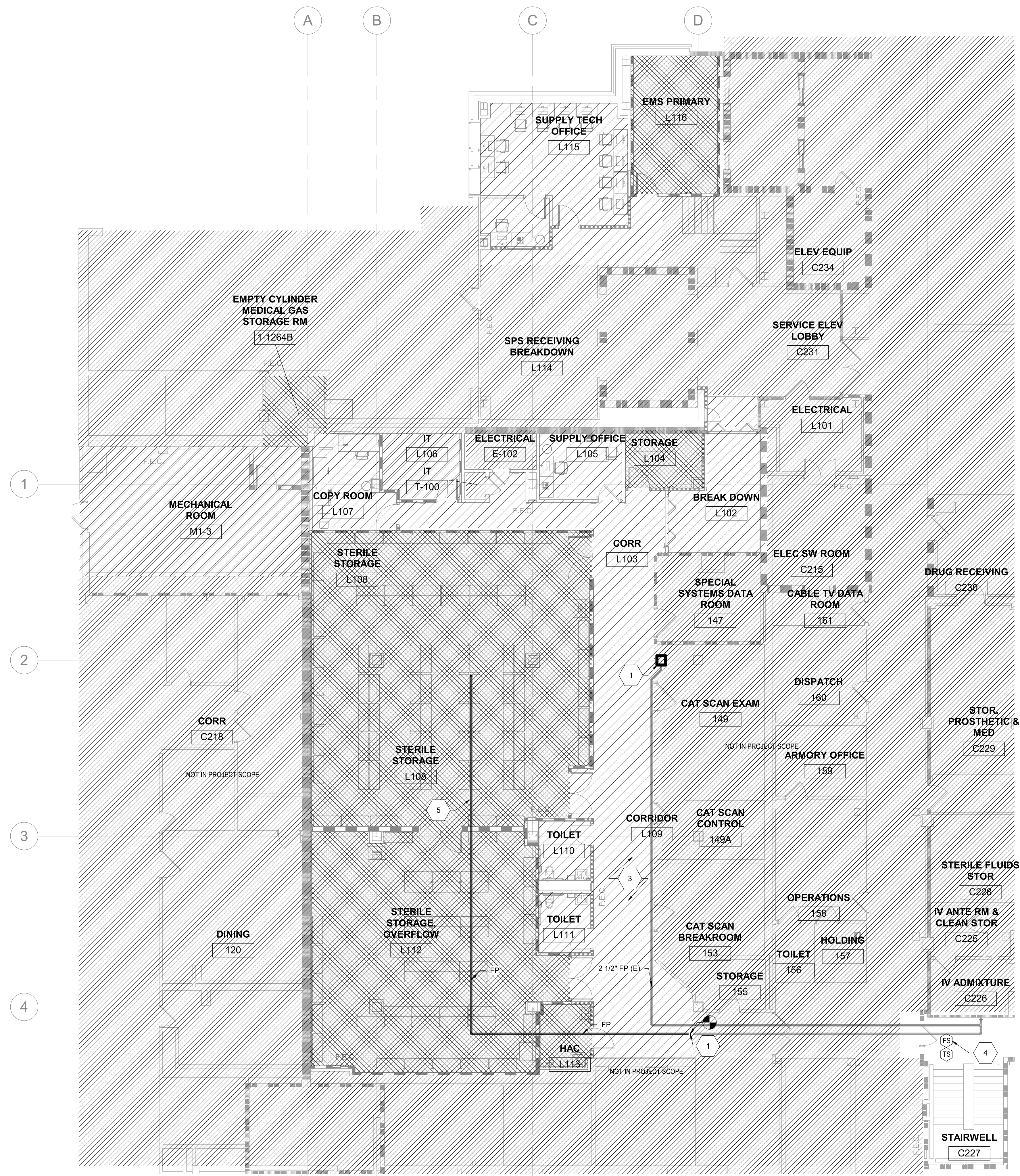
F4 FIRST FLOOR FIRE PROTECTION PLAN 1/8" = 1'-0"
