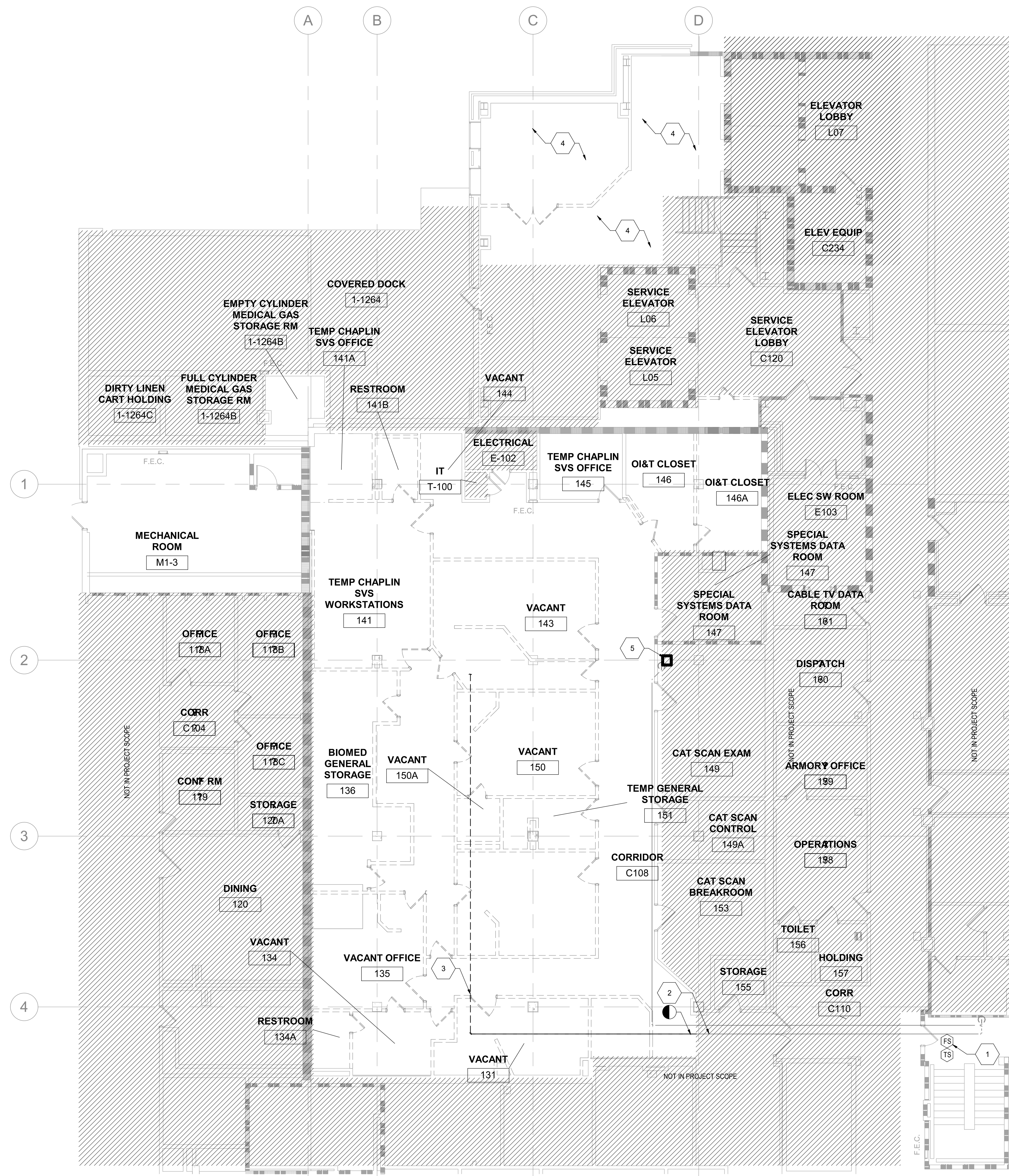
F4 FIRST FLOOR FIRE PROTECTION DEMOLITION PLAN 1/8" = 1'-0"
