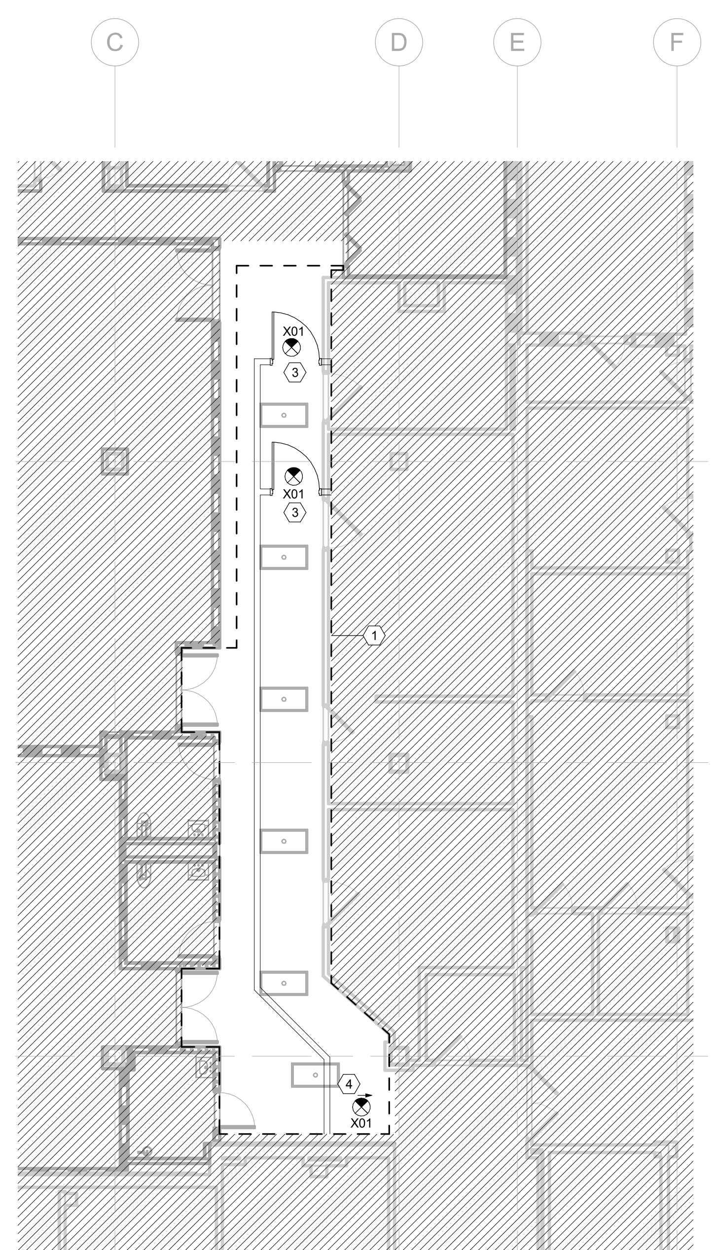
C2 FIRST FLOOR - LIGHTING PLAN - TEMPORARY 1/8" = 1'-0"
