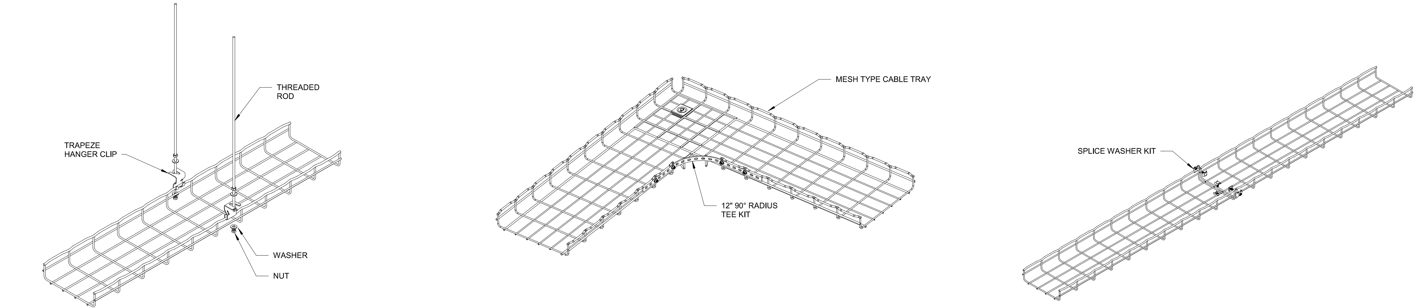
A4 CABLE TRAY DETAILS - A NO SCALE
