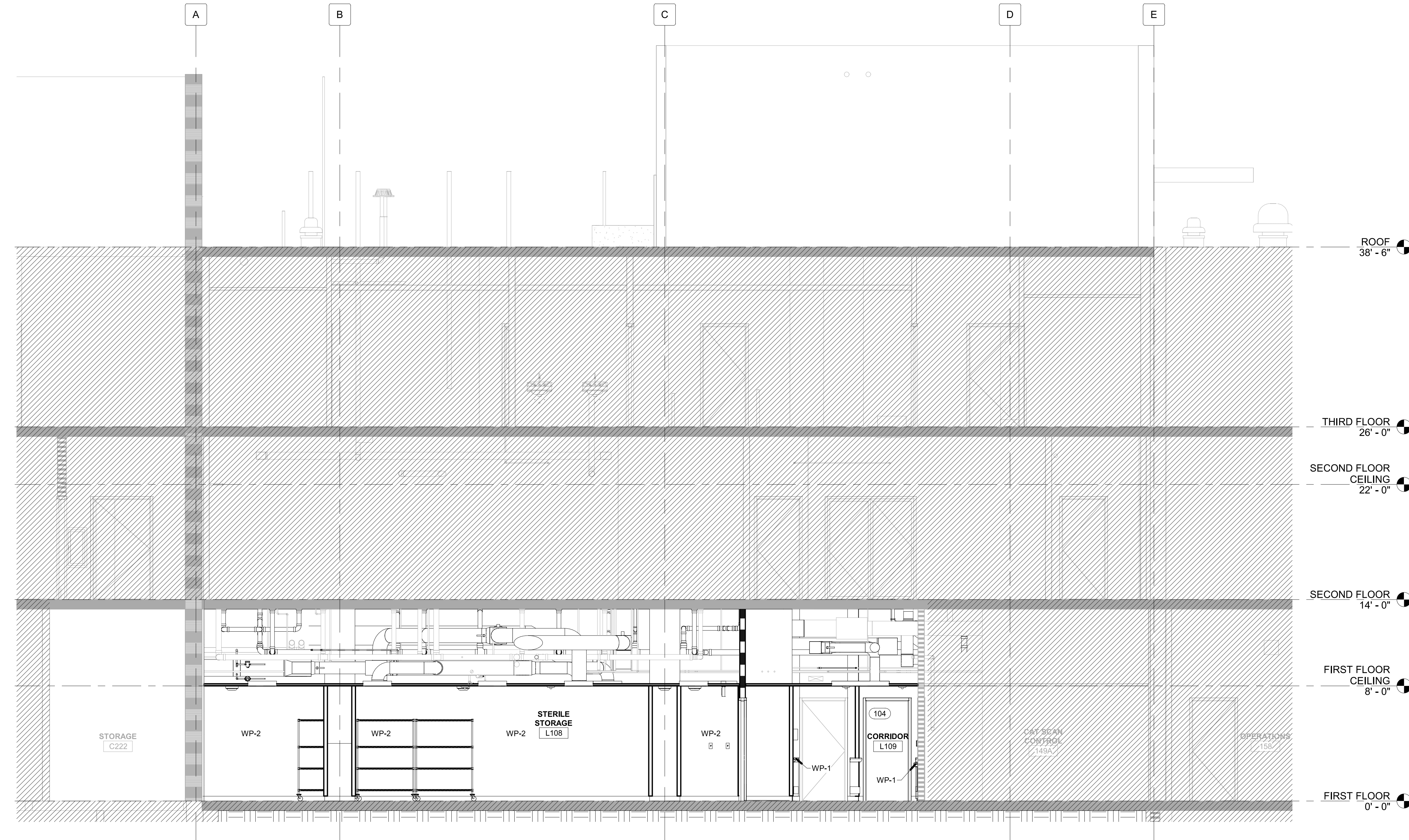
E3 BUILDING SECTION - OVERALL 02 1/4" = 1'-0"
