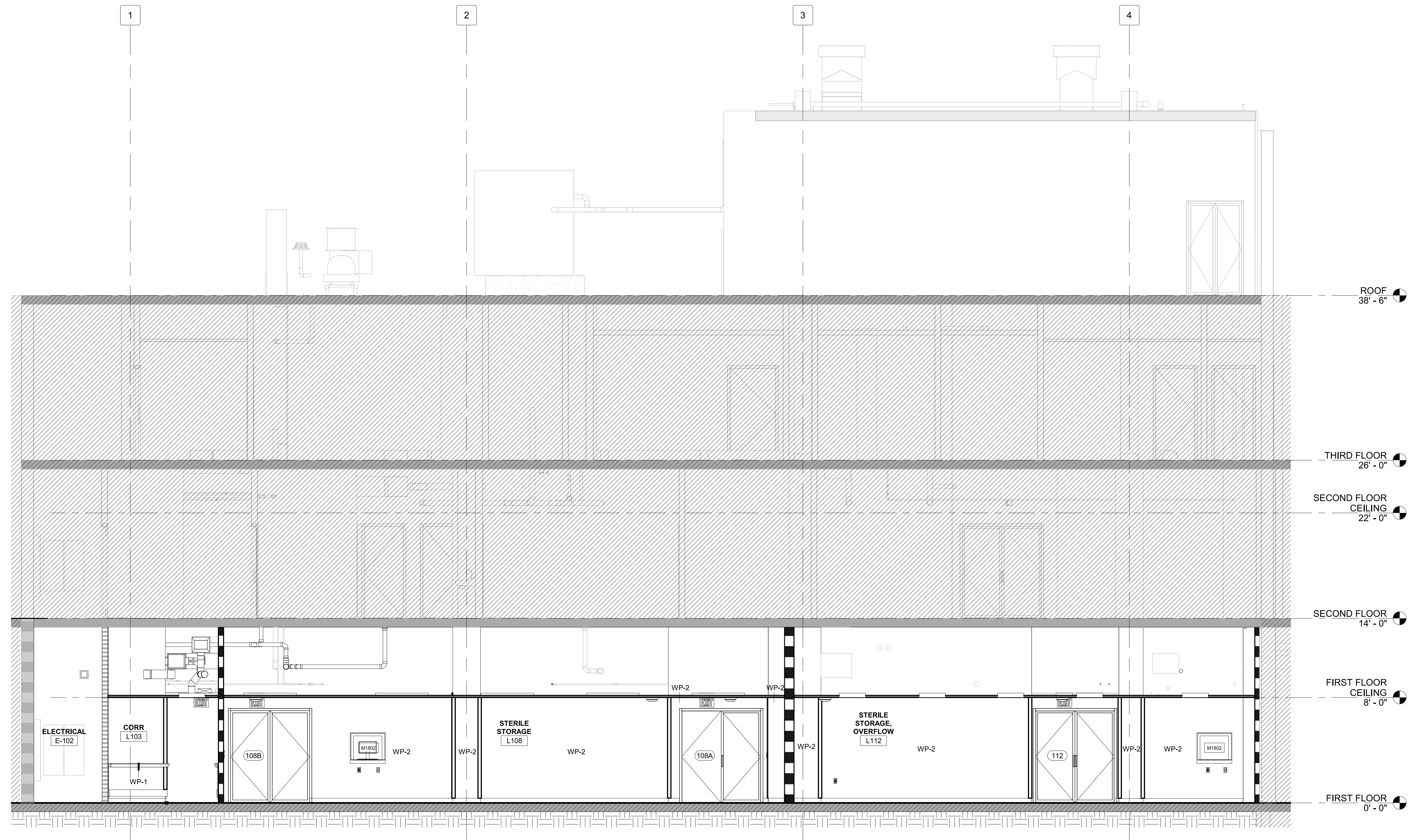
E3 BUILDING SECTION - OVERALL 01 1/4" = 1'-0"
