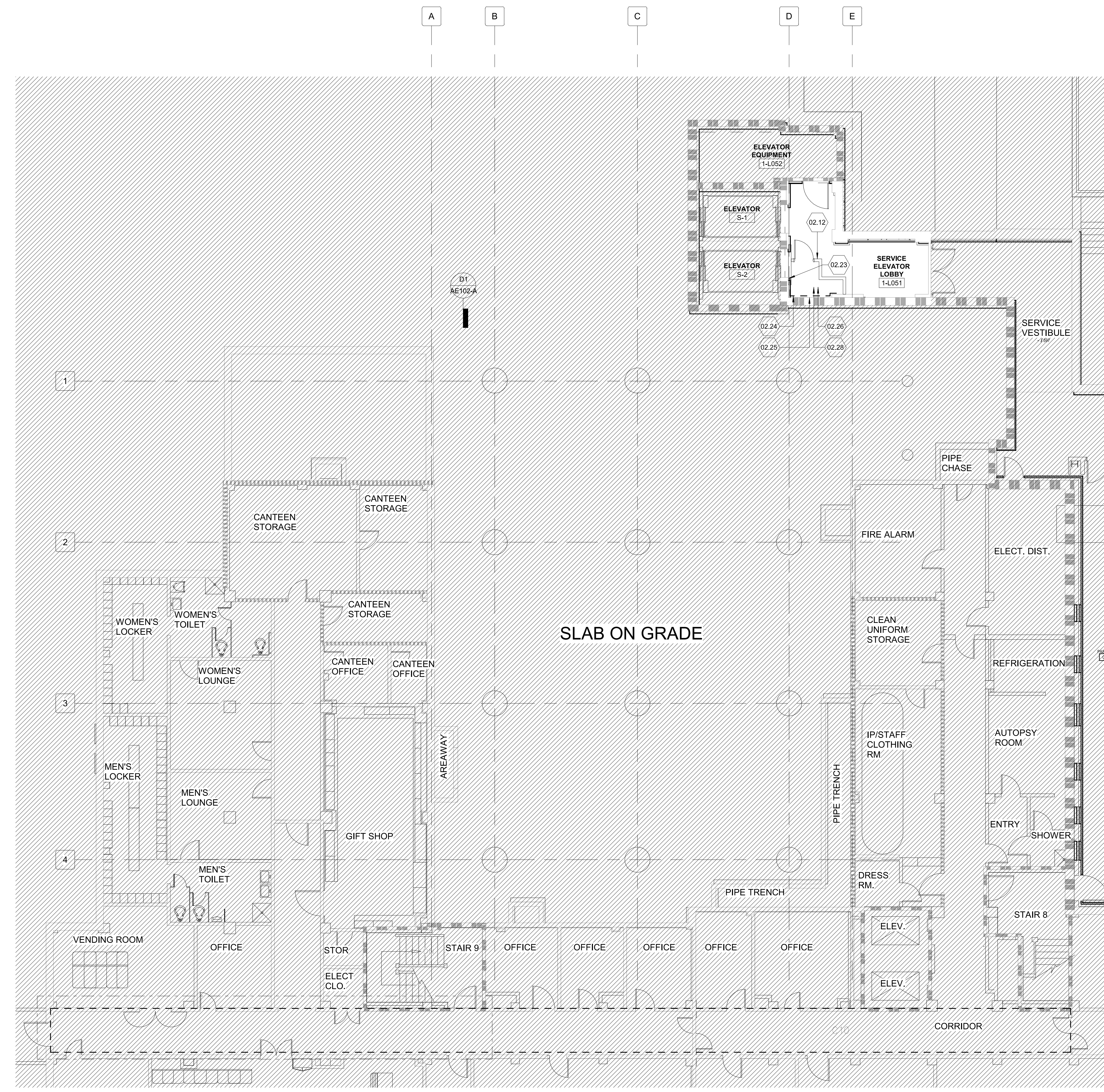
F5 BASEMENT FLOOR - DEMOLITION PLAN 1/8" = 1'-0"
