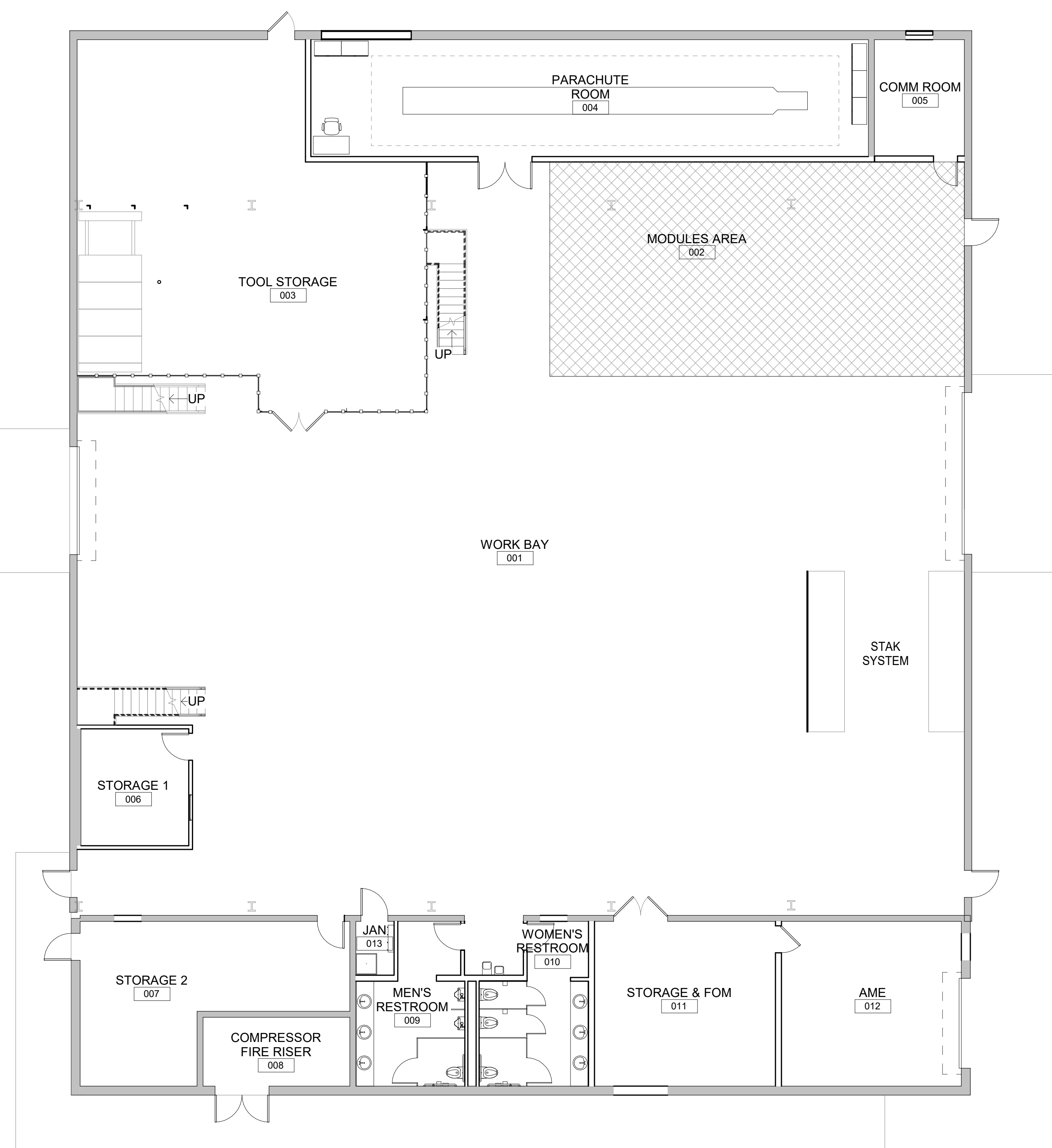
A1 GROUND FLOOR FURNITURE PLAN 1/8" = 1'-0" PLAN NORTH 0 4' 8' 16'
