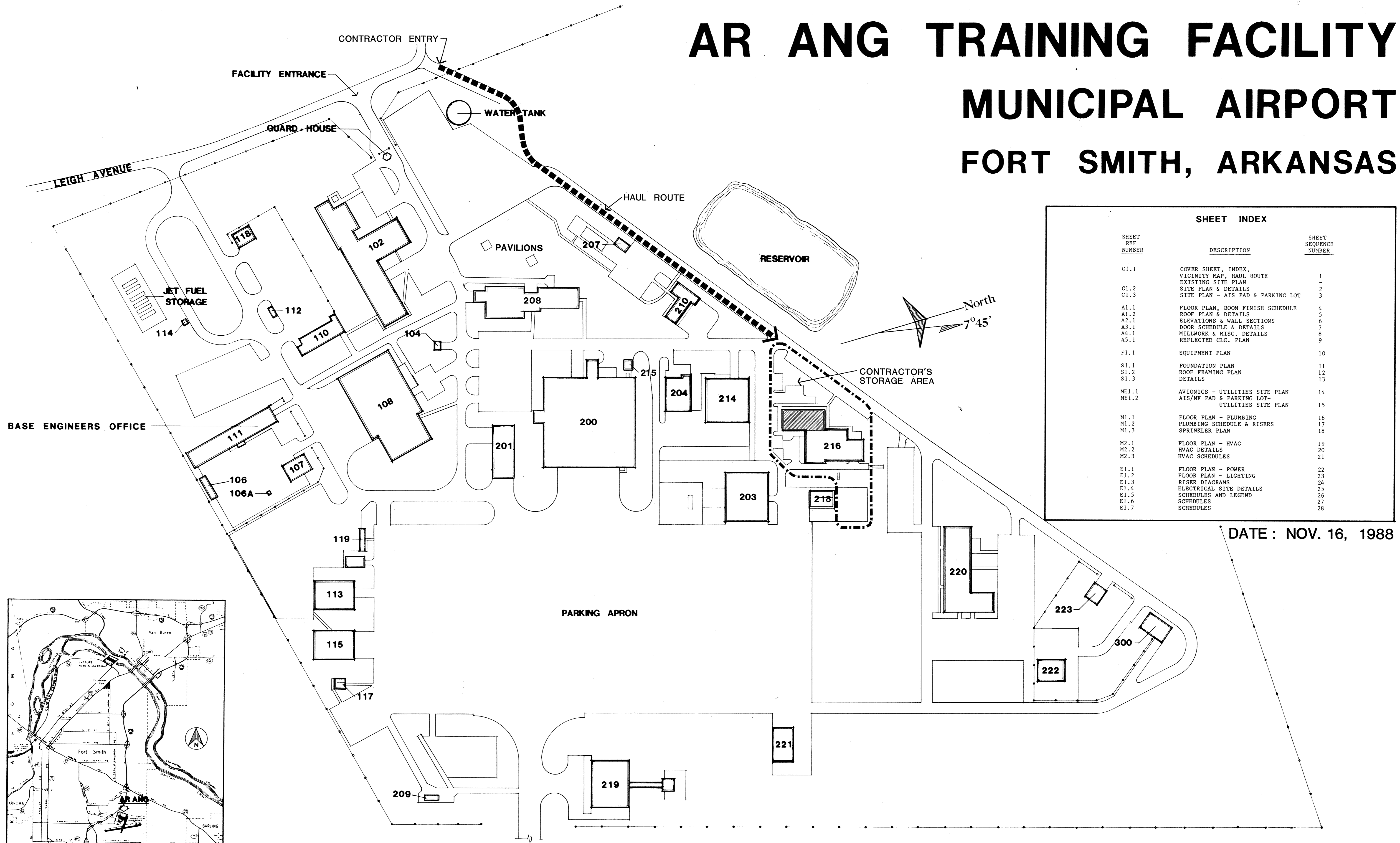
SITE PLAN 1" = 100'
