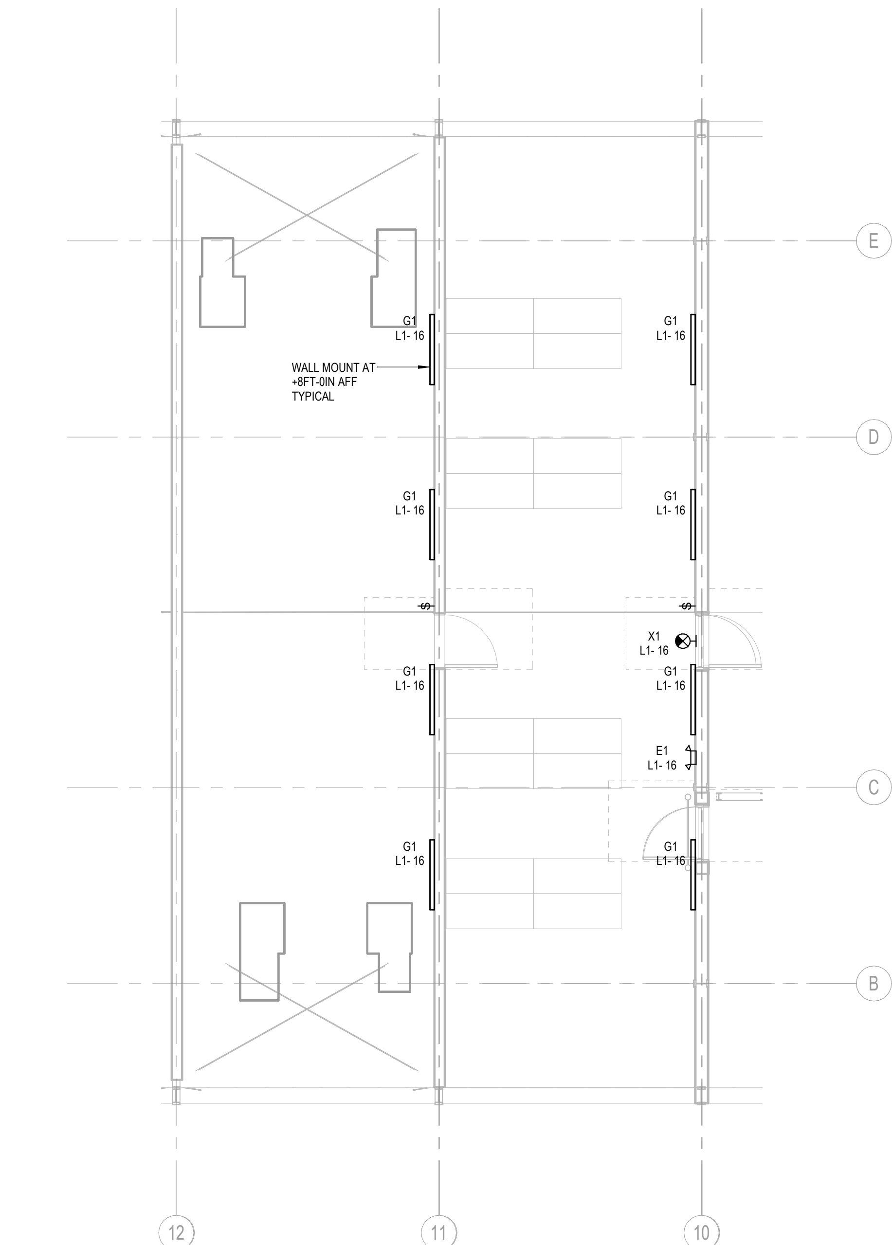
2 LIGHTING PLAN - EQUIPMENT PLATFORM 3/16" = 1'-0"
