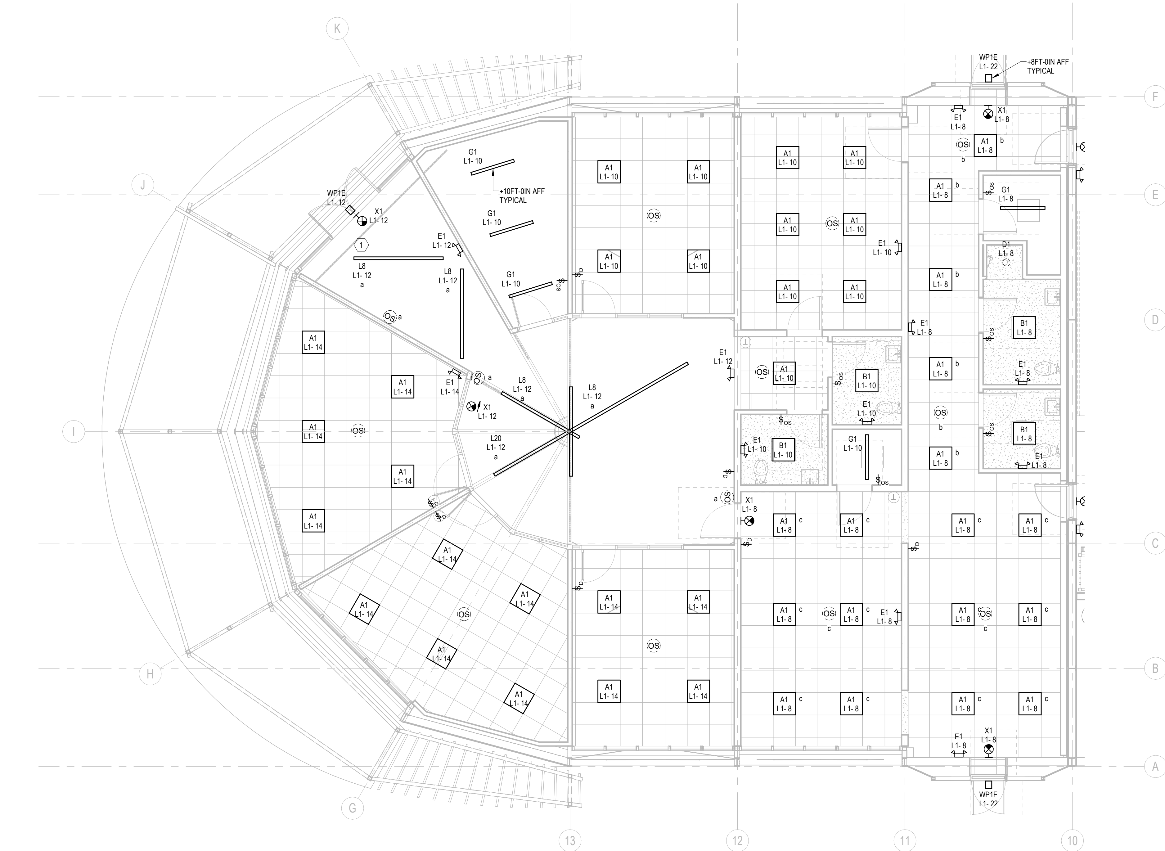
1 LIGHTING PLAN - ENLARGED OFFICE 3/16" = 1'-0"
