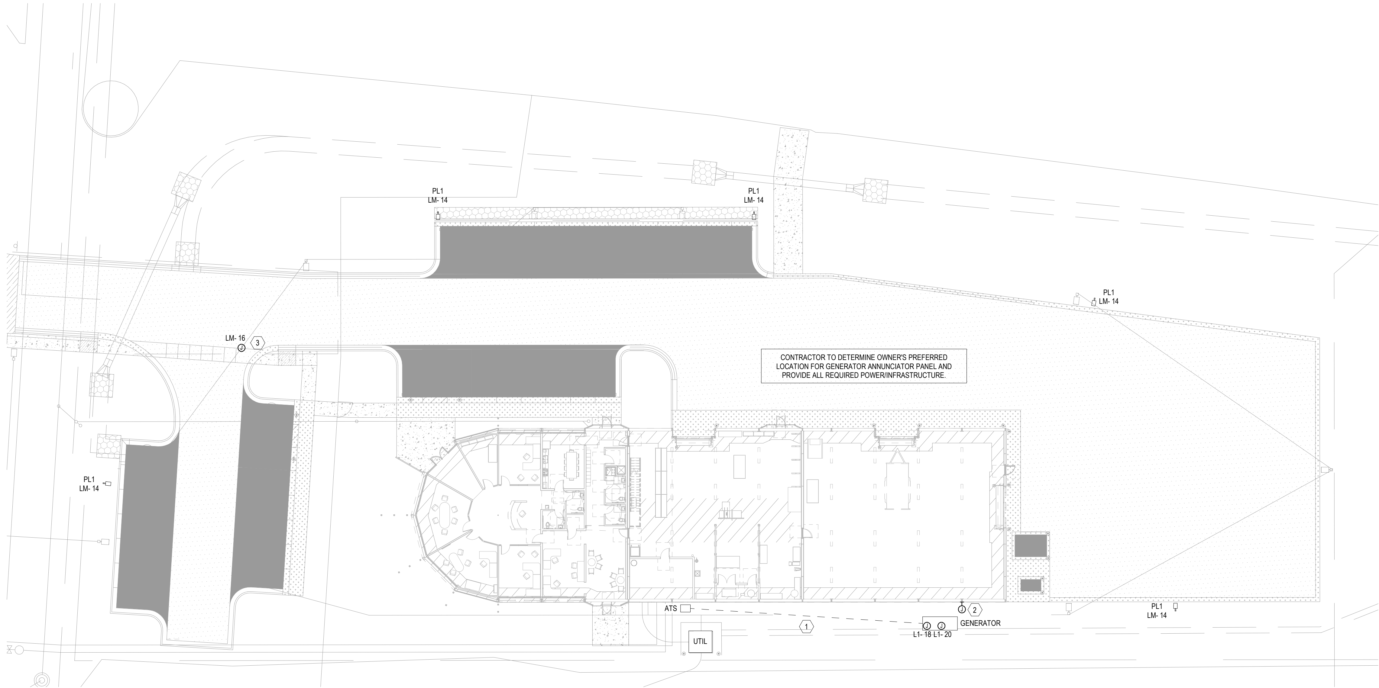
1 ELECTRICAL PLAN - SITE 1" = 20'-0"
