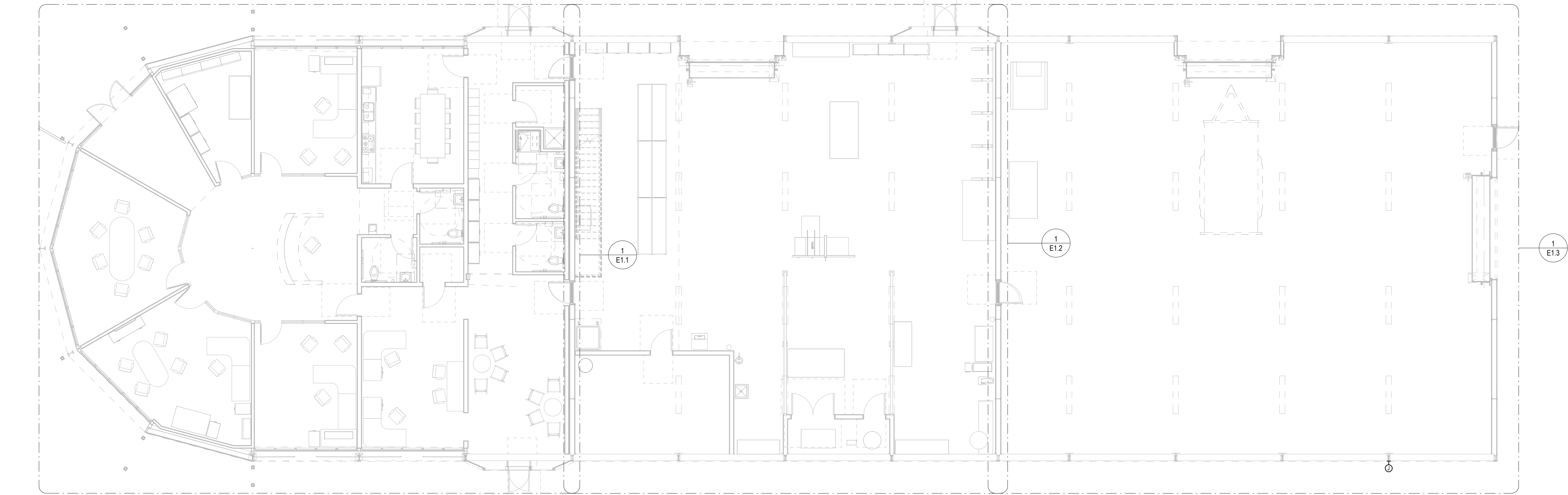
1 POWER PLAN - OVERALL 1/8" = 1'-0"
