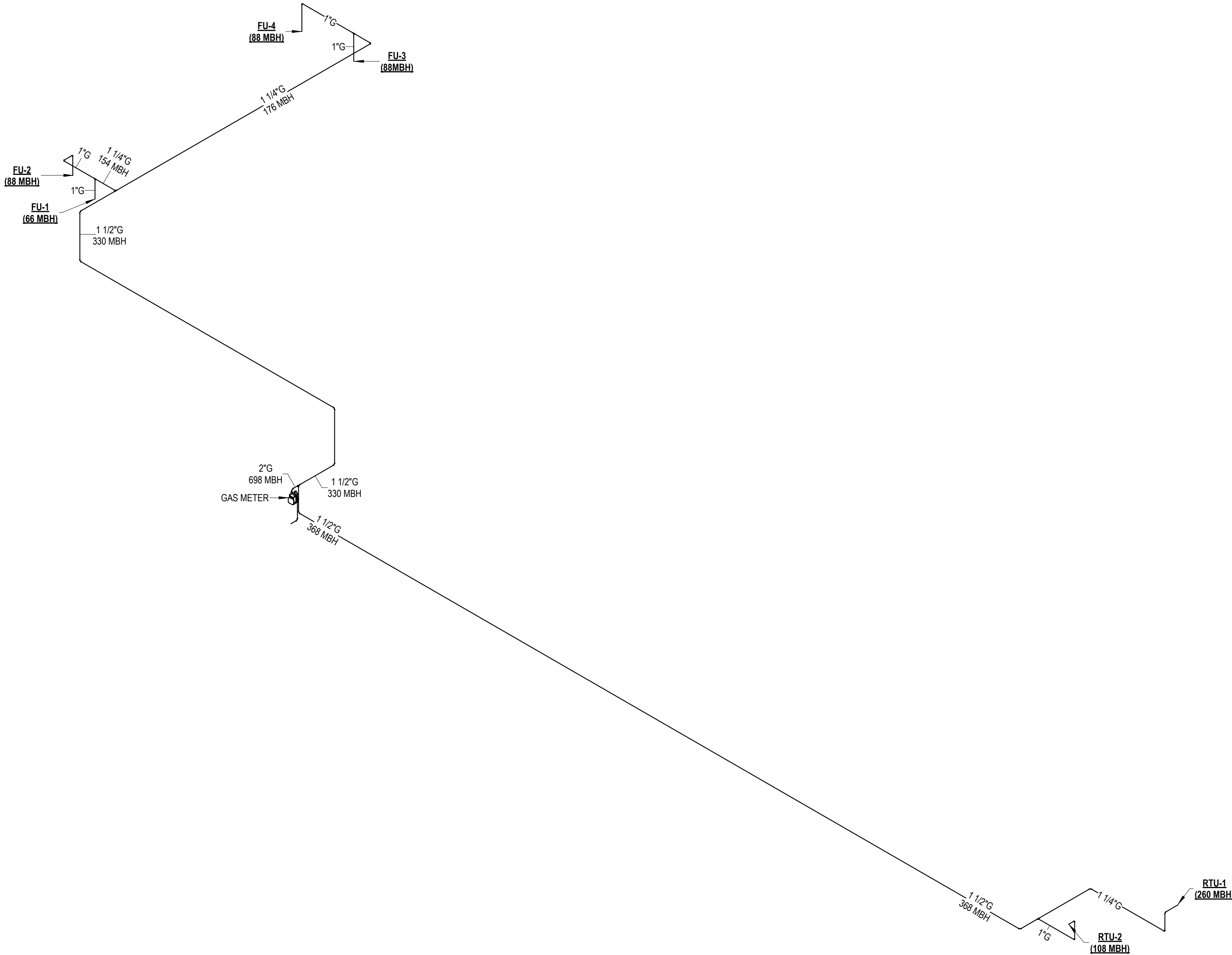
1 GAS ISOMETRIC
