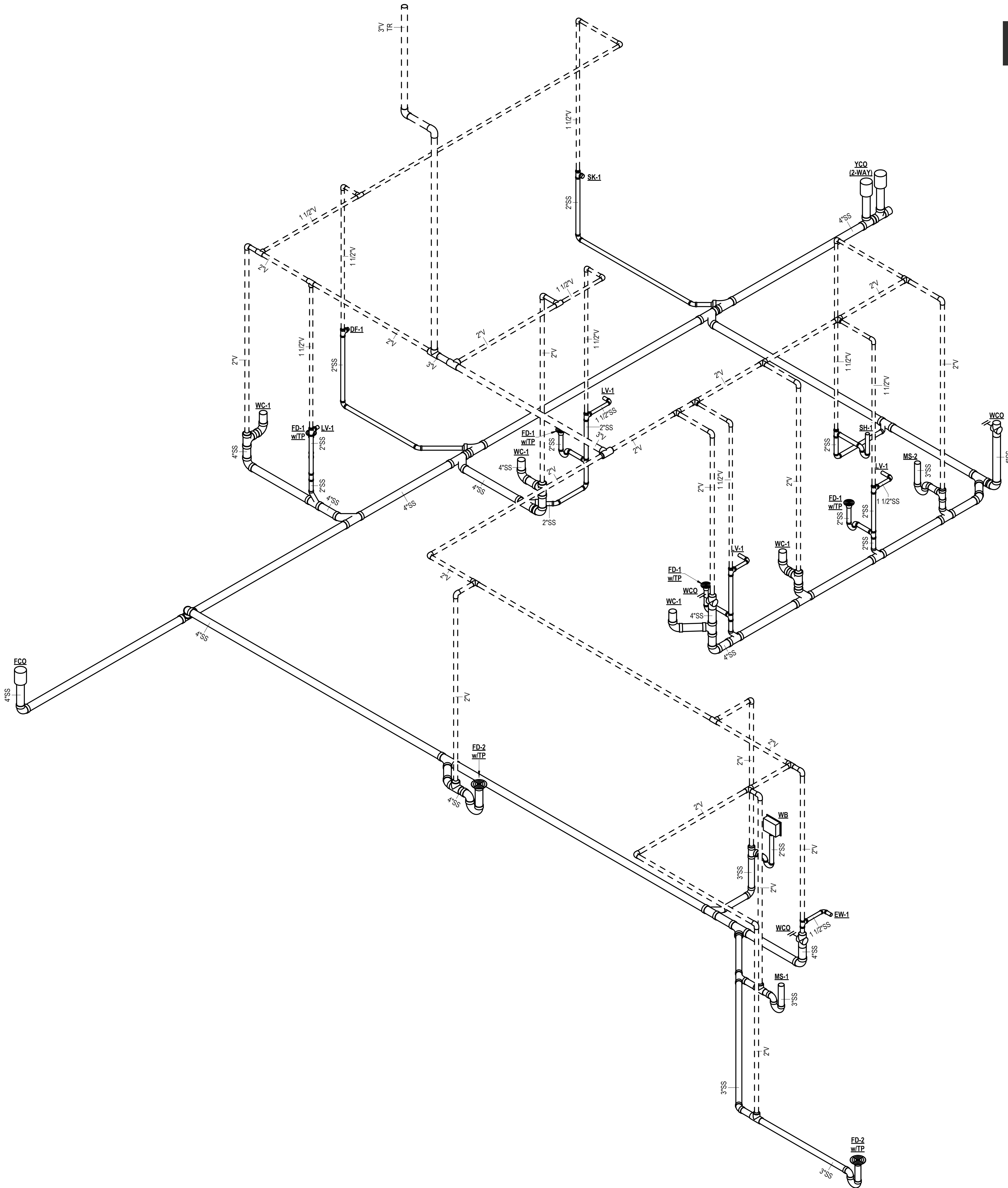
1 DWV ISOMETRIC
