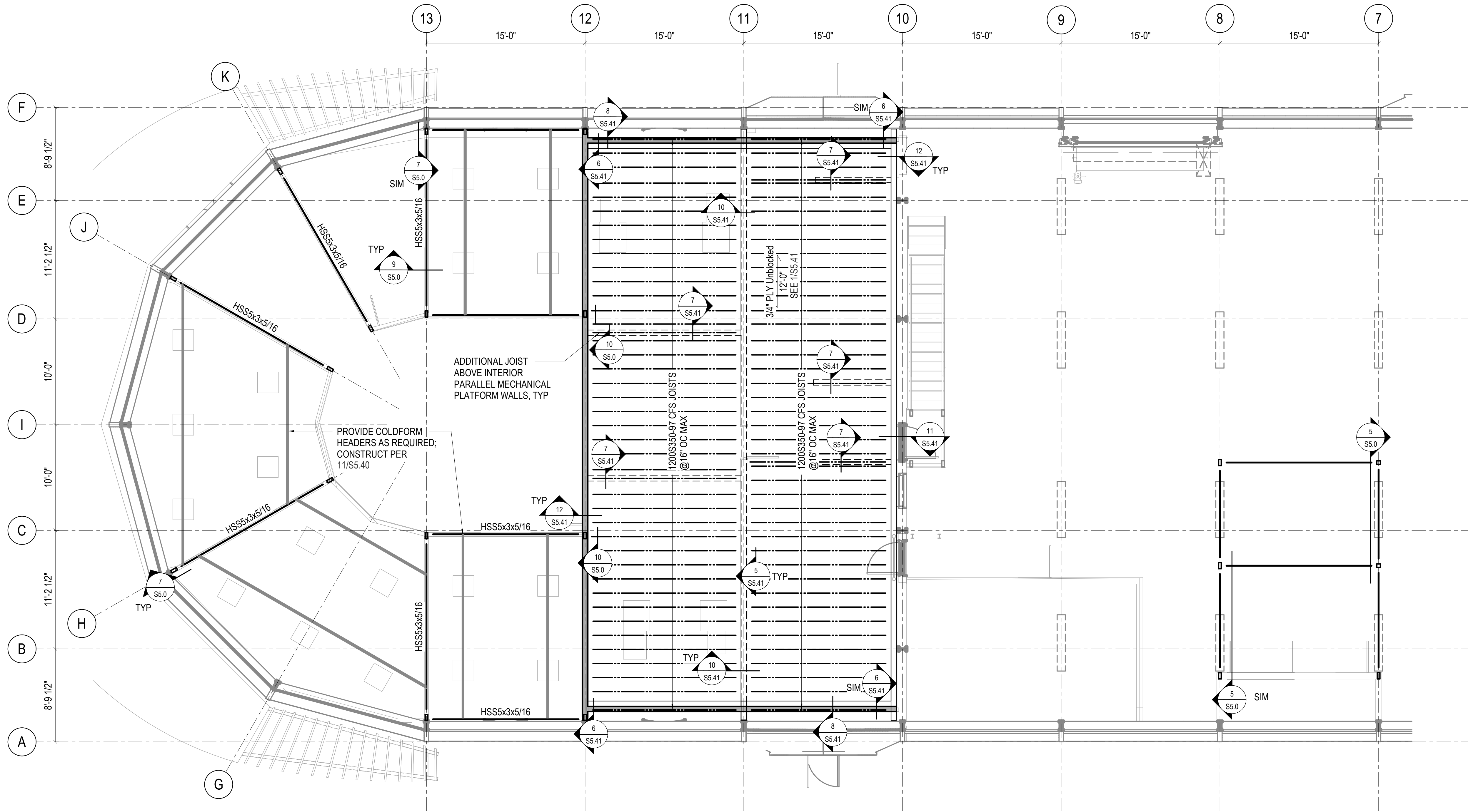
1 EQUIPMENT PLATFORM FRAMING PLAN 3/16" = 1'-0"
