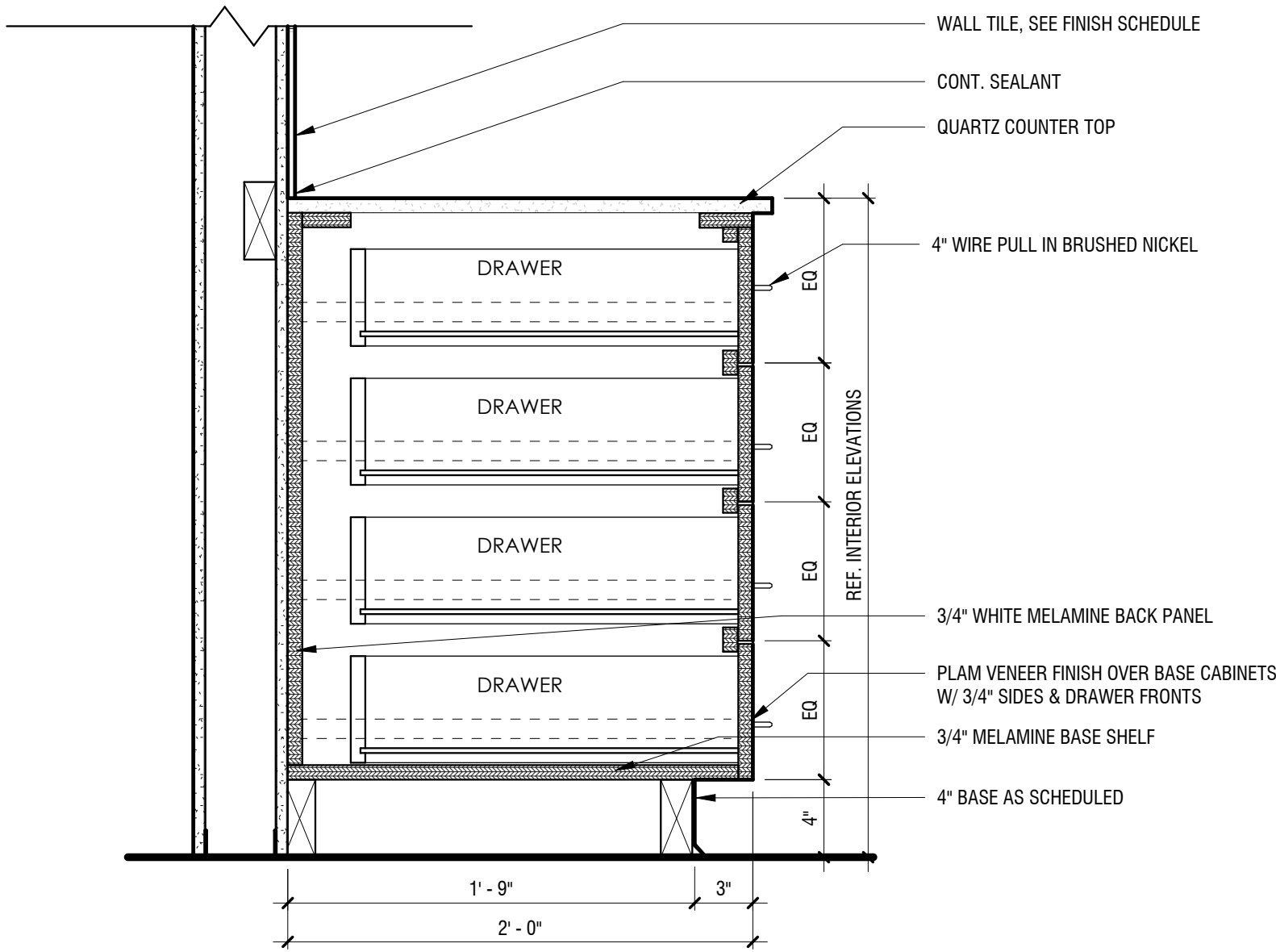
1 BASE CABINET W/ 4 DRAWERS A4.2 1 1/2" = 1'-0"
