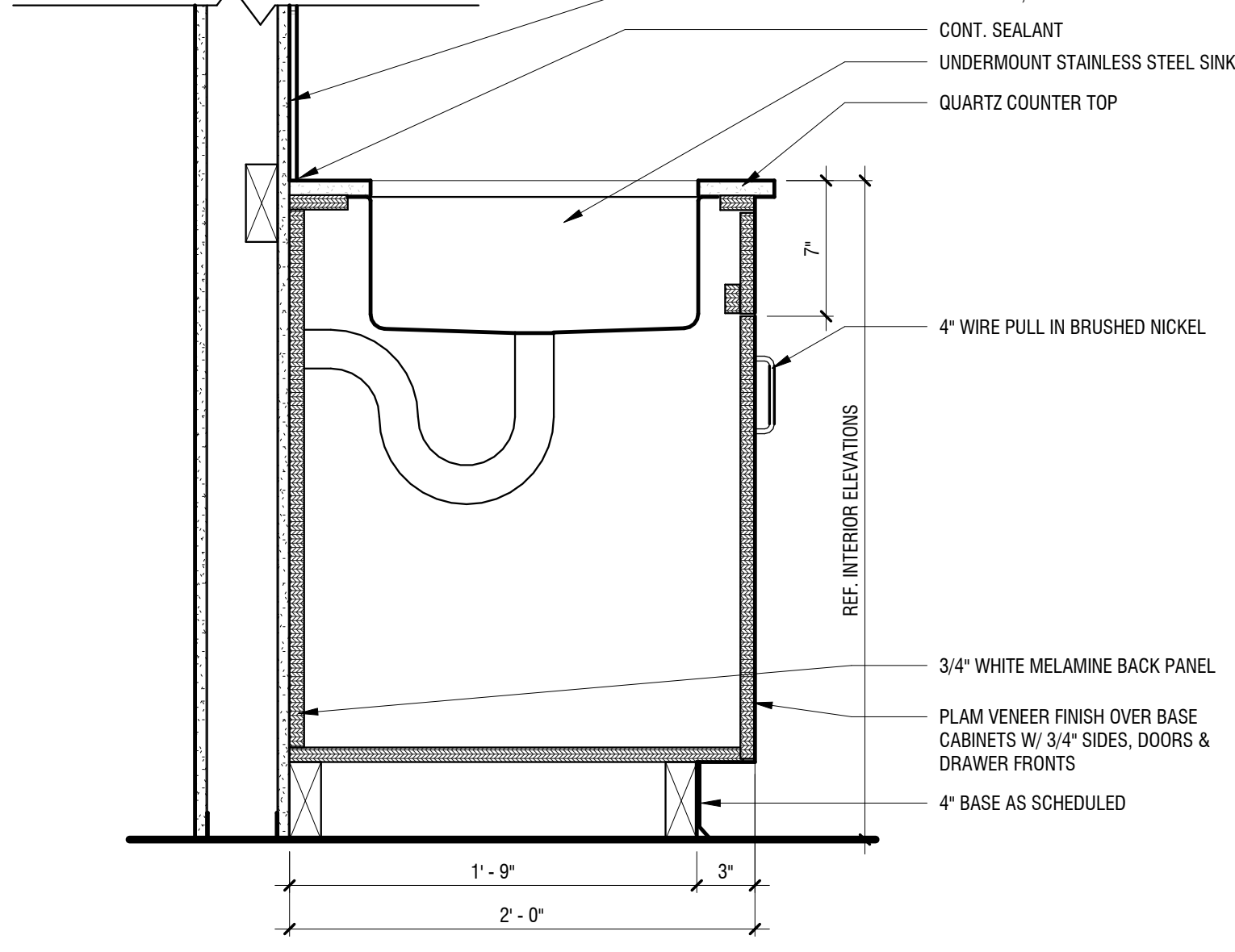
2 BASE CABINET WITH SINK A4.2 1 1/2" = 1'-0"
