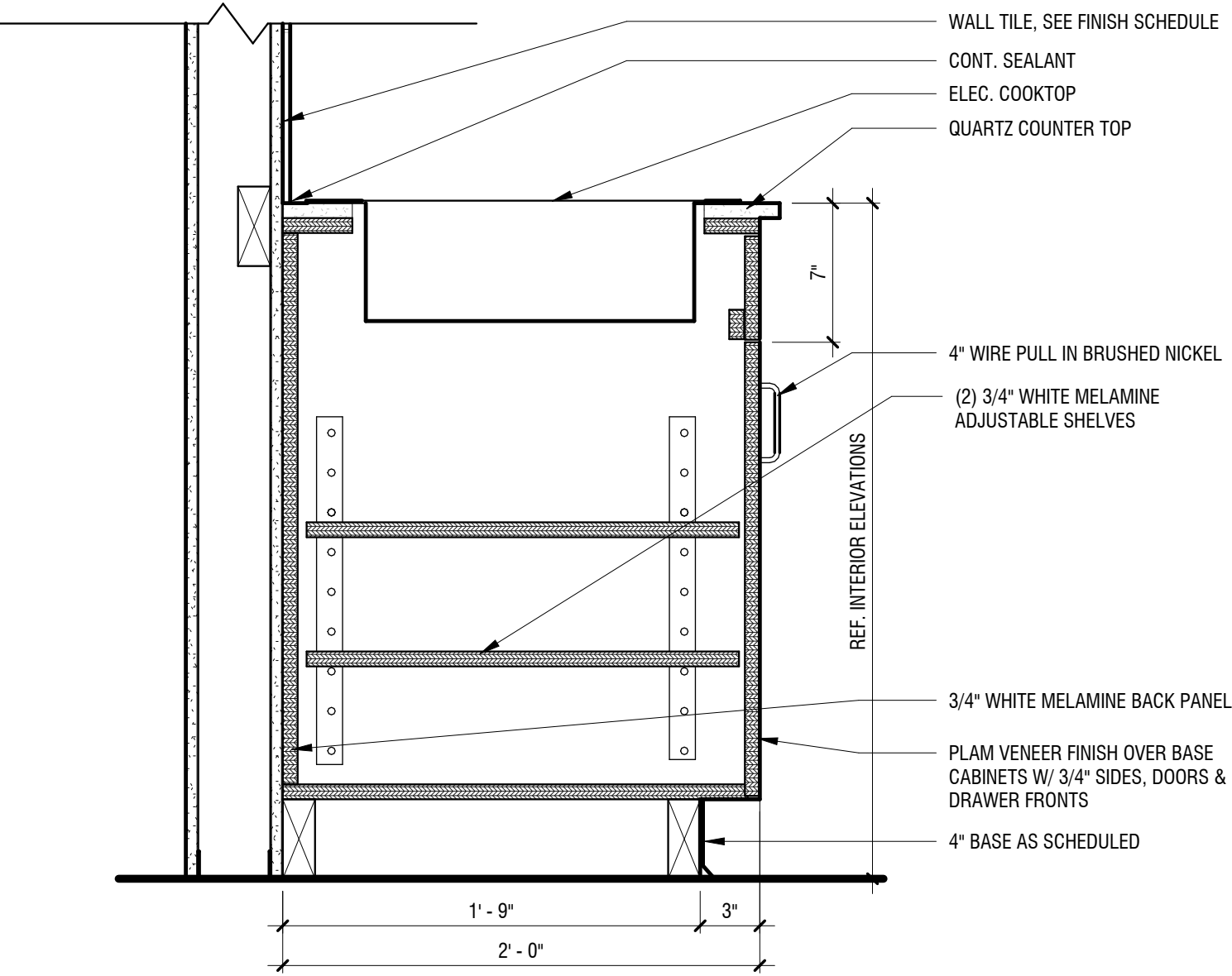
3 BASE CABINET WITH COOKTOP A4.2 1 1/2" = 1'-0"
