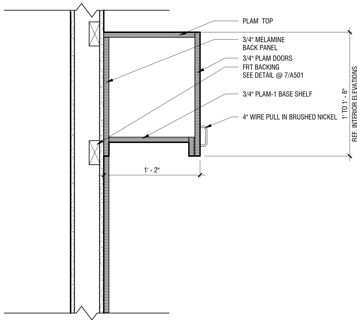
6 UPPER CABINET NO SHELVES A4.2 1 1/2" = 1'-0"
