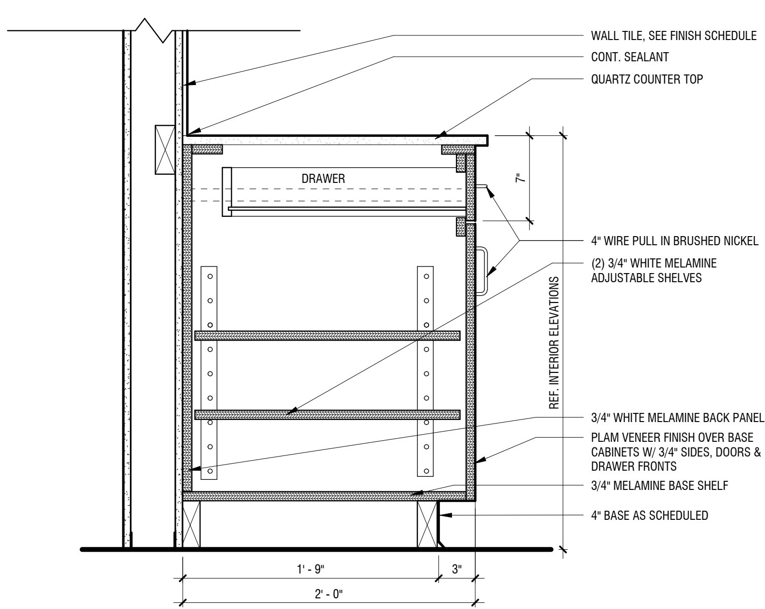
4 BASE CABINET W/ DRAWER A4.2 1 1/2" = 1'-0"
