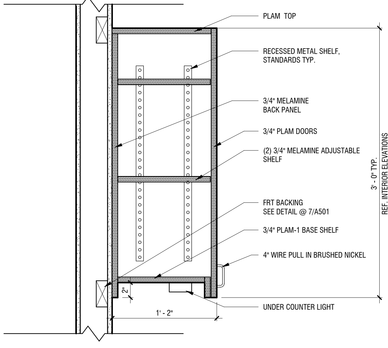
5 UPPER CABINET A4.2 1 1/2" = 1'-0"
