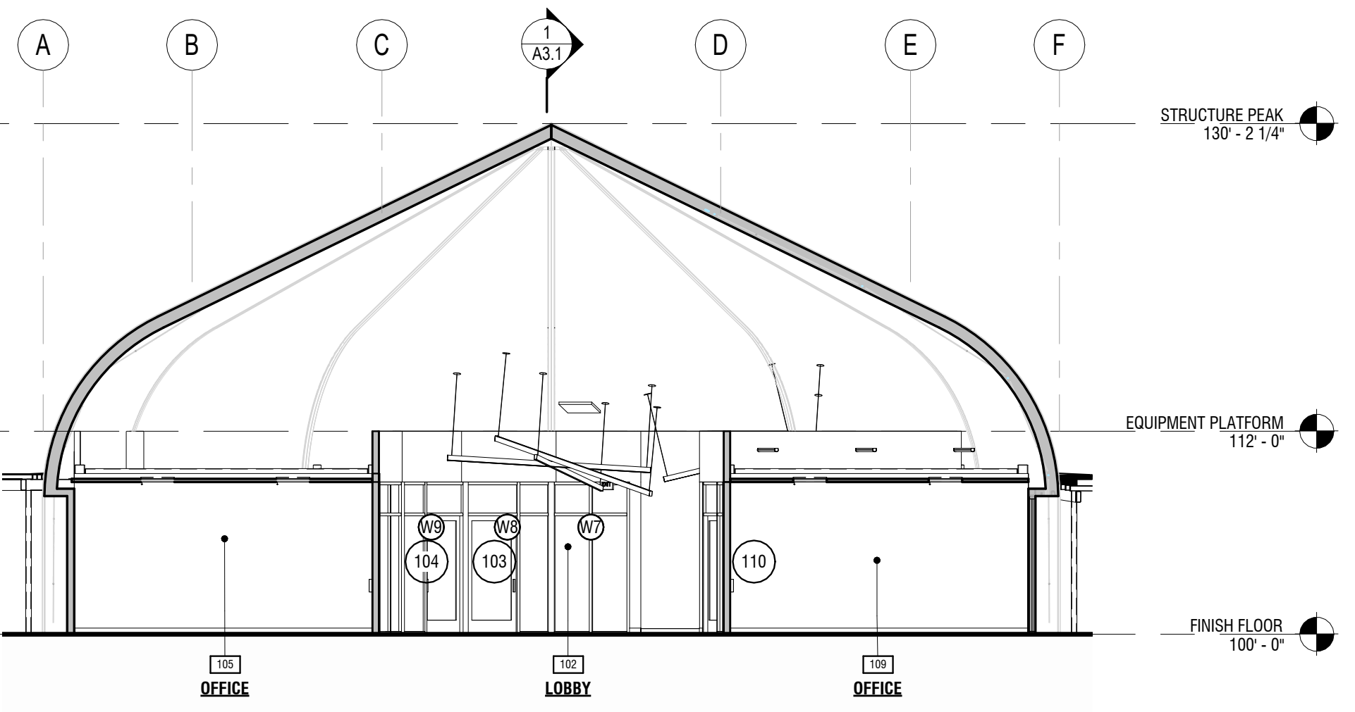
2 SECTION AT OFFICES AND LOBBY A3.1 1/8" = 1'-0"
