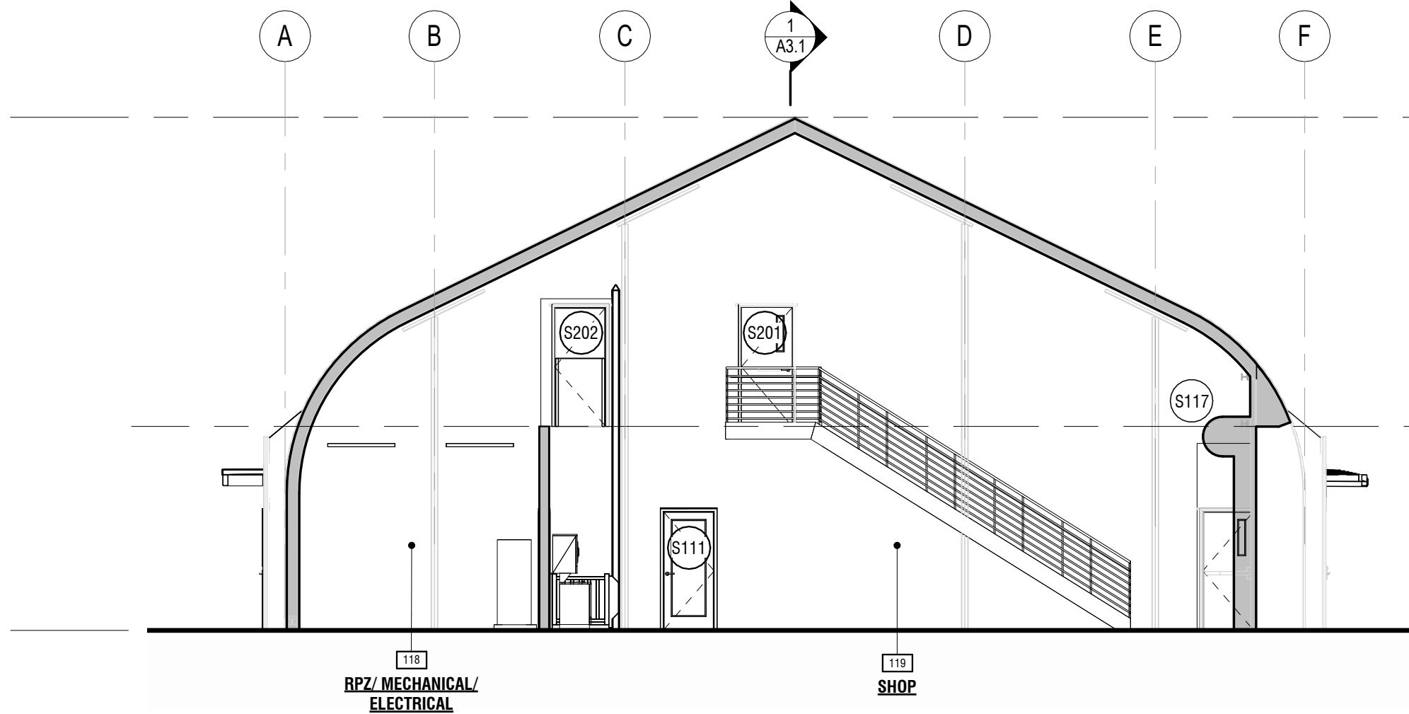
5 SECTION AT INVENTORY A3.1 1/8" = 1'-0"
