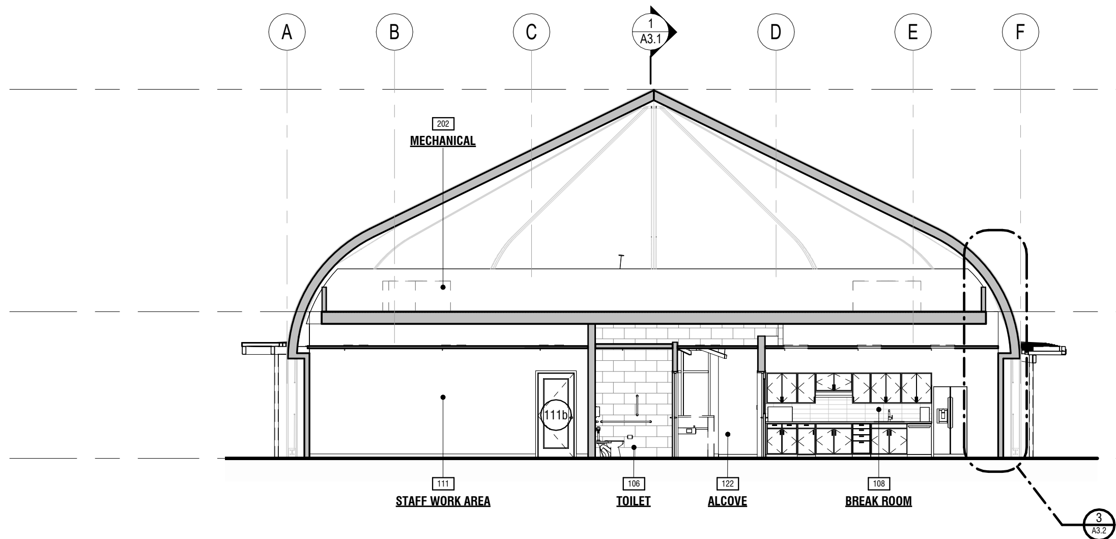
3 SECTION LOOKING EAST A3.1 1/8" = 1'-0"
