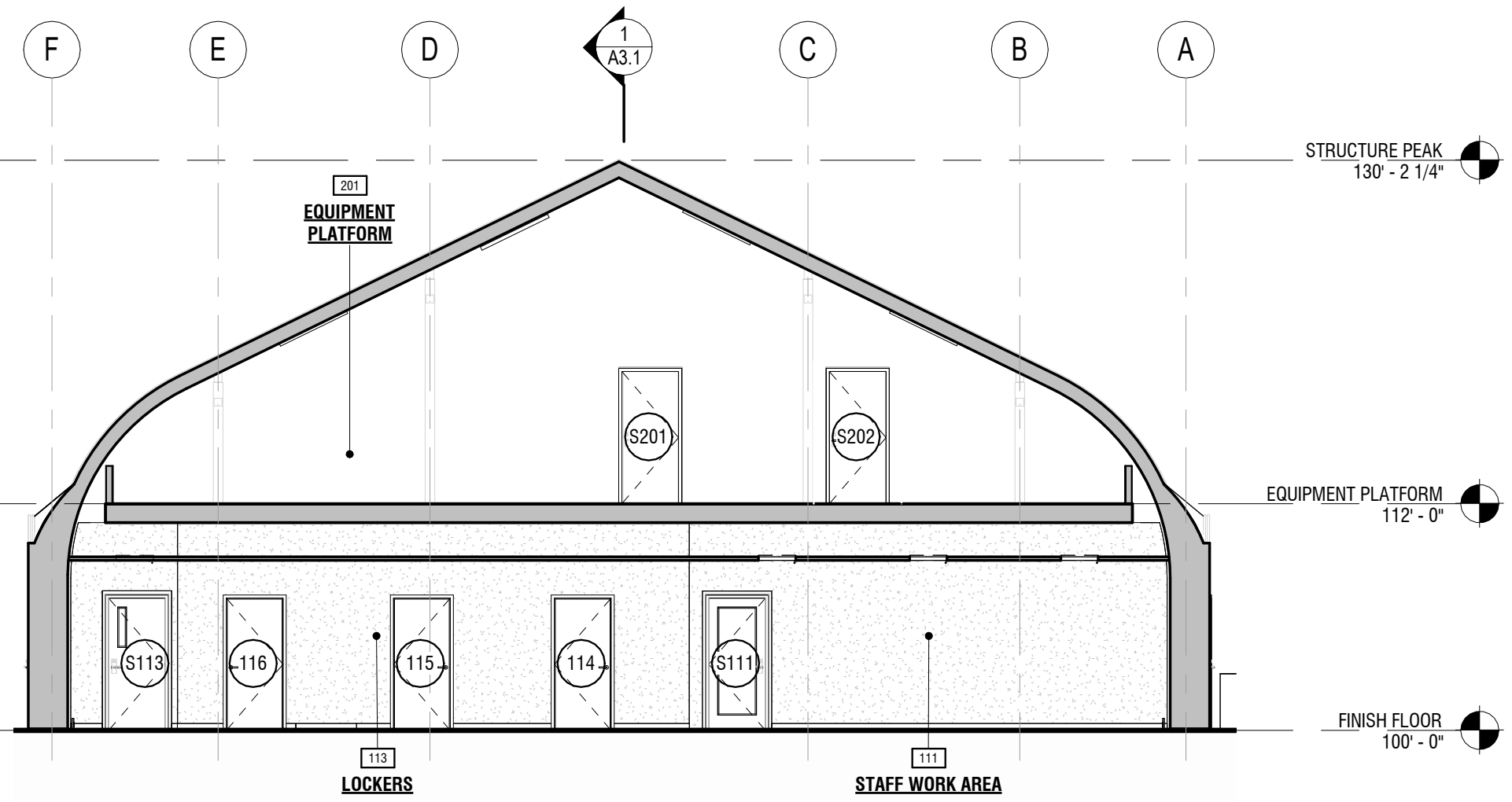
4 SECTION AT LOCKERS/EQUIPMENT PLATFORM A3.1 1/8" = 1'-0"
