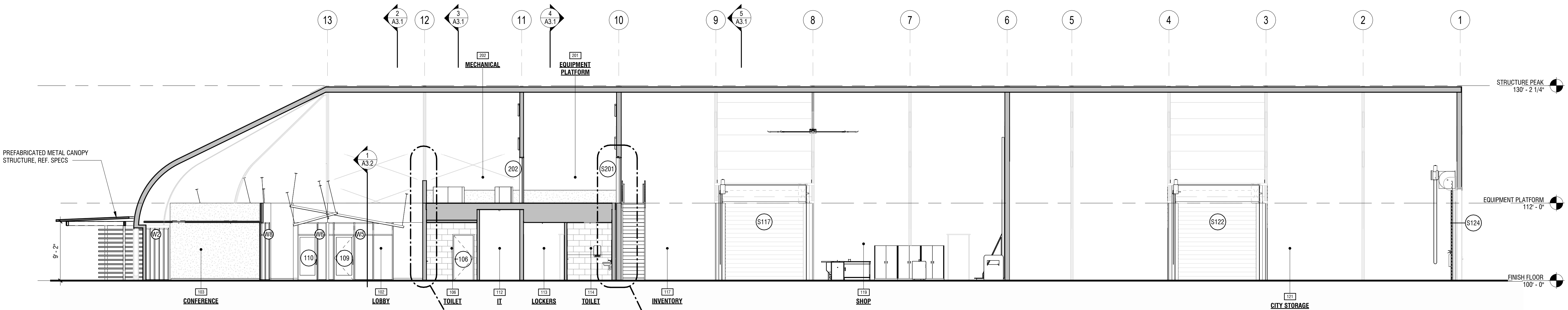
1 SECTION LOOKING NORTH A3.1 1/8" = 1'-0"
