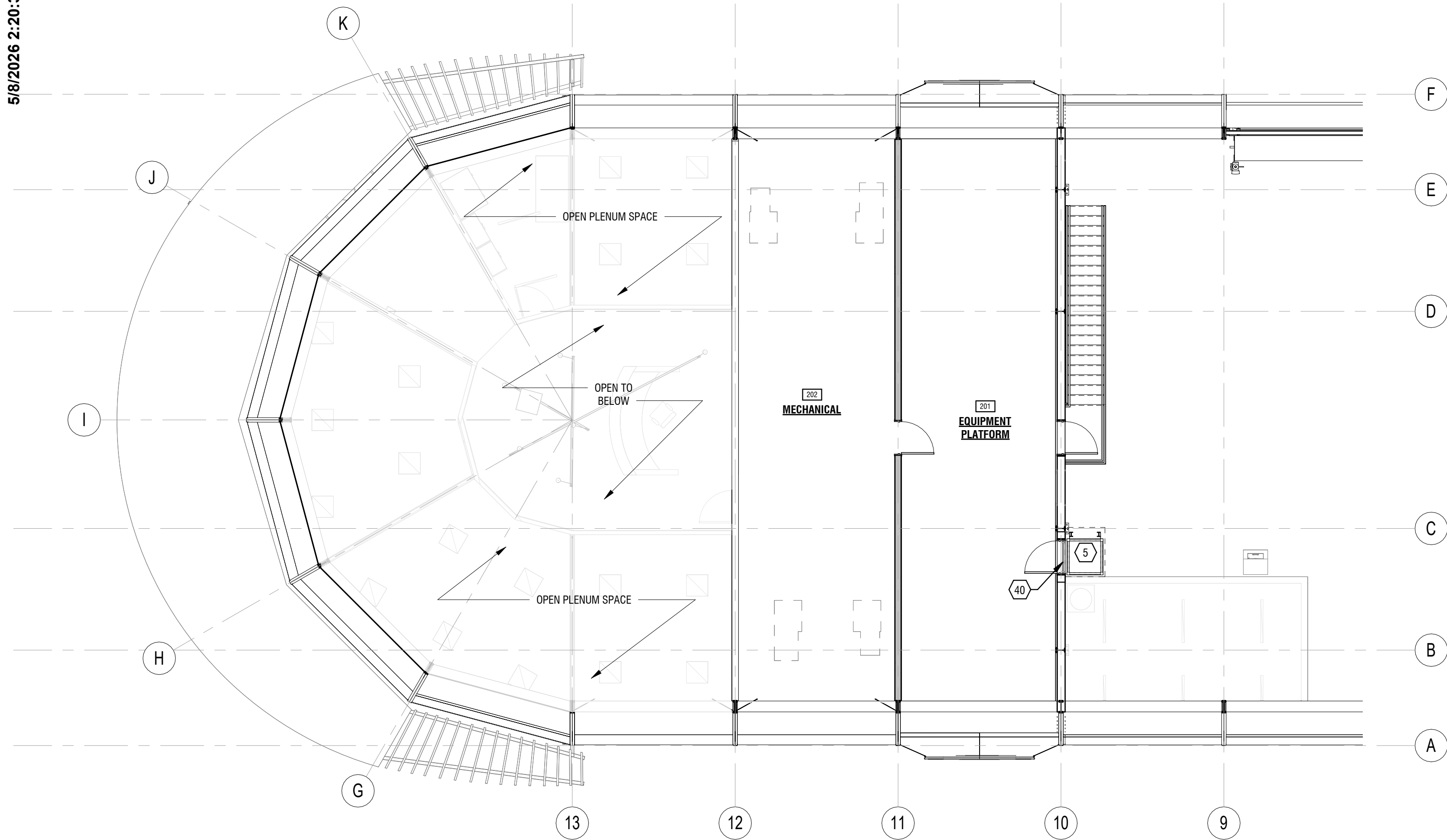
2 EQUIPMENT PLATFORM PLAN A1.4 1/8" = 1'-0"
