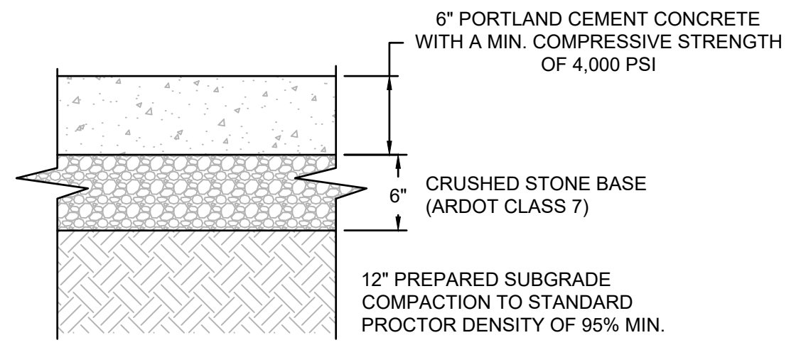
STANDARD DUTY CONCRETE PAVING DETAIL NOT TO SCALE
