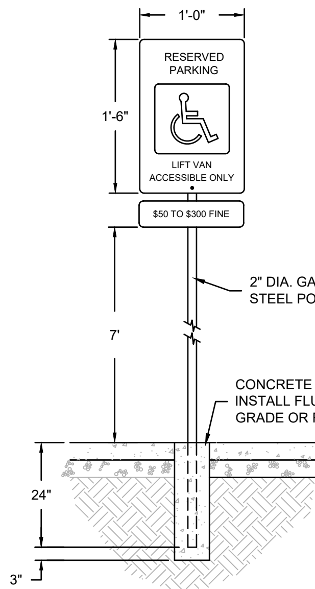
POLE MOUNTED LIFT VAN ACCESSIBLE SIGN
