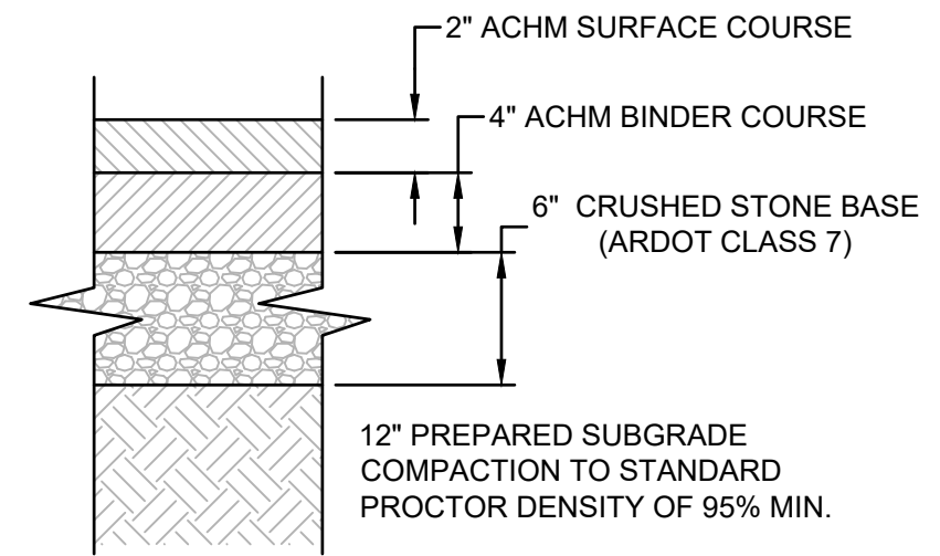
HEAVY DUTY ASPHALT PAVEMENT SECTION NOT TO SCALE
