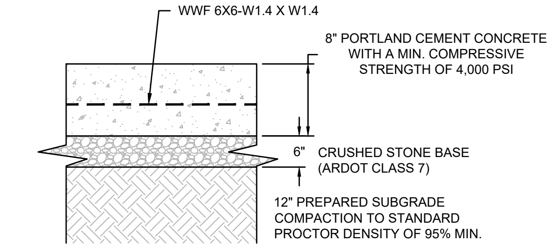
HEAVY DUTY CONCRETE PAVING DETAIL NOT TO SCALE
