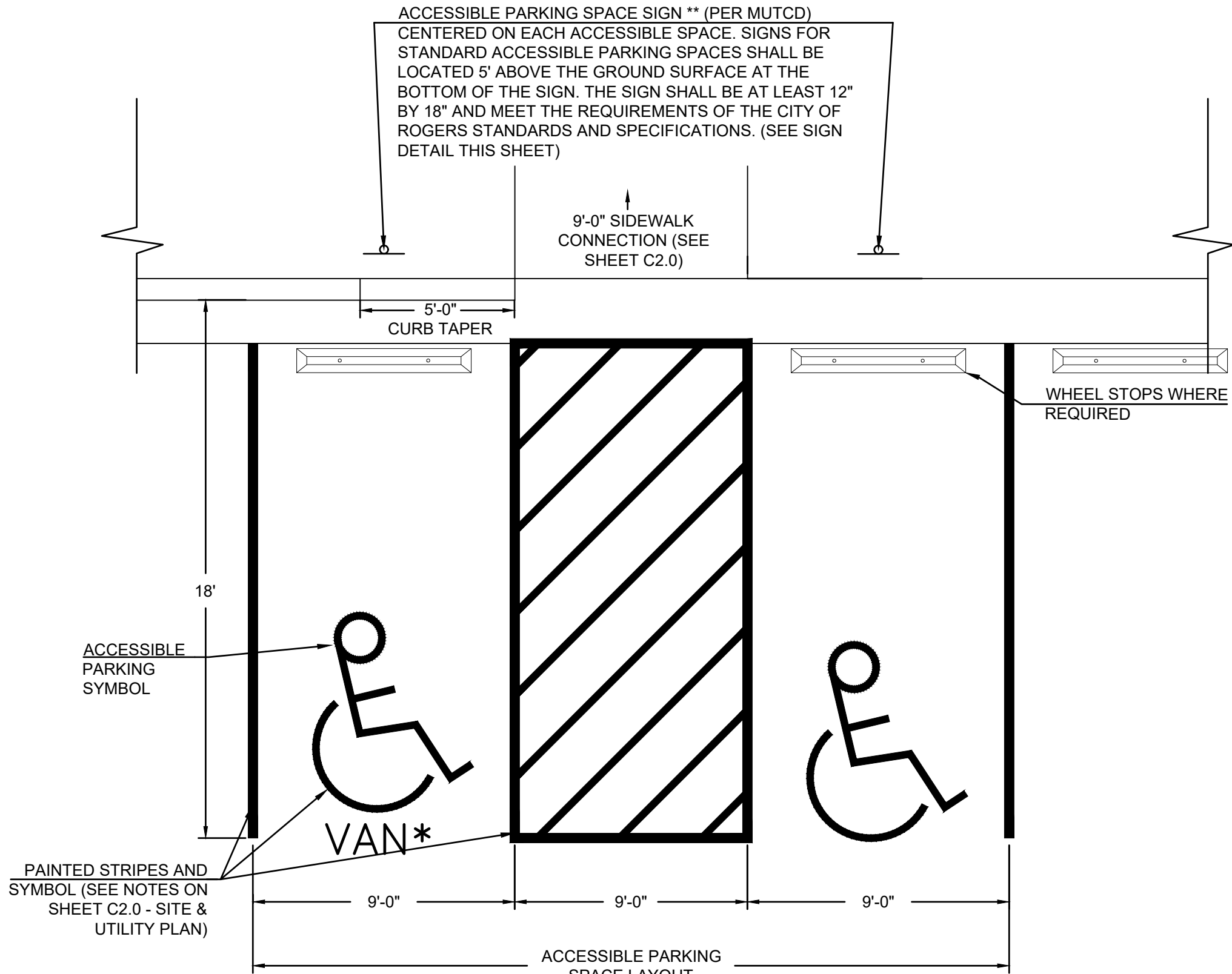
ACCESSIBLE PARKING SPACE LAYOUT DETAIL (TYP.) NOT TO SCALE
