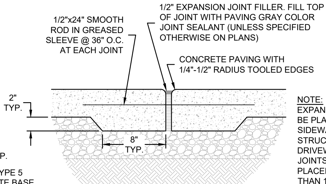
EXPANSION & CONSTRUCTION JOINT DETAIL
