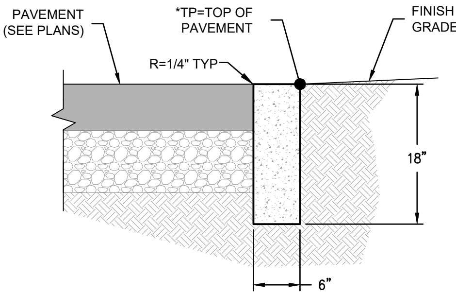
FLUSH RIBBON CURB (PRIVATE ONLY) DETAIL NOT TO SCALE
