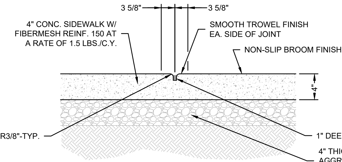
SIDEWALK & TOOLED CONTROL JOINT DETAIL
