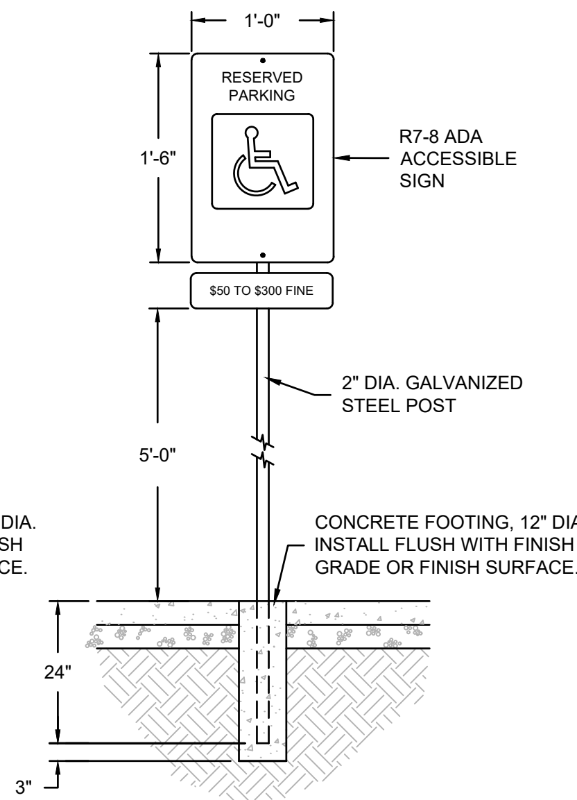
POLE MOUNTED ACCESSIBLE SIGN NOT TO SCALE
