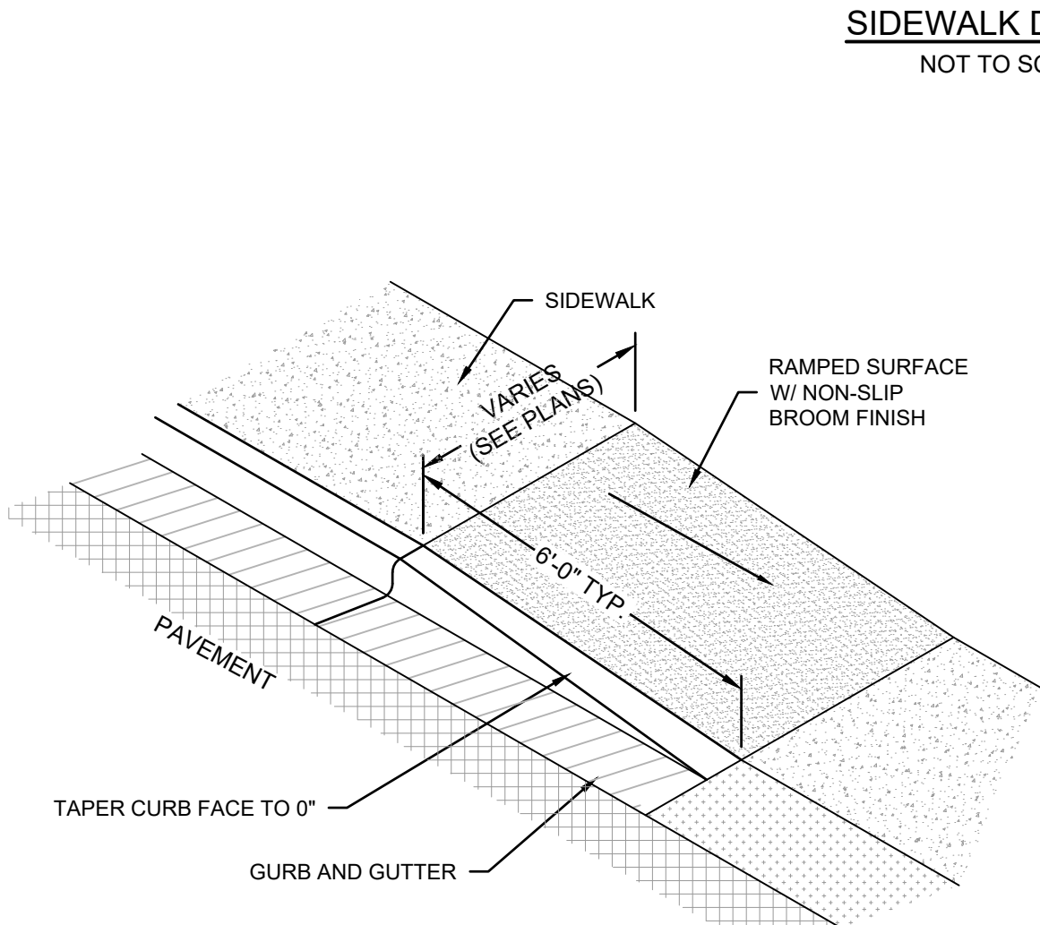
CURB & SIDEWALK TRANSITION TO PAVEMENT DETAIL NOT TO SCALE
