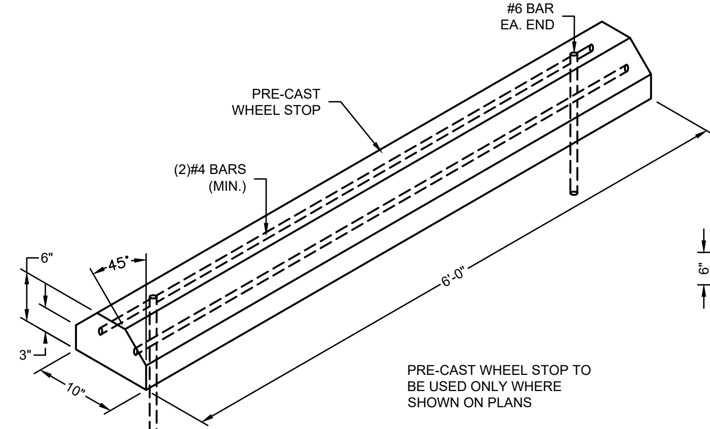
PRE-CAST WHEEL STOP DETAILS NOT TO SCALE
