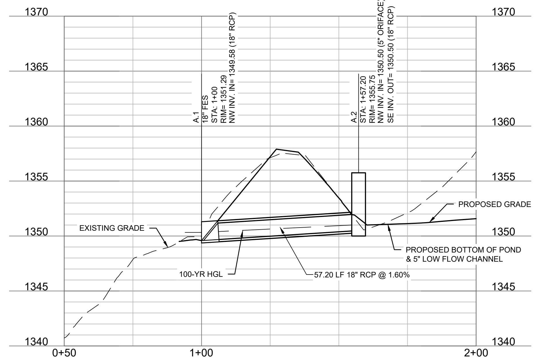
STORM LINE A (0+50 - 2+00)
